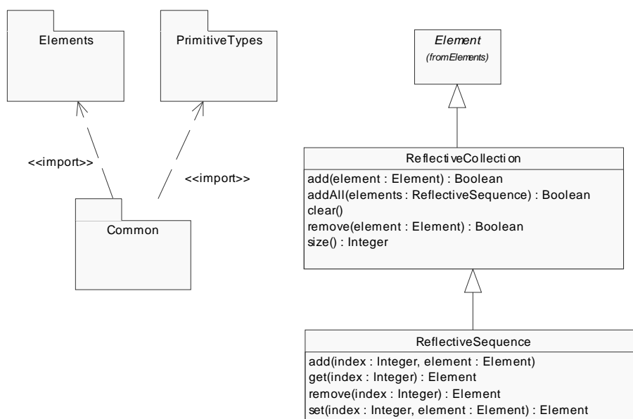
Figure 5-4. The Common package.
