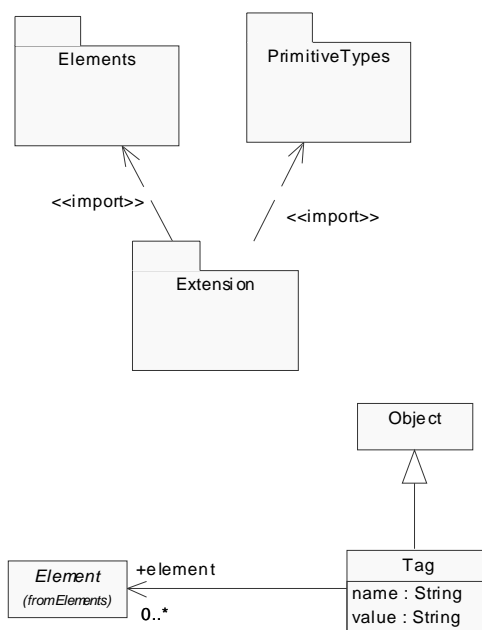
Figure 6-5. The Identities package.
