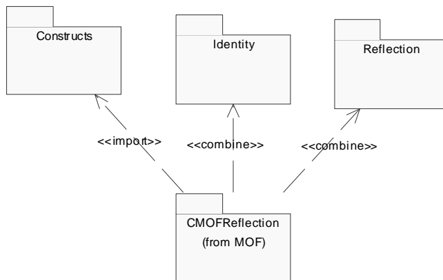
Figure 8-7. CMOF Reflection package.
