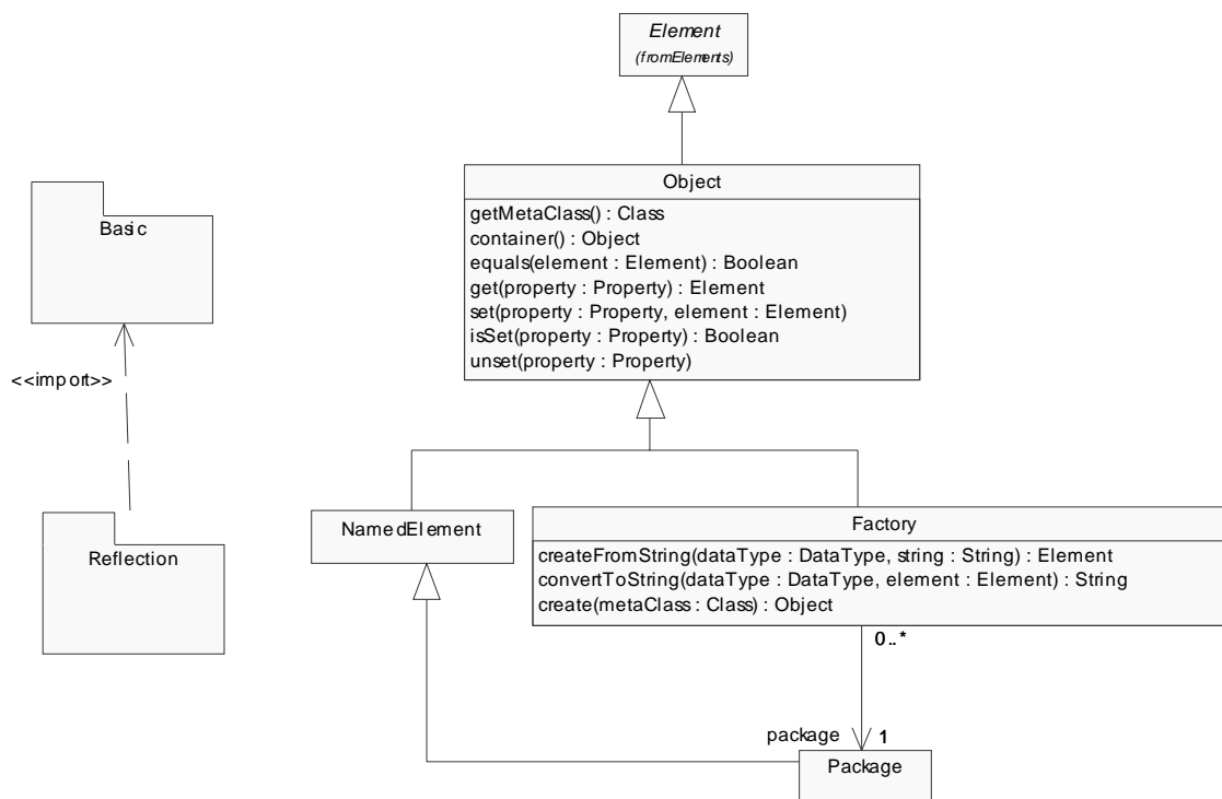
Figure 4-2. The Reflection package.
