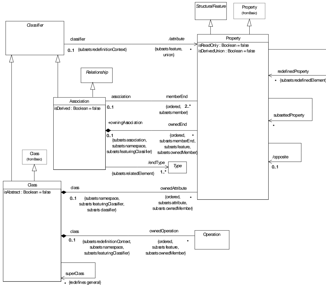
Figure 9-12. Key concrete classes from the UML Core::Constructs
