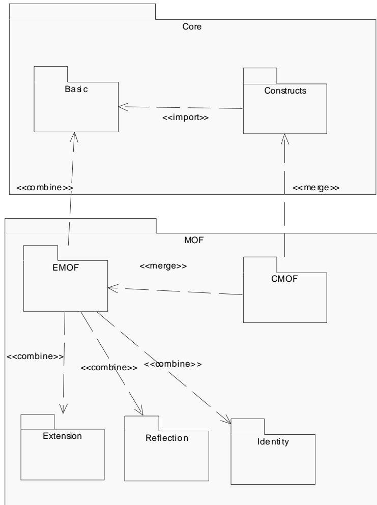
Figure 1-1. MOF imports from the UML Core
