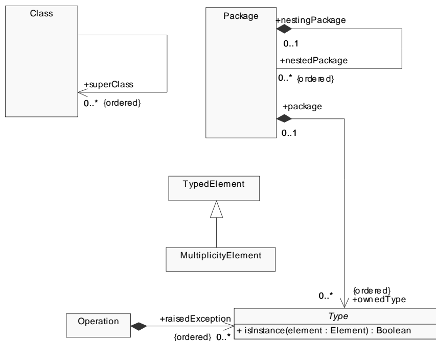
Figure 7-2. EMOF Extensions
