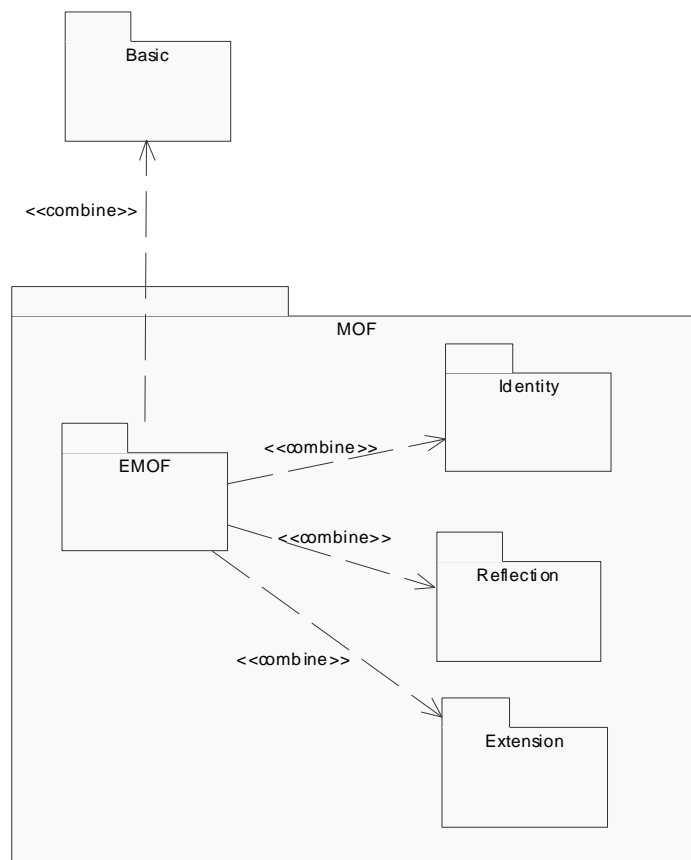
Figure 7-1. EMOF Model- Overview
