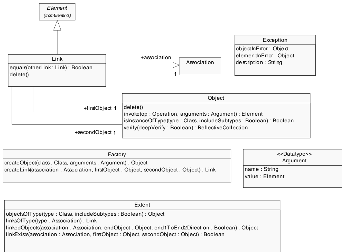
Figure 8-8. CMOF Extensions to Reflection
