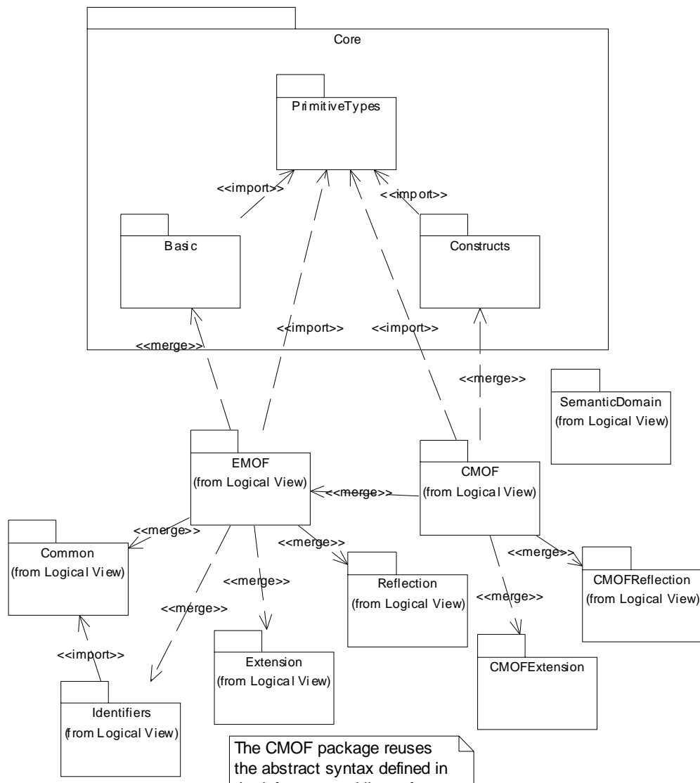
Figure 14.1 - CMOF Packages
