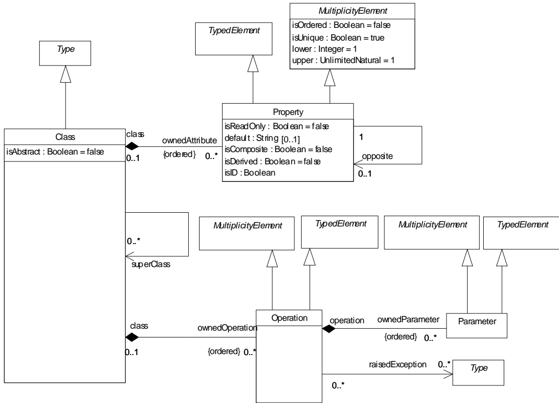
Figure 12.2 - EMOF Classes
