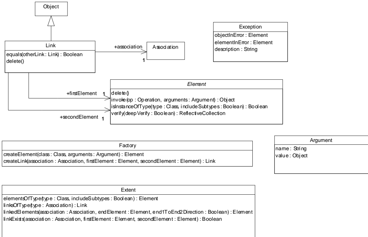
Figure 13.2 - CMOF Reflection package
