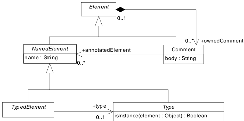
Figure 12.5 - EMOF Types
