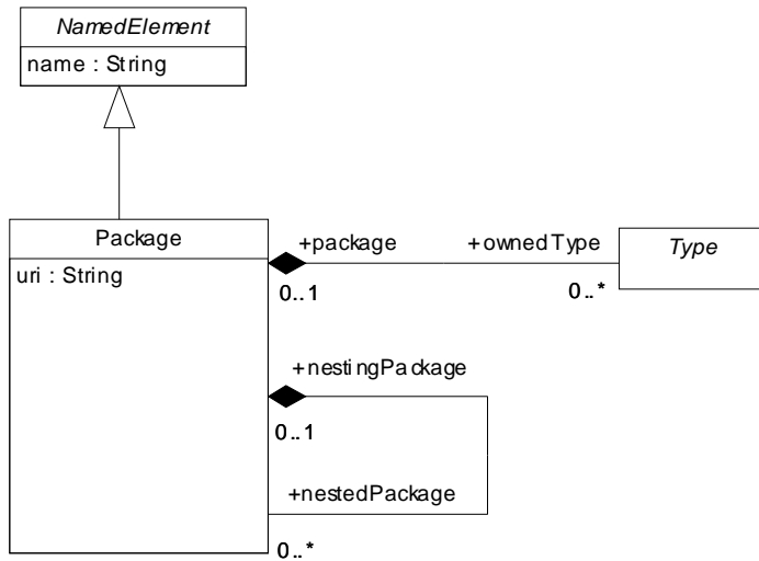
Figure 12.4 - EMOF Packages
