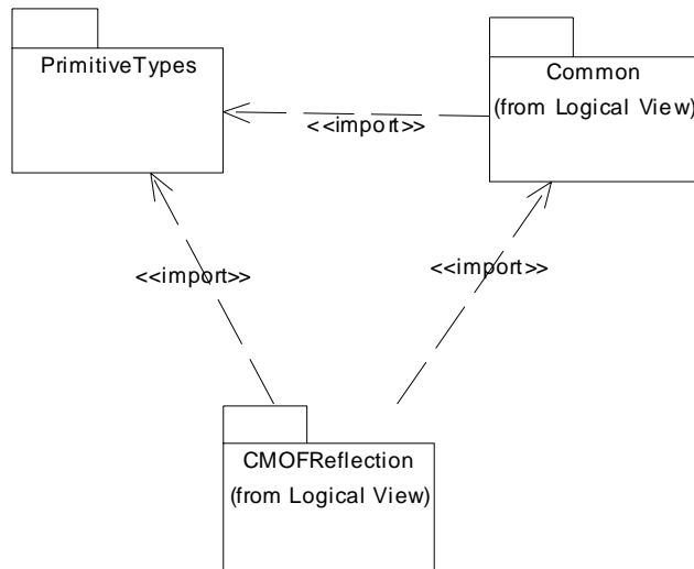
Figure 13.1 - CMOF Reflection
