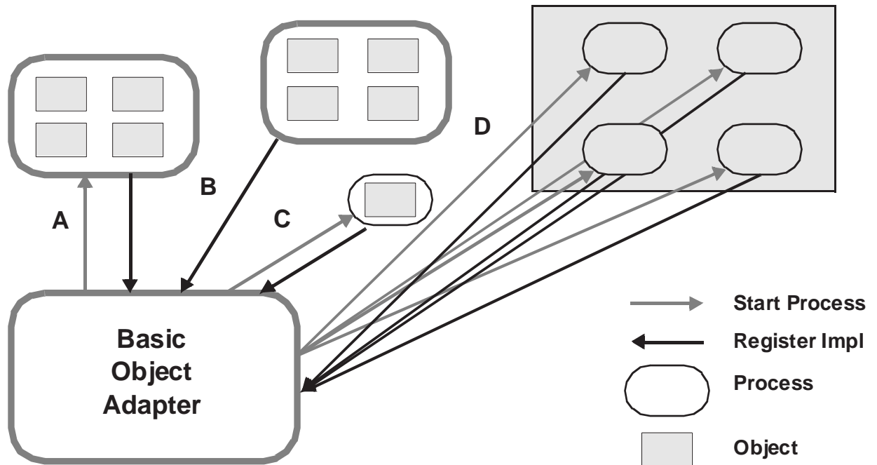
Figure 8-2 Implementation Activation Policies
