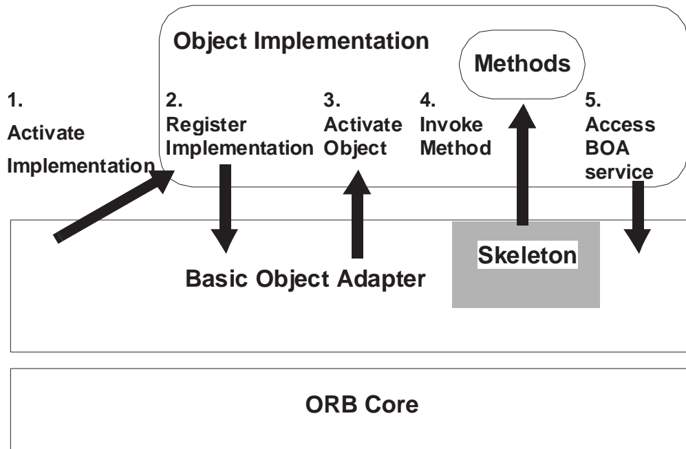
Figure 8-1 The Structure and Operation of the Basic Object Adapter
