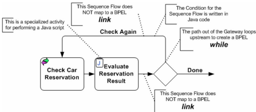
Figure 5: A Loop within the Process
