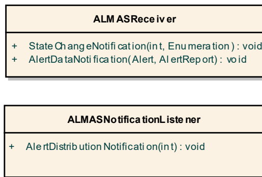
Figure 6.1.1 : PIM class diagram for ALMAS Clients
