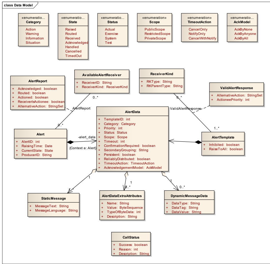
Figure 6.2.2: PIM class diagram for ALMAS Data Model
