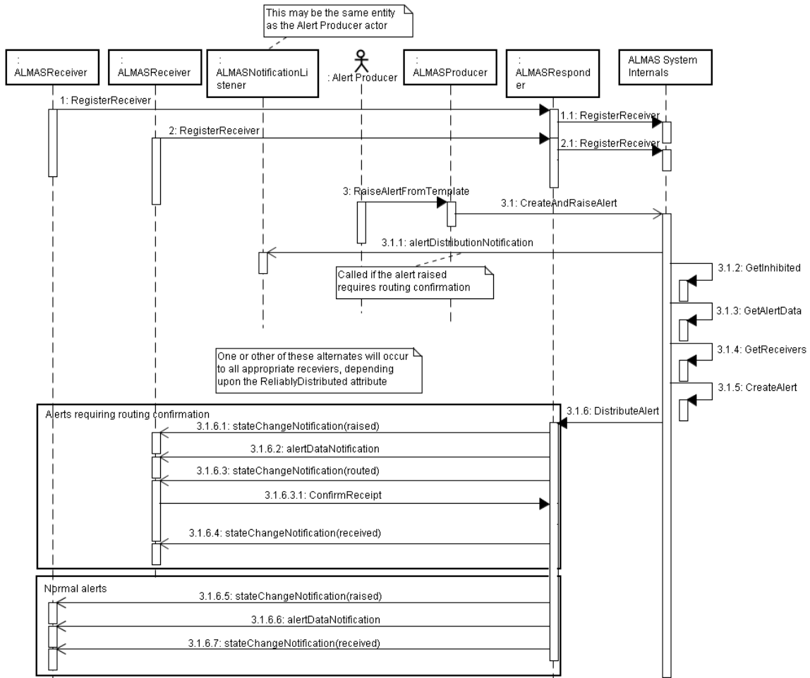
Figure 6-7-7: Alert Registration and Creation Sequence Diagram
