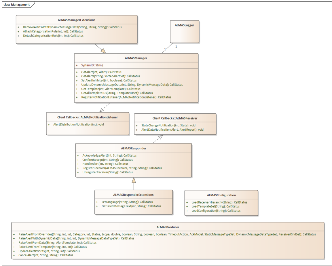
Figure 6.3-3: PIM class diagram for ALMAS Management
