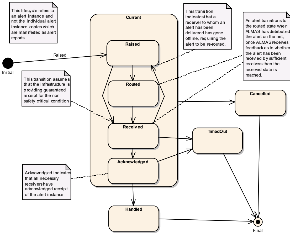
Figure 6-5-5: Action/Situation Alert Lifecycle
