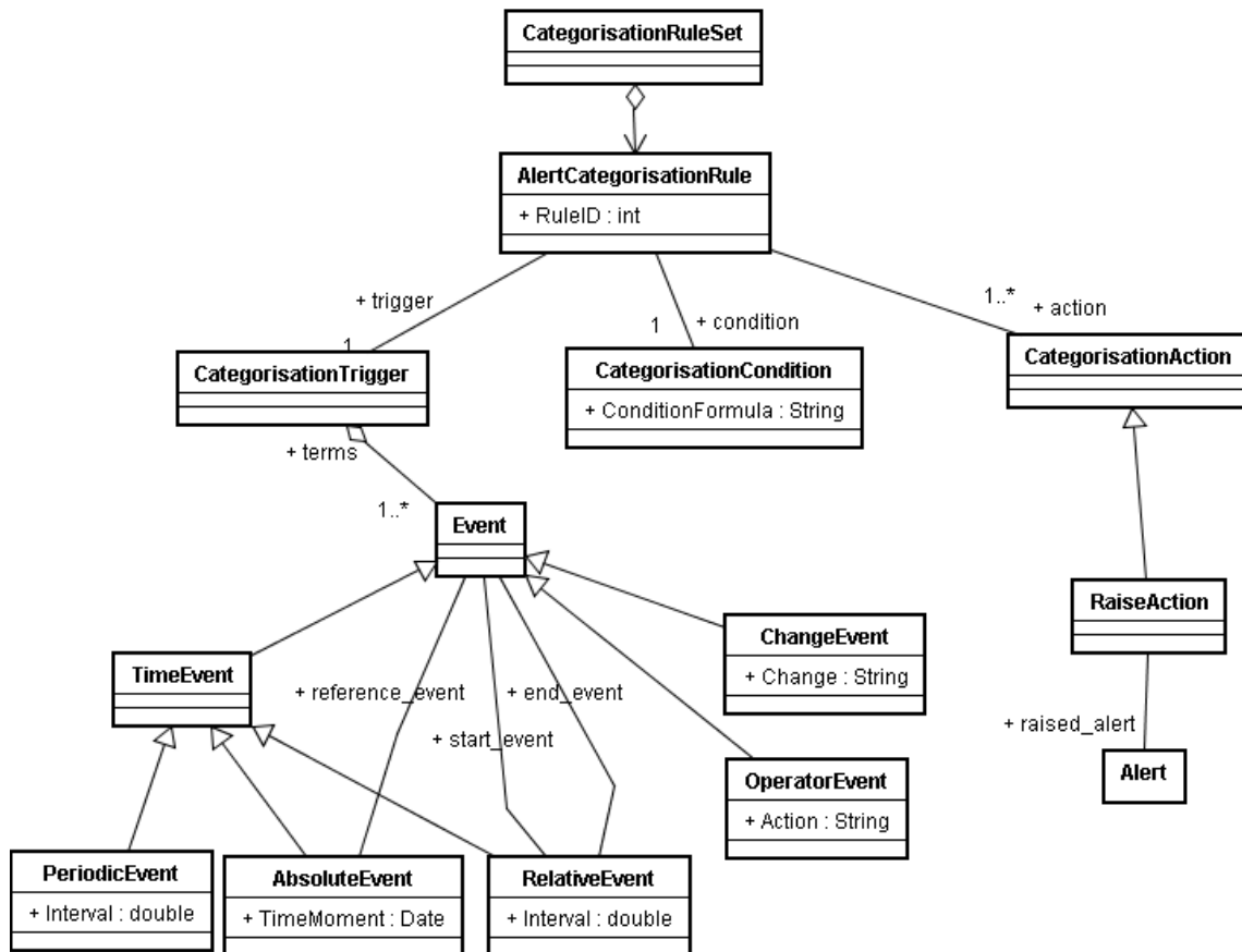
Figure 6.4.4: Alert Categorisation Platform Independent Model
