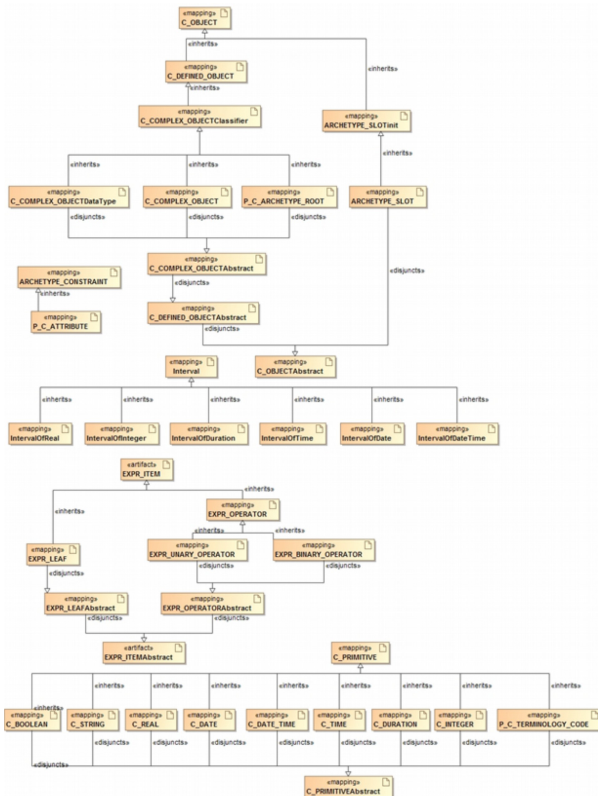
Figure 7. AML Transformation Disjunction and Inheritance
