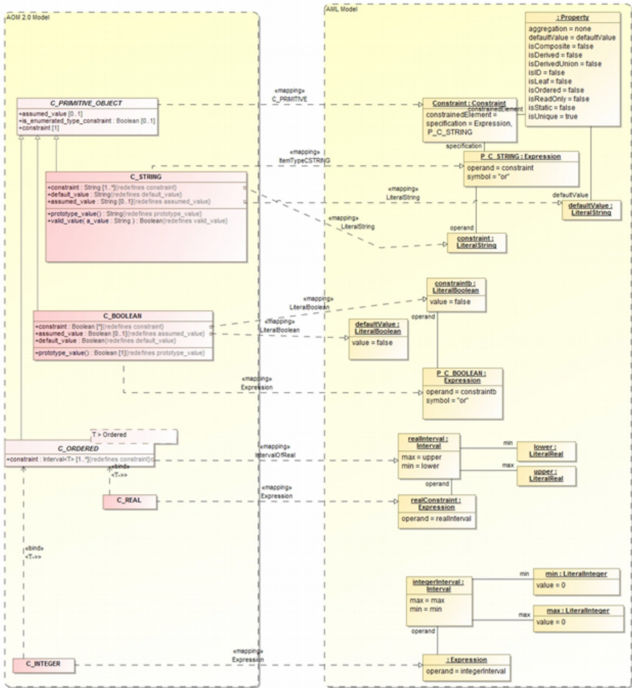
Figure 16. Primitive Constraints
