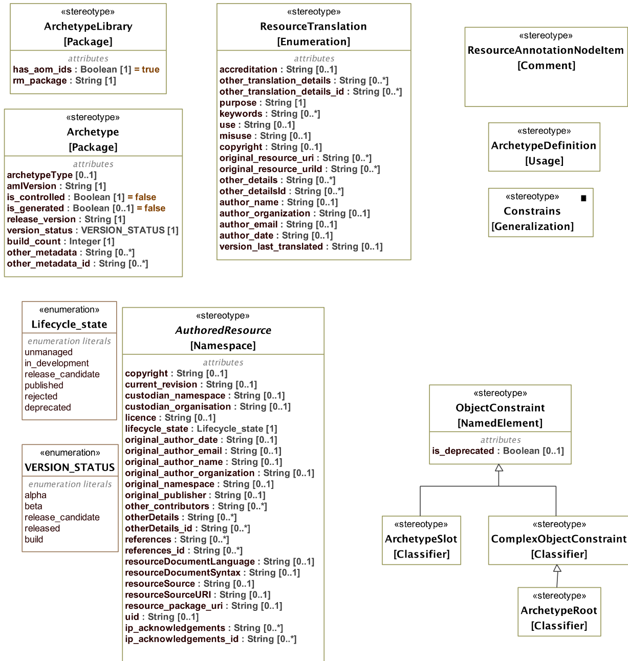
Figure 4. Constraint Profile
