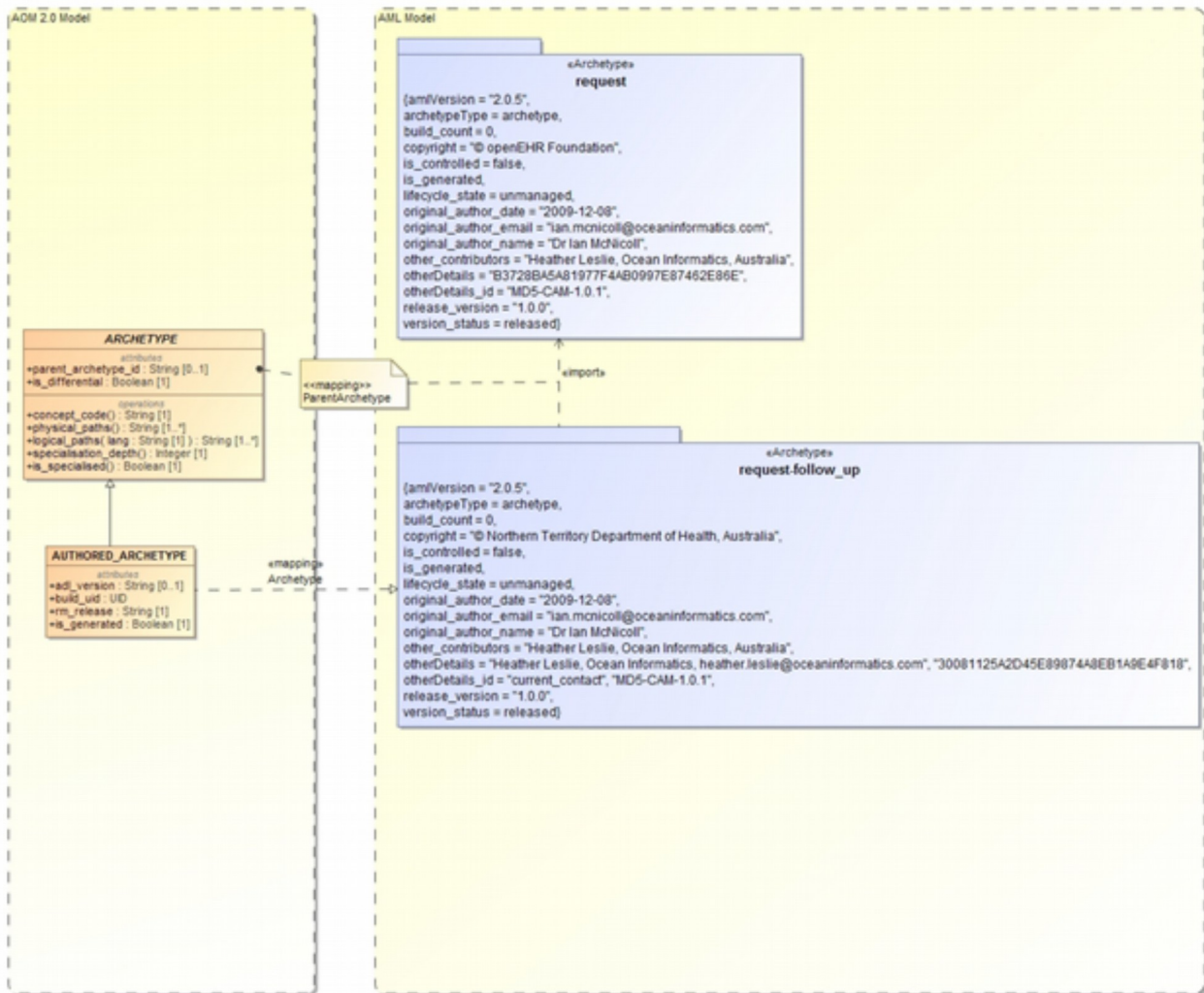
Figure 8. AML Transformation Mapping Notation Overview
