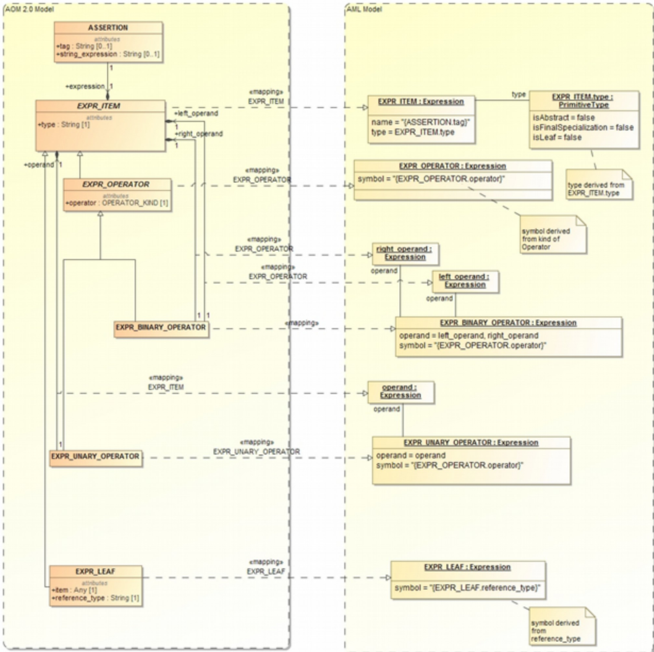
Figure 19. Assertions Mapping Overview
