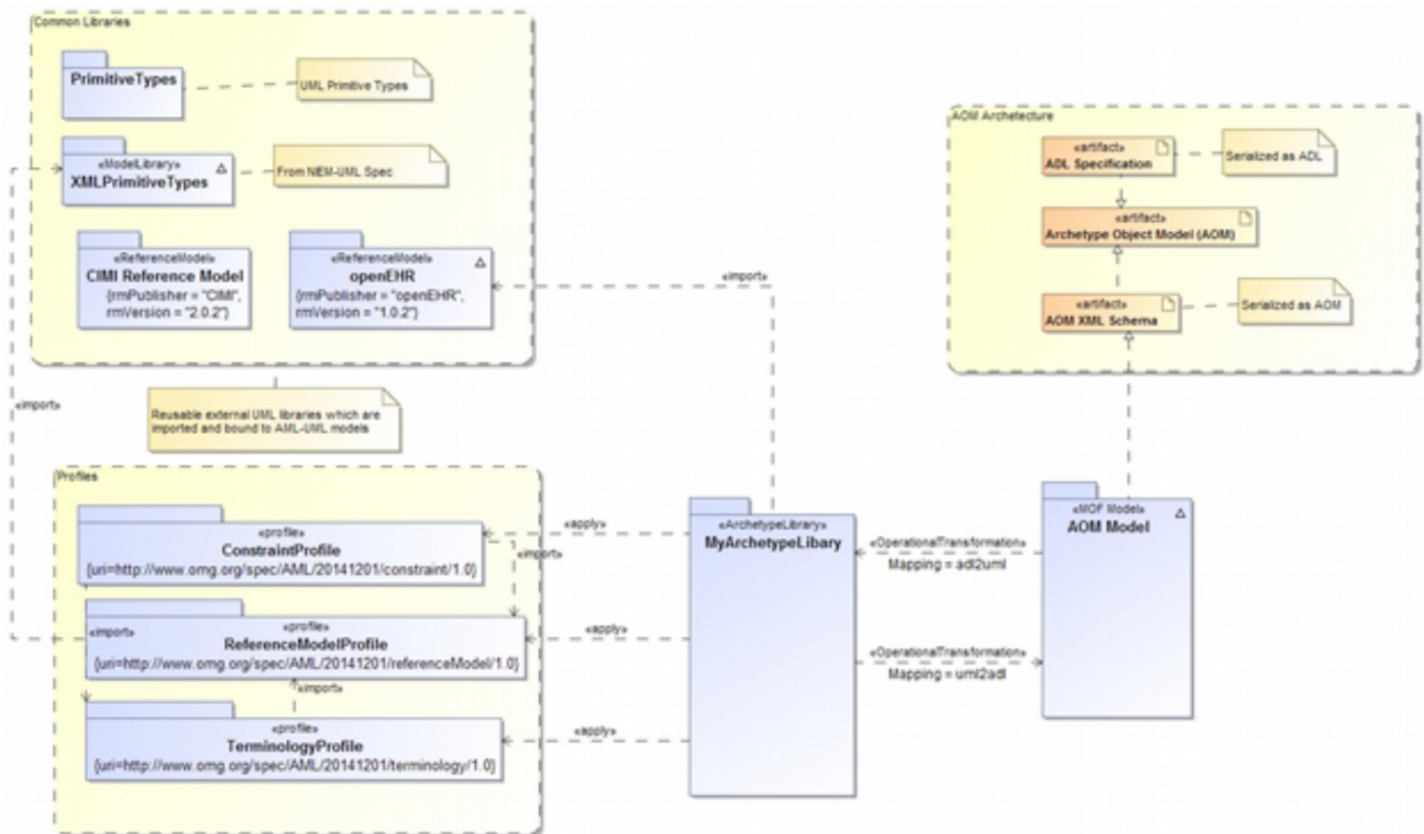
Figure 5. AML Provisioning Context
