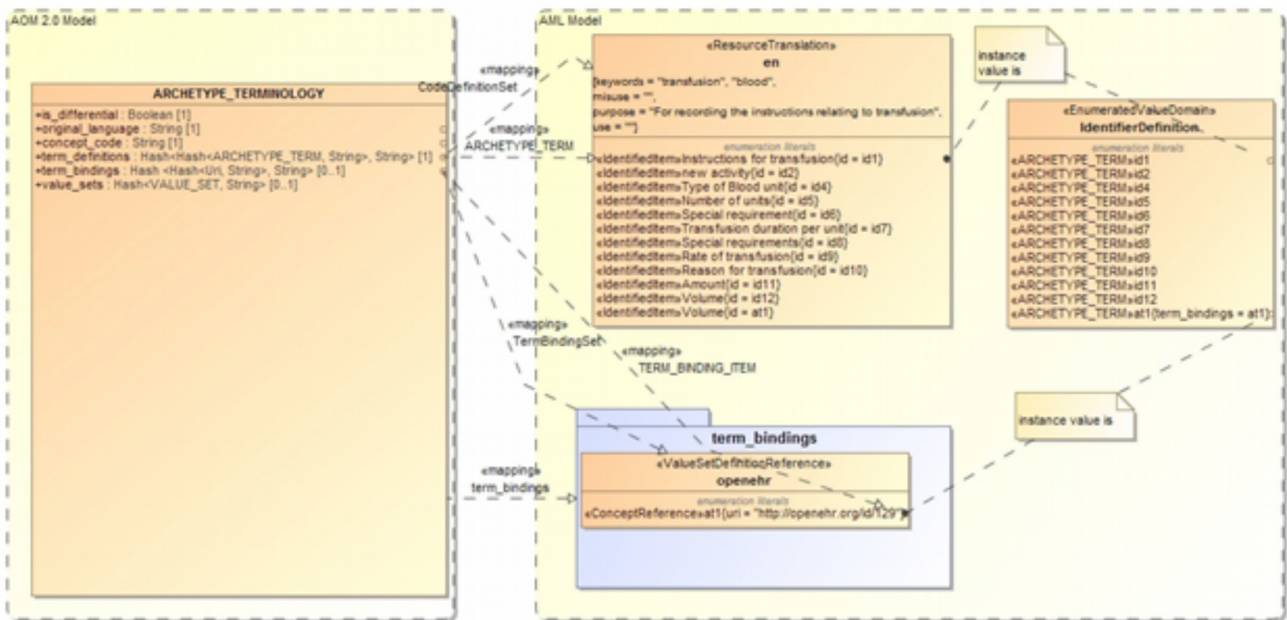
Figure 12. Terminology Binding Mapping Overview
