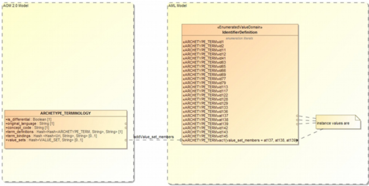
Figure 13. Local Value-sets
