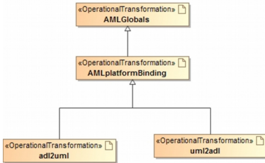
Figure 6. AML Transformations
