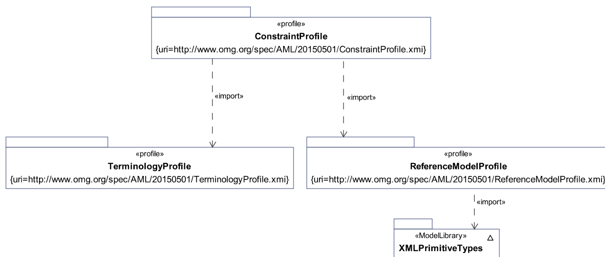
Figure 1. AML Dependencies
