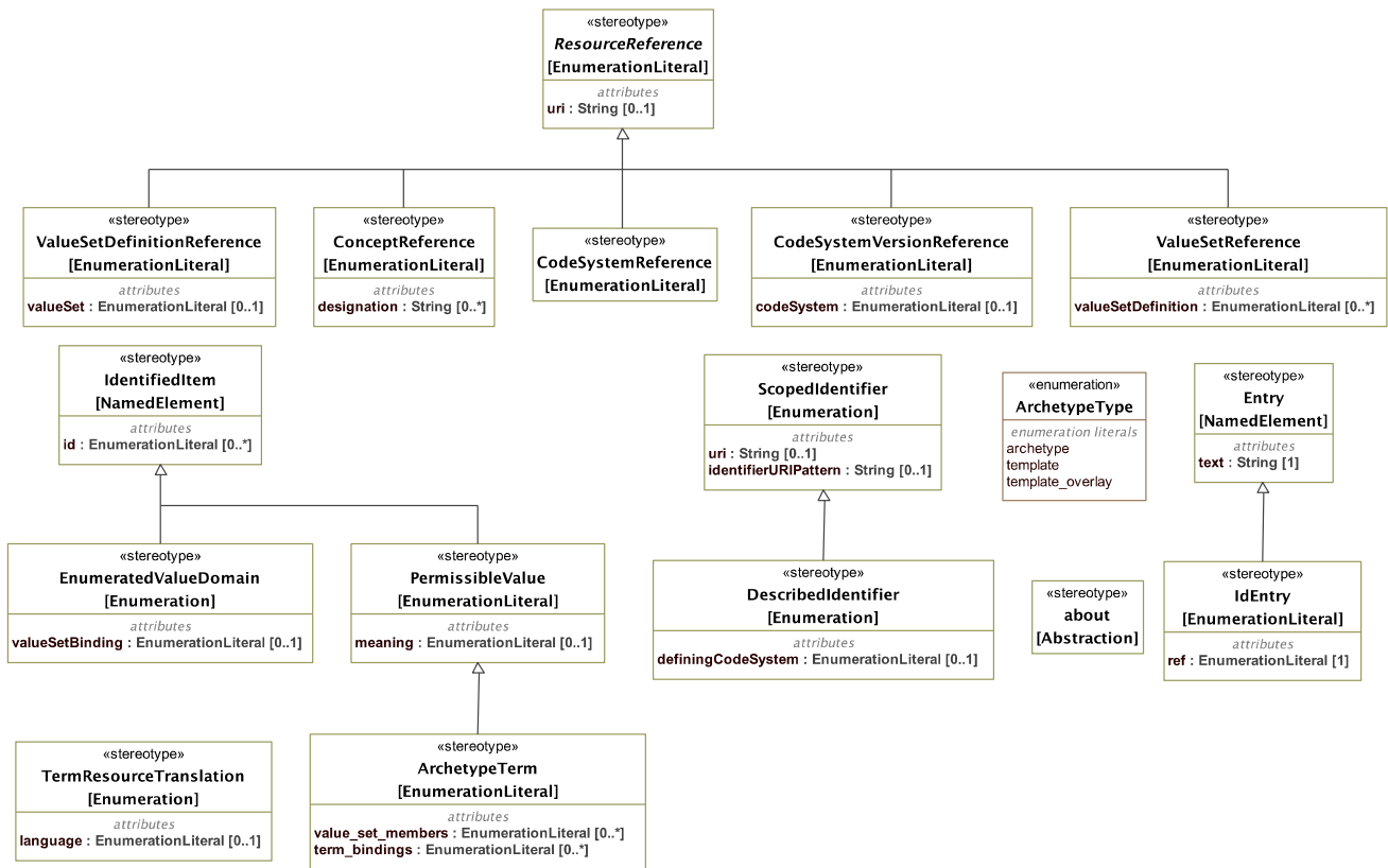
Figure 3. Terminology Binding Profile
