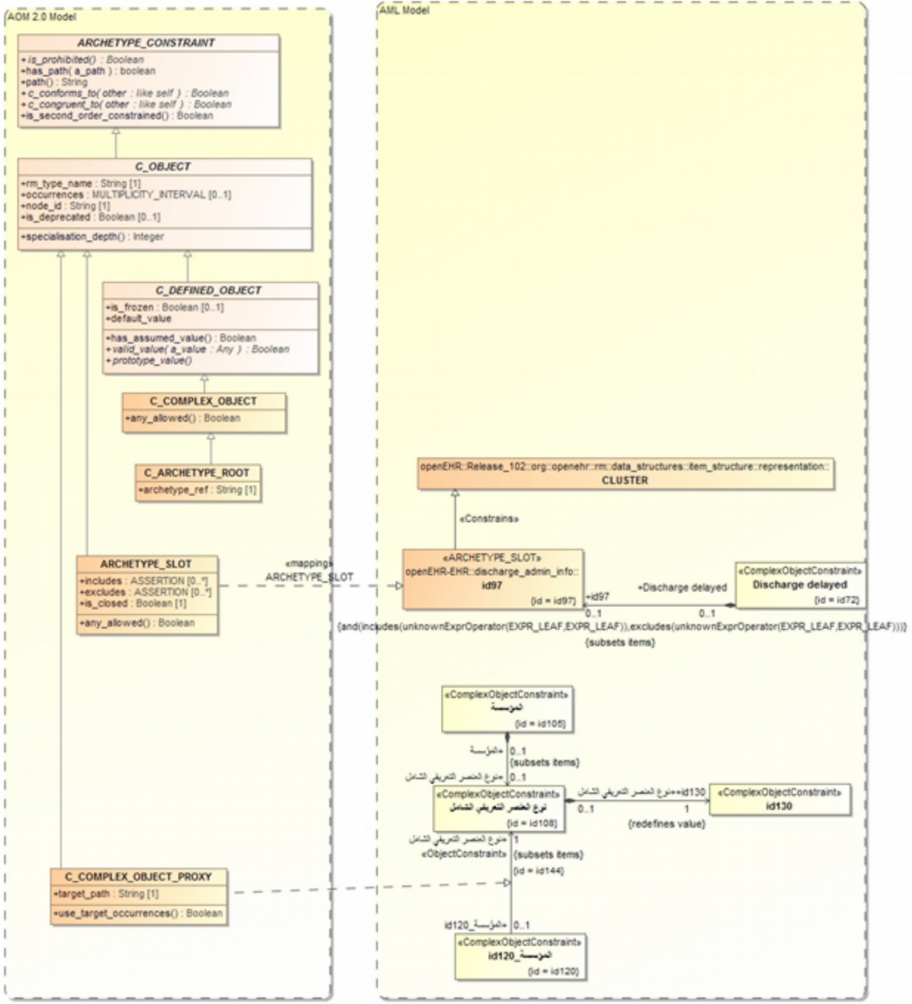
Figure 15. Object Reference Mapping
