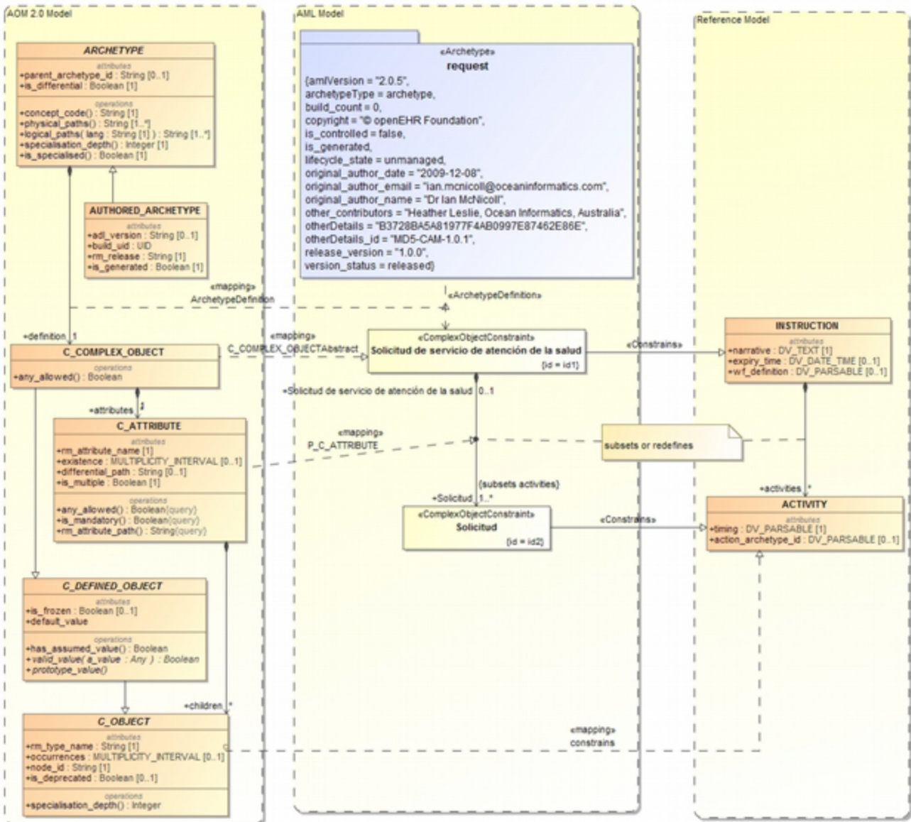
Figure 14. Archetype Definition Mapping Overview
