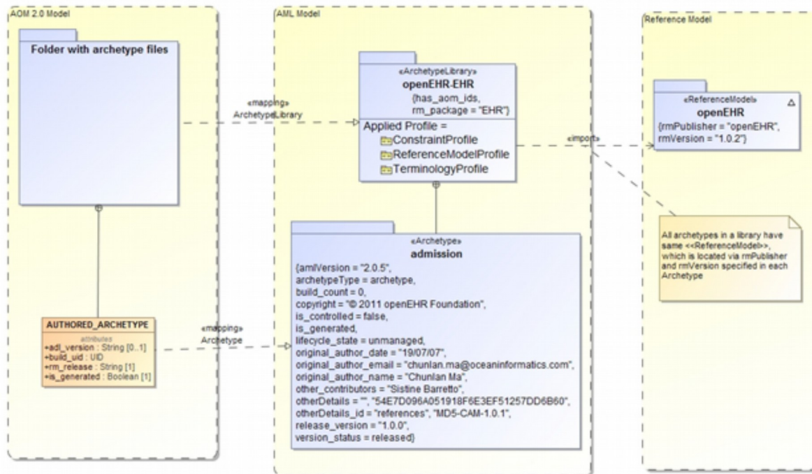
Figure 9. <<Archetype Library>> Mapping Overview
