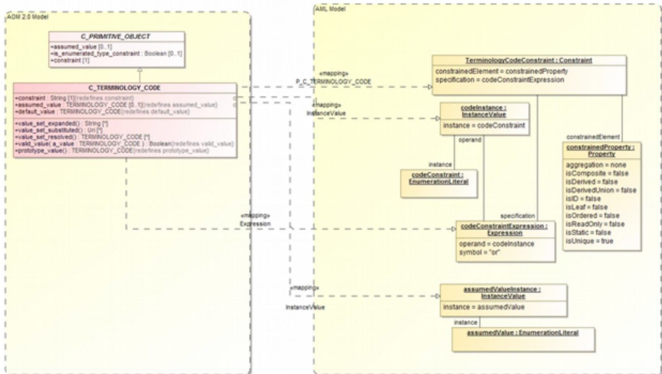
Figure 18. Code Constraint Mapping Overview
