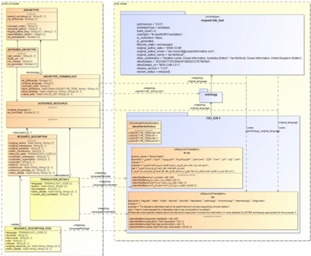
Figure 11. Terminology Definition Mapping Overview
