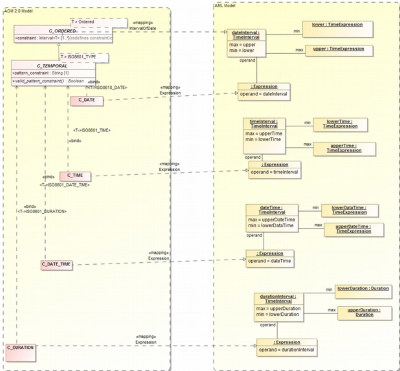
Figure 17. Temporal Constraints Mapping Overview
