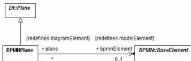
Figure 12.2 – BPMN Plane
