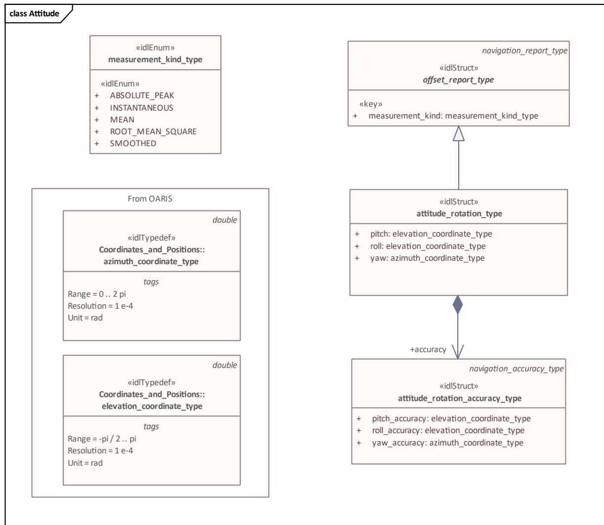
Figure 7.3 Attitude (Logical diagram)
