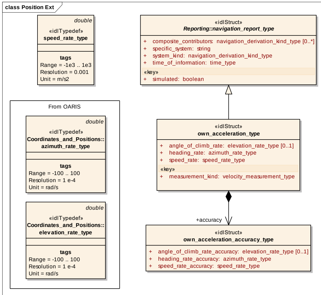
Figure 7.7 Position Ext (Logical diagram)
