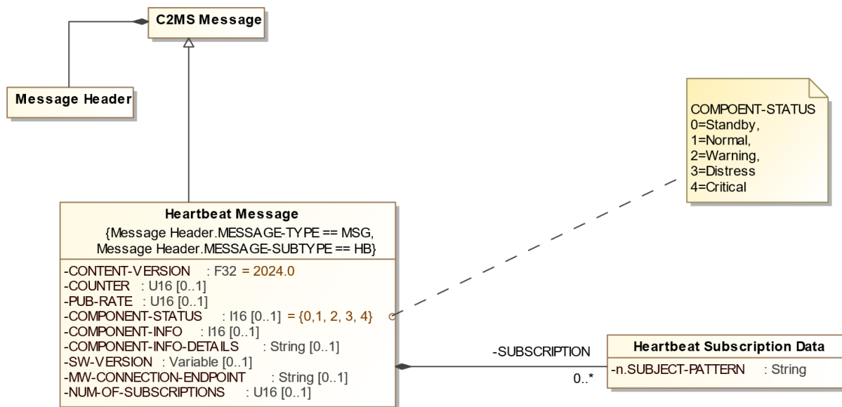
Figure 8-11. Heartbeat Message Diagram
