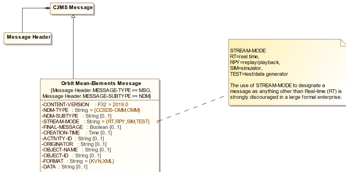
Figure 8-40. Orbit Mean-Elements Message Diagram
