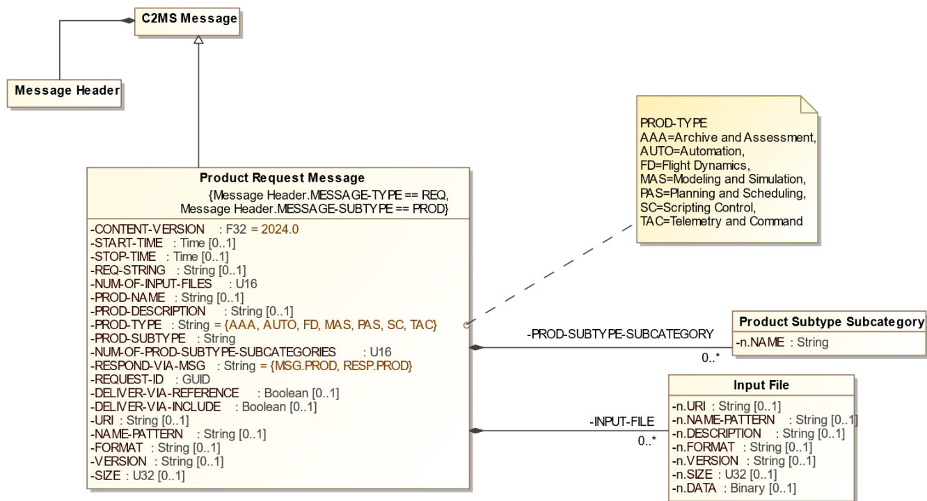
Figure 8-32. Product Request Message Diagram
