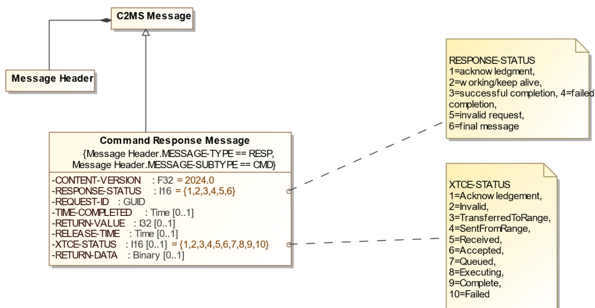
Figure 8-30. Command Response Message Diagram
