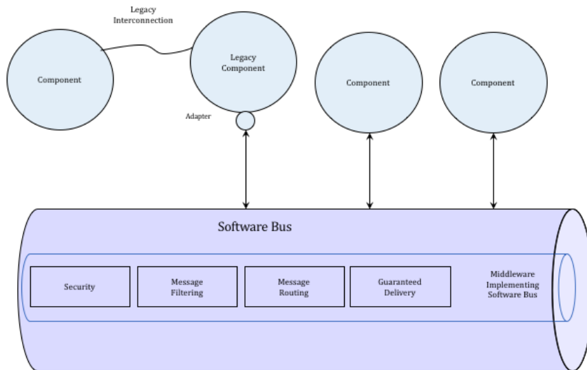
Figure I-1. Original GMSEC API/Bus Features
