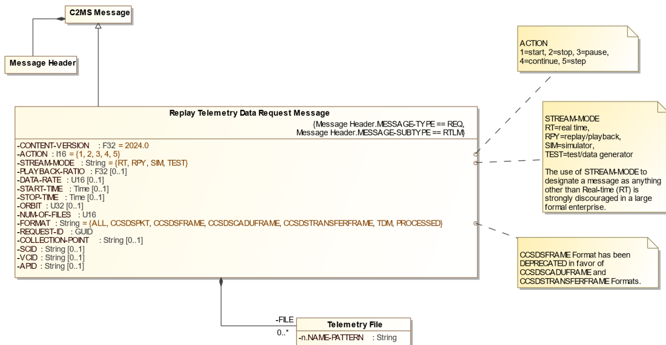
Figure 8-19. Replay Telemetry Data Request Message Diagram
