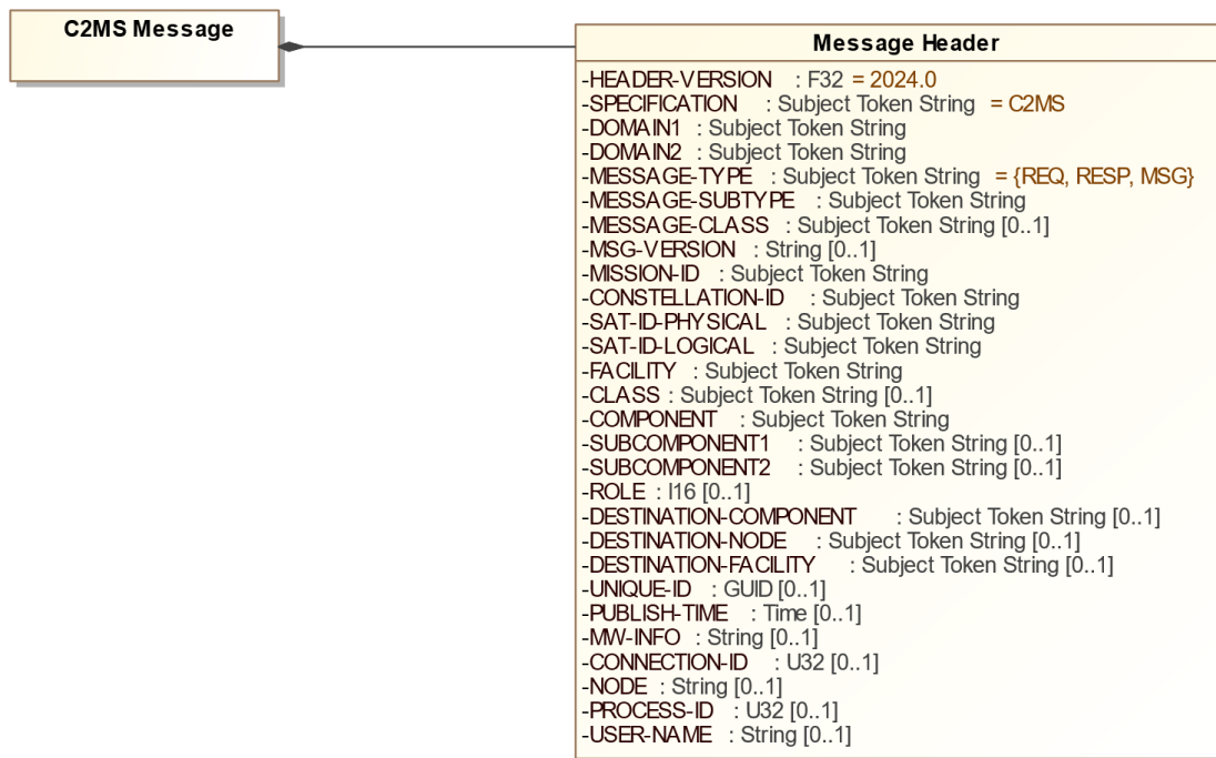
Figure 8-2. Message Header Diagram
