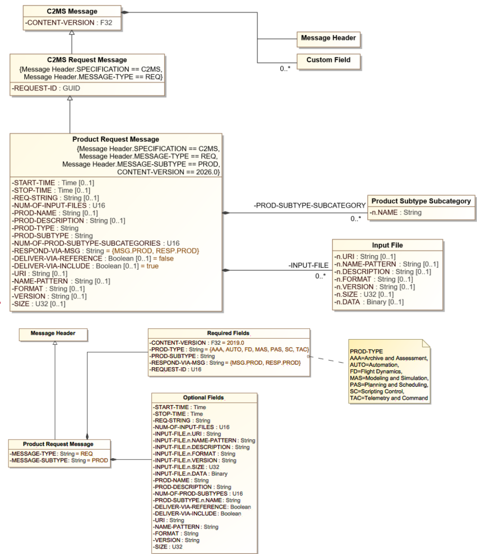
Figure 8-30. Figure 8.38: Product Request Message Diagram
