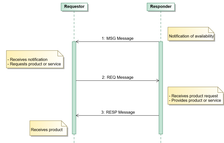
Figure 7.9: Sequence Diagram of Triad 2: Publish/Notify/Request/Response Message Exchange Pattern
