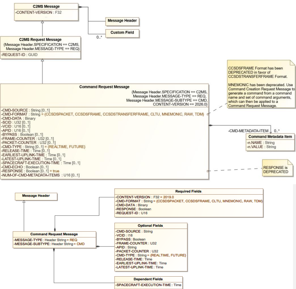
Figure 8-27. Figure 8.33: Command Request Message Contents Diagram
