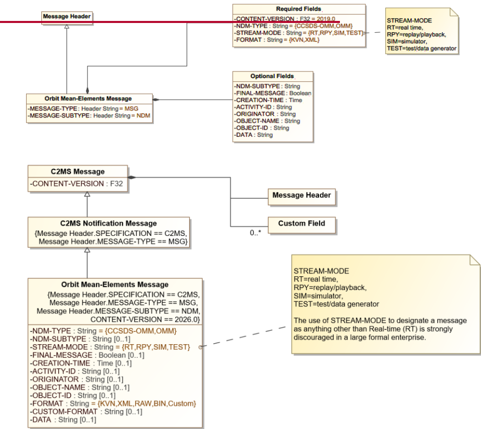
Figure 8-38. 8.46: Orbit Mean-Elements Message Diagram
