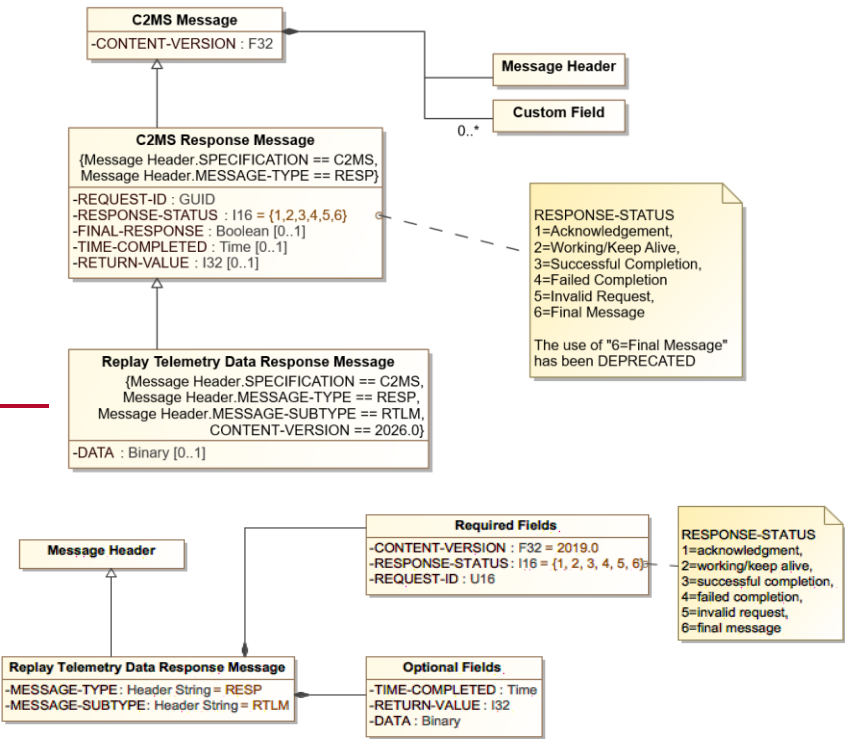
Figure 8.24: Replay Telemetry Data Response Message Diagram
