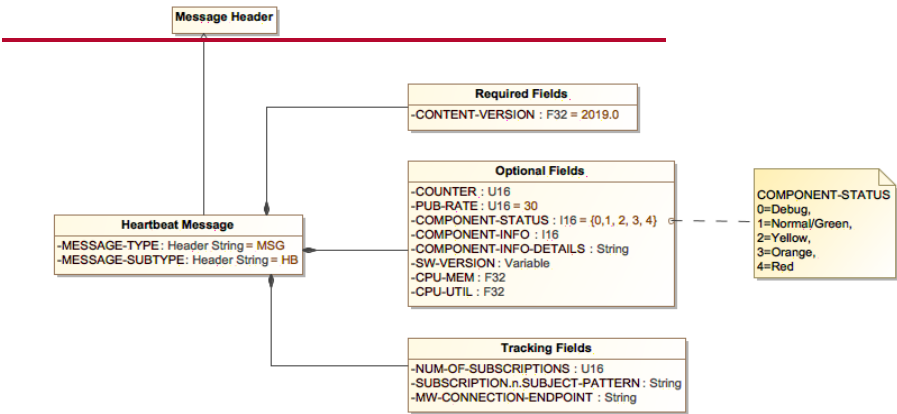
Figure 8-11. Heartbeat Message Diagram
