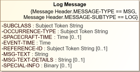
Figure 6.1: Message Field Multiplicity
