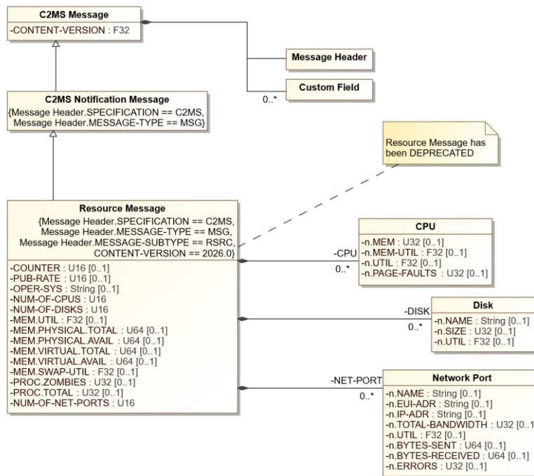
Figure 8.16: Resource Message Diagram
