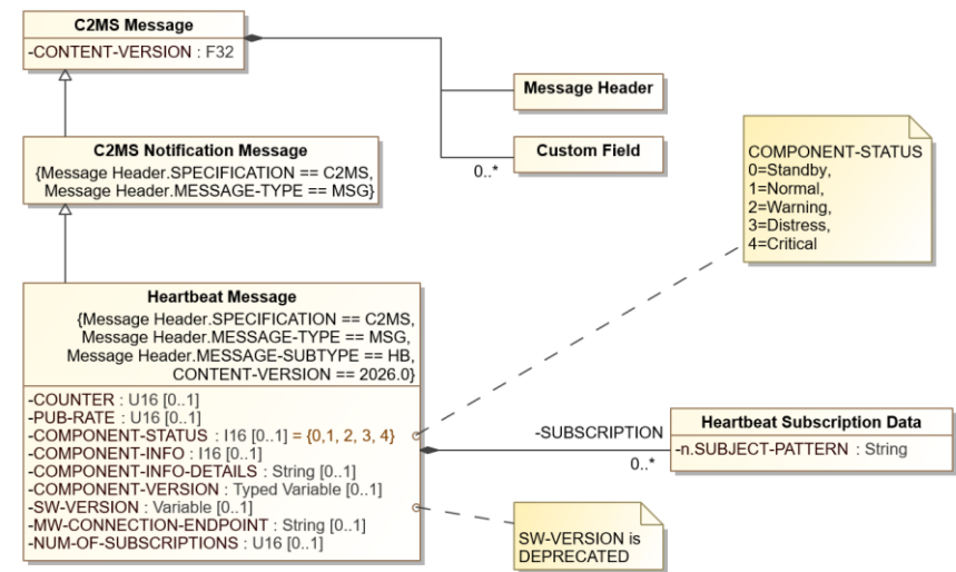
Figure 8.15: Heartbeat Message Diagram
