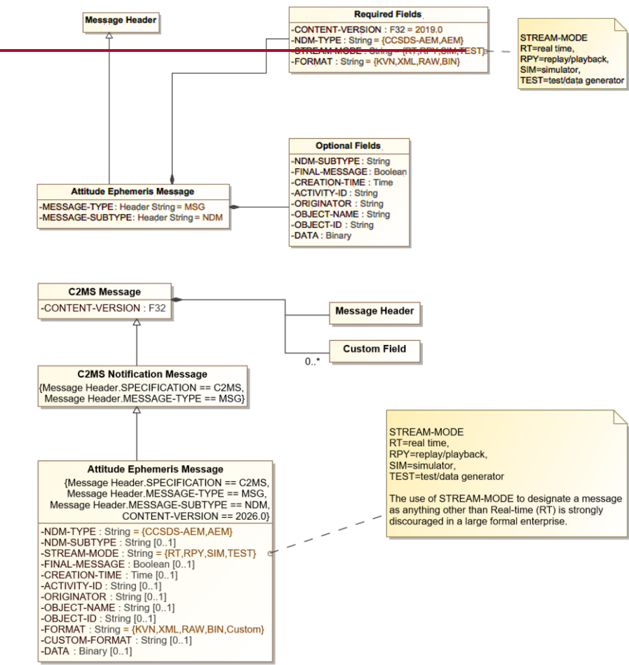
Figure 8-36. 8.44: Attitude Ephemeris Message Diagram
