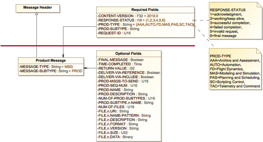
Figure 8-32. Figure 8.40: Product Message Diagram
