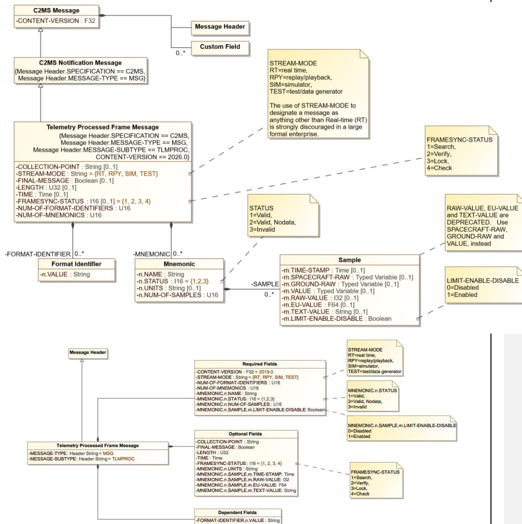
Figure 8-16. 8.22: Telemetry Processed Frame Message Diagram
