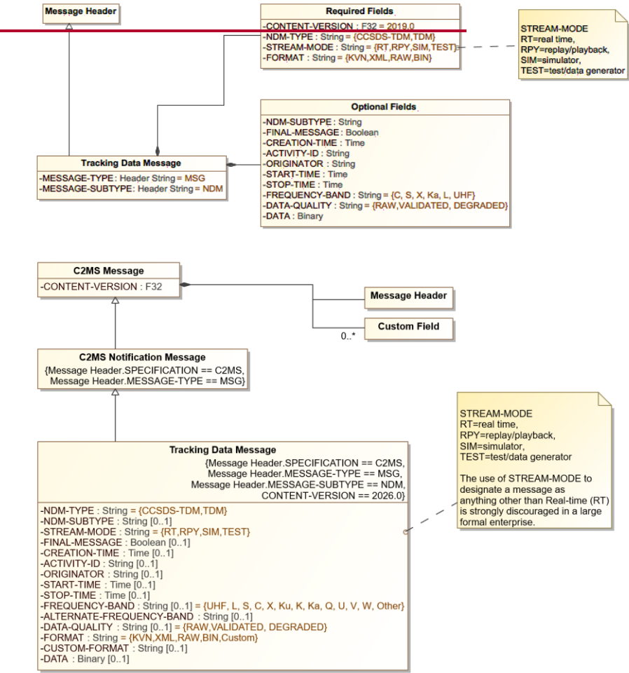
Figure 8-40. — 8.48: Tracking Data Message Diagram
