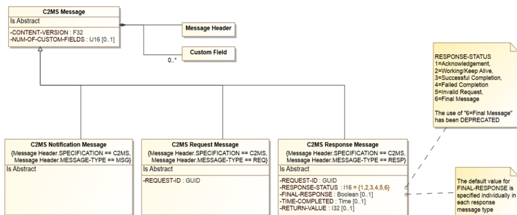
Figure 8.4: C2MS Message Hierarchy
