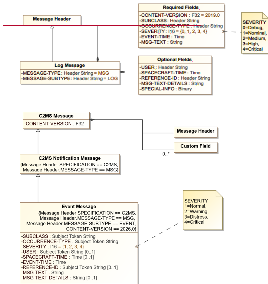
Figure 8.3. Log8.6: Event Message Diagram
