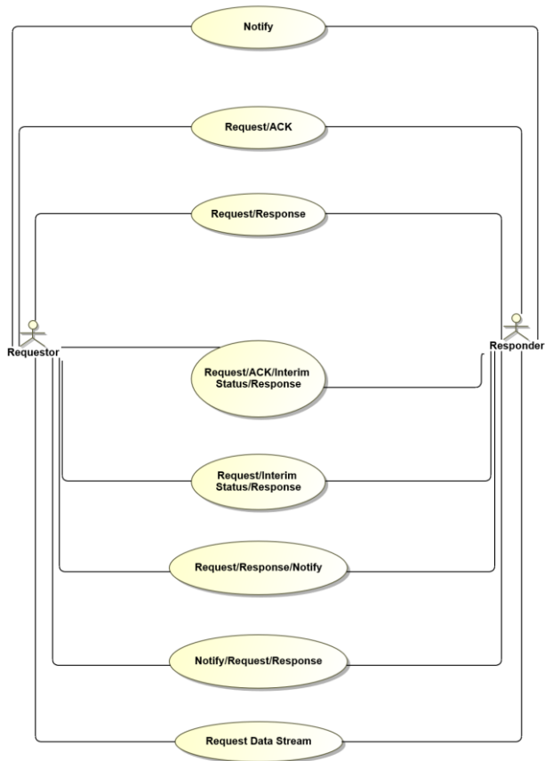
Figure 7-1. Figure 7.1: C2MS Message Exchange Patterns Diagram
