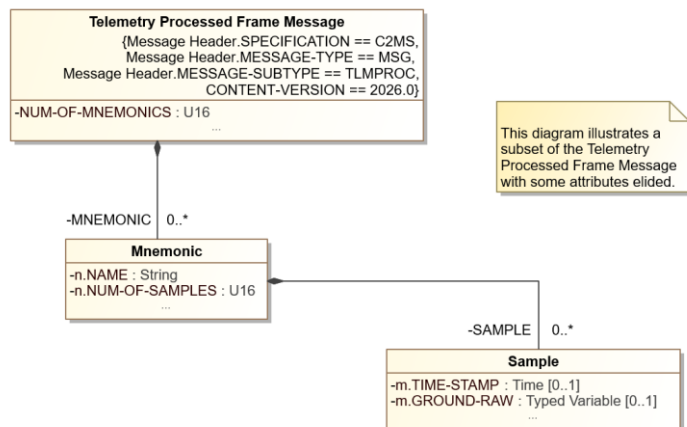
Figure 6.2: Message Series Fields
