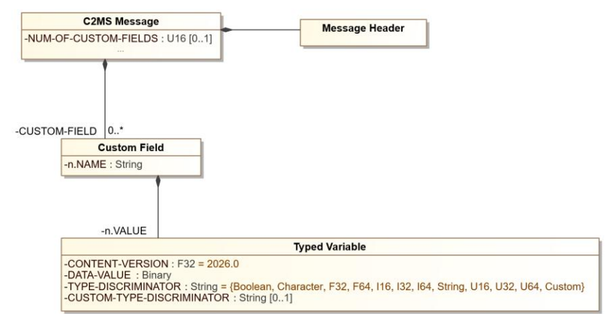
Figure 8.5: Custom Field Diagram
