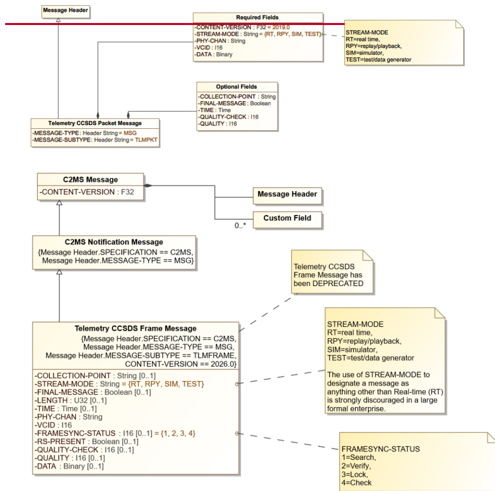
Figure 8-13. 8.18: Telemetry CCSDS PacketFrame Message Diagram
