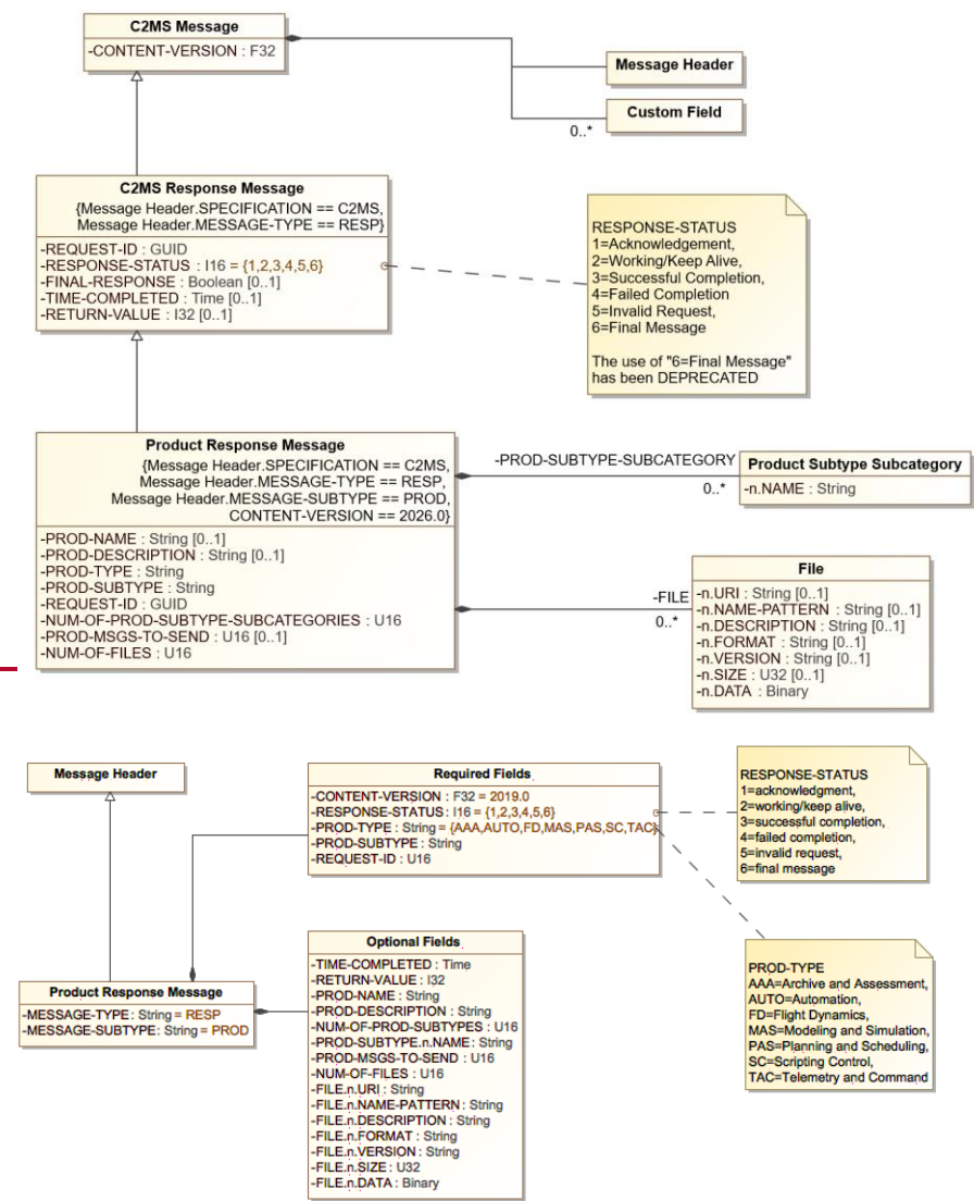
Figure 8-31 below shows a UML object diagram Class Diagram of the Product Response Message with its required and optional fields.
