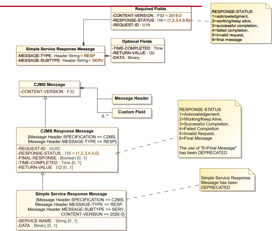
Figure 8-34. 8.42: Simple Service Response Message Diagram
