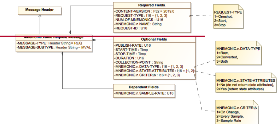
Figure 8-20. Mnemonic Value Request Message Diagram
