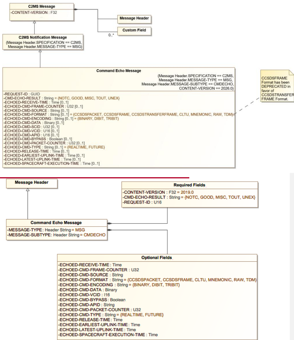
Figure 8-29 belowThe following figure shows a UML object diagram Class Diagram of the Command Echo Message with its required and optional fields.
