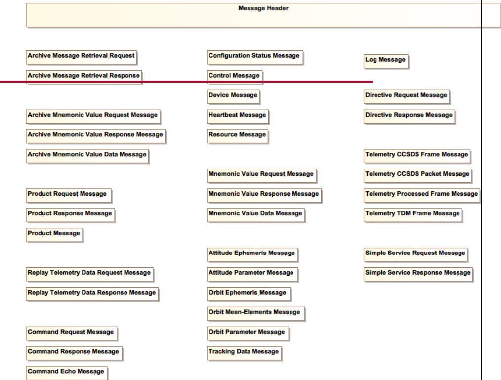
Figure 8-1. High Level UML Class Diagram
