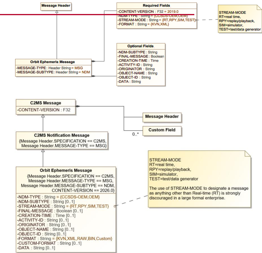
Figure 8-39. 8.47: Orbit Ephemeris Message Diagram
