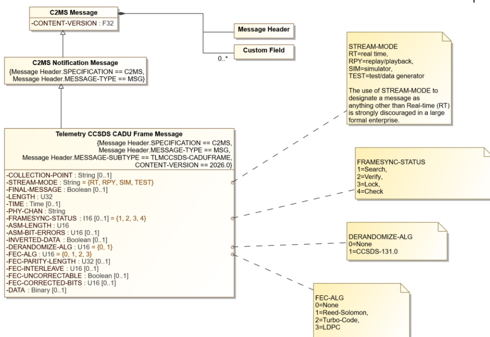
Figure 8.19: Telemetry CCSDS CADU Frame Message Diagram
