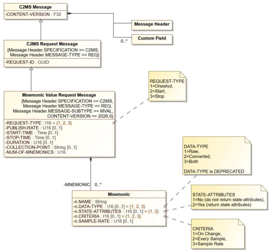
Figure 8-20 below shows a UML object diagram Class Diagram of the Mnemonic Value Request Message with its required, optional, and dependent fields.
