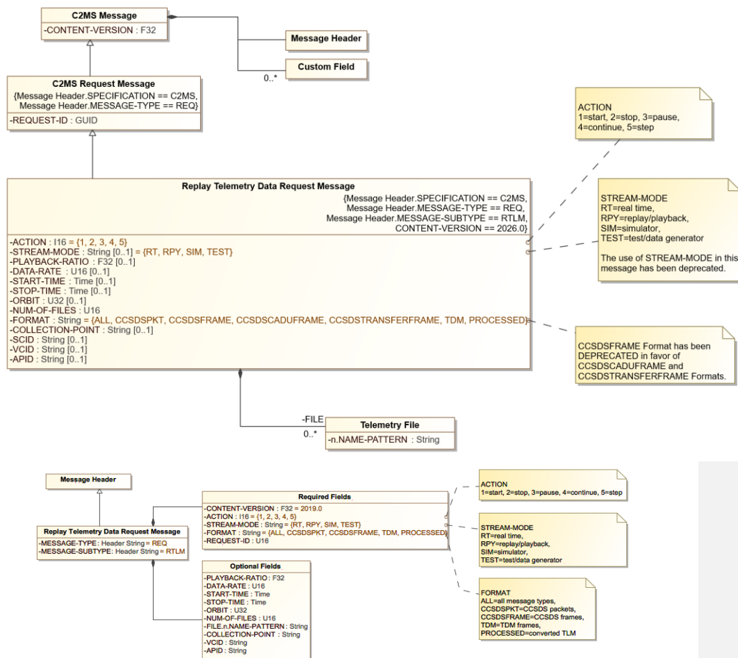
Figure 8-17. 8.23: Replay Telemetry Data Request Message Diagram
