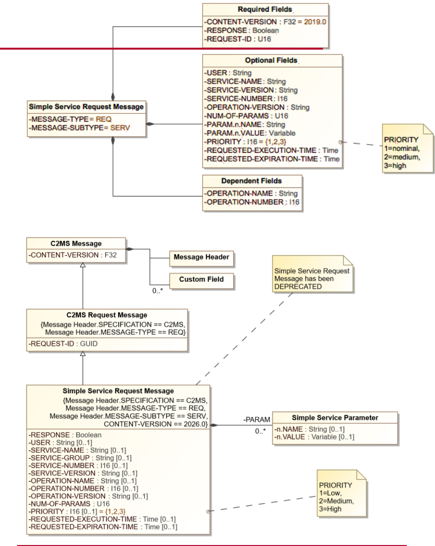
Figure 8-33 belowThe following figure shows a UML object diagram Class Diagram of the Simple Service Request Message with its required and optional fields.
