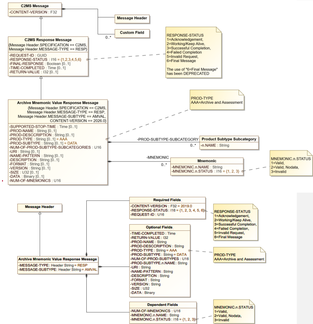
Figure 8-24. 8.30: Archive Mnemonic Value Response Message Diagram
