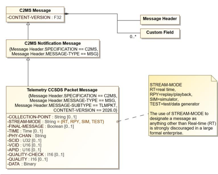
Figure 8.17: Telemetry CCSDS Packet Message Diagram
