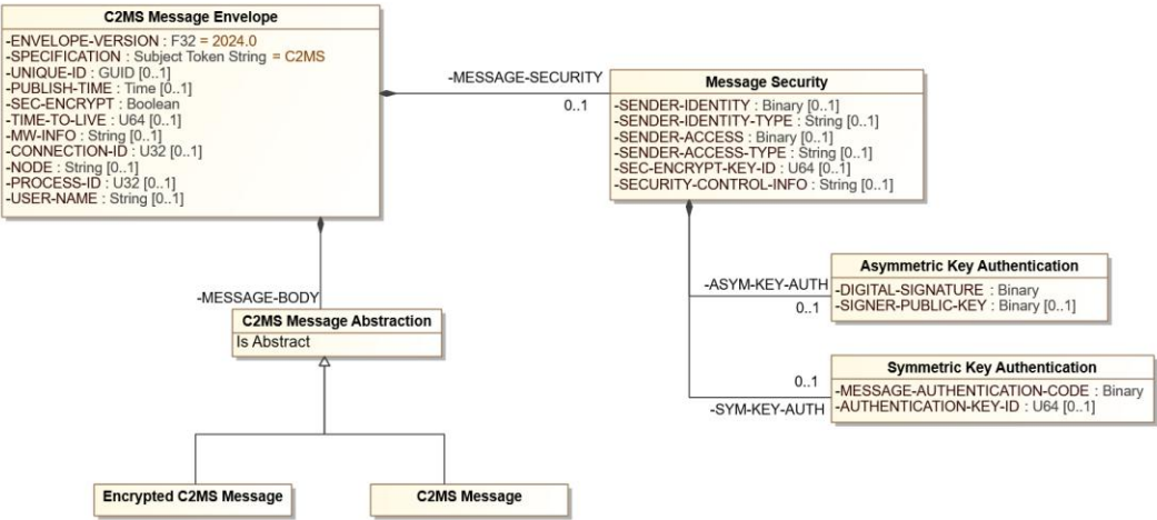
Figure 8.1: C2MS Message Envelope Diagram
