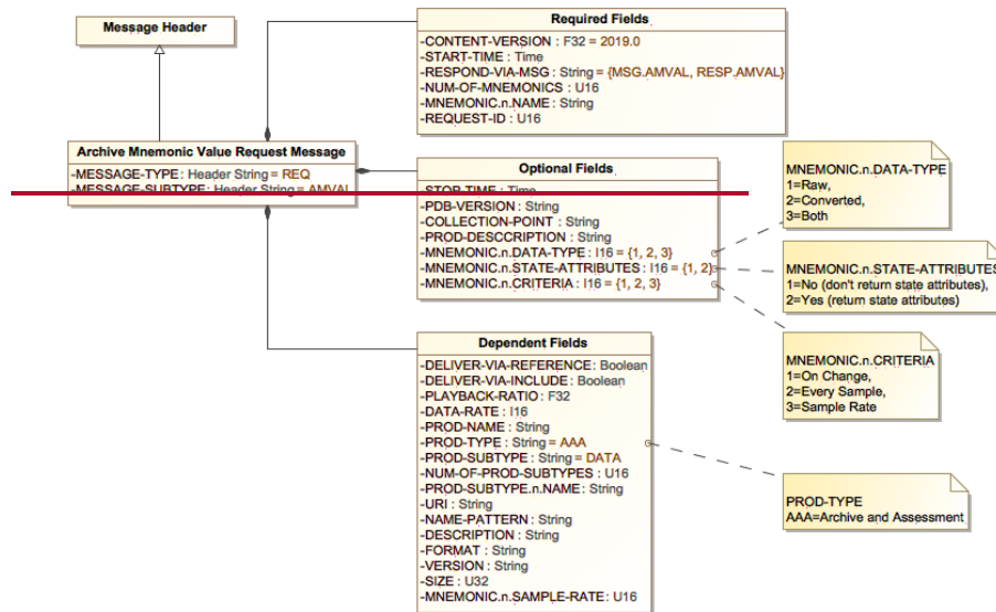
Figure 8-23. Figure 8.29: Archive Mnemonic Value Request Message Diagram
