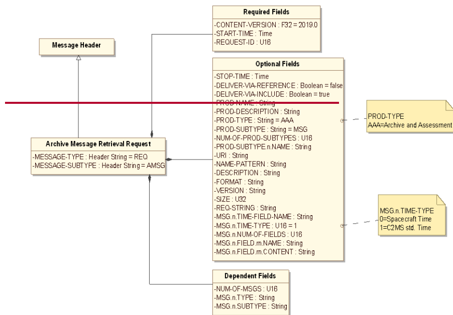
Figure 8-4. Figure 8.8: Archive Message Retrieval Request Diagram
