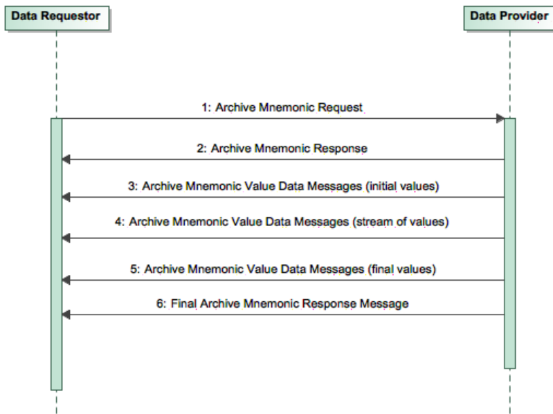
Figure 8.25. — 8.31: Archive Mnemonic Value Message Sequence Diagram
