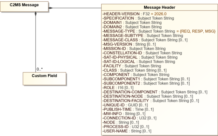
Figure 8.3: Message Header Diagram
