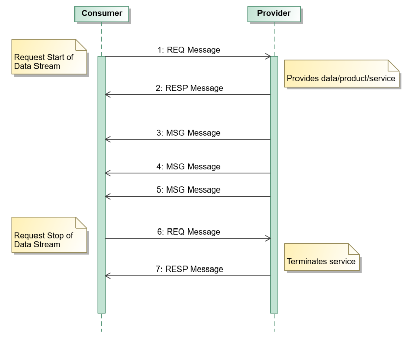
Figure 7.10: Sequence Diagram of Request Data Stream Message Exchange Pattern
