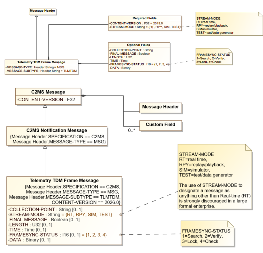
Figure 8-15. 8.21: Telemetry TDM Frame Message Diagram
