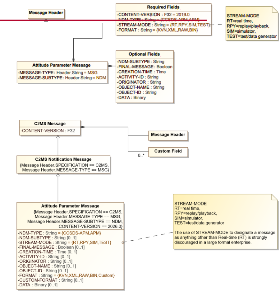
Figure 8-35. 8.43: Attitude Parameter Message Diagram
