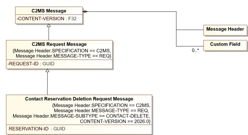
Figure 8.52: Contact Reservation Deletion Request Message Diagram
