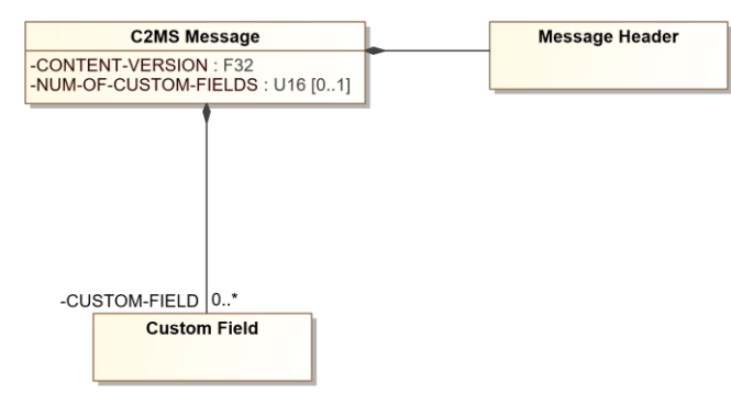
Figure 8.2: C2MS Message Diagram
