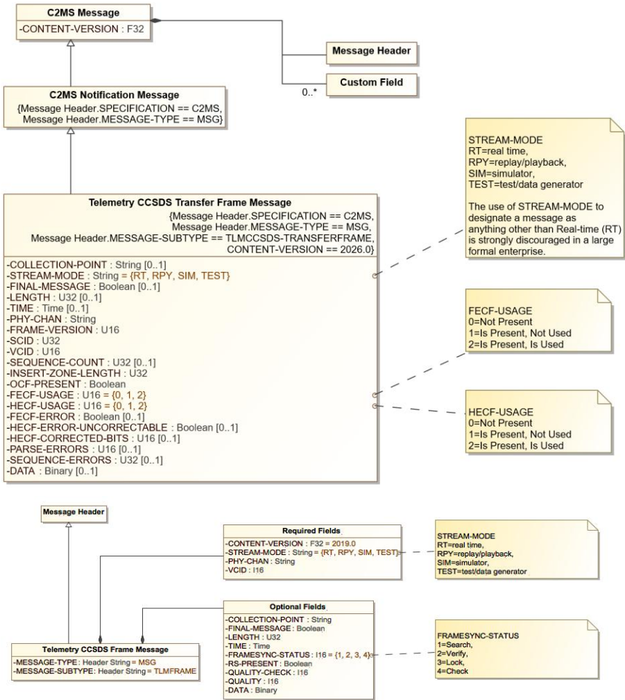
Figure 8-14. 8.20: Telemetry CCSDS Transfer Frame Message Diagram
