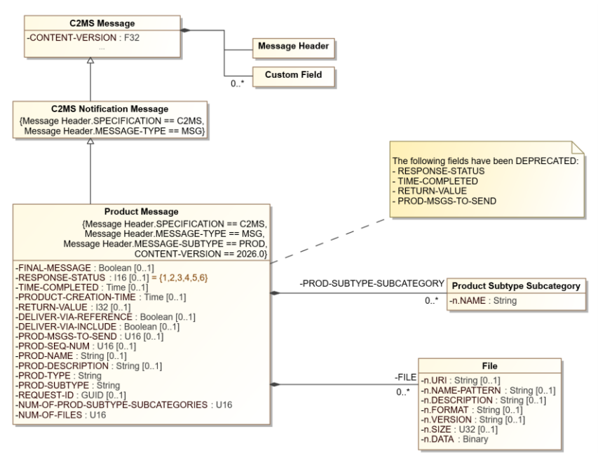
Figure 8-32 below The following figure shows a UML object diagram Class Diagram of the Product Message
