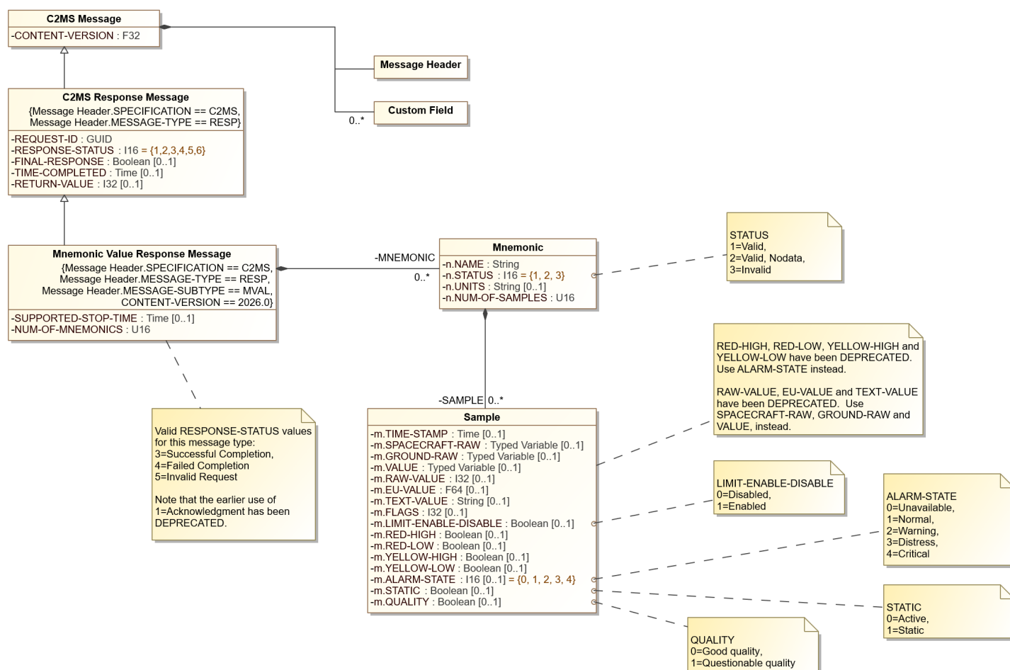
Figure 8.27: Mnemonic Value Response Message Diagram
