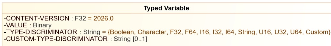
Figure 6.3: Variable Type Diagram
