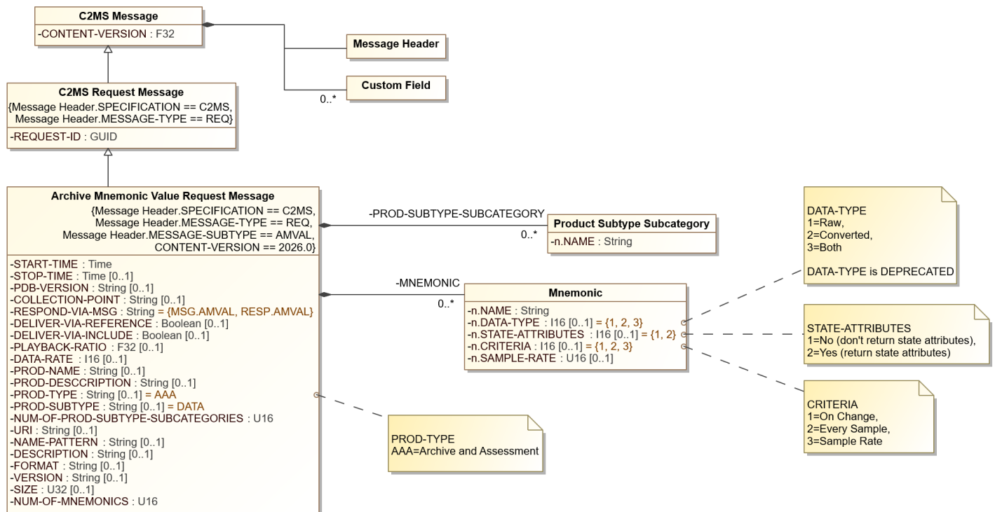
Figure 8.29: Archive Mnemonic Value Request Message Diagram
