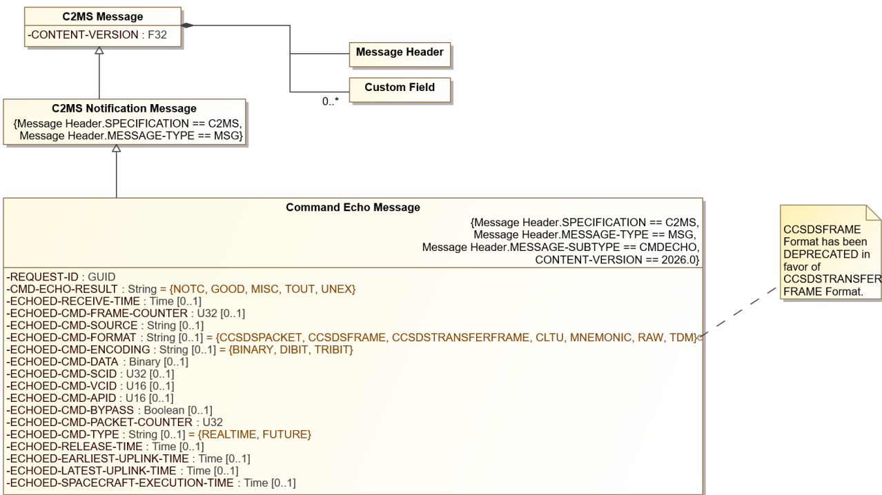
Figure 8.35: Command Echo Message Diagram
