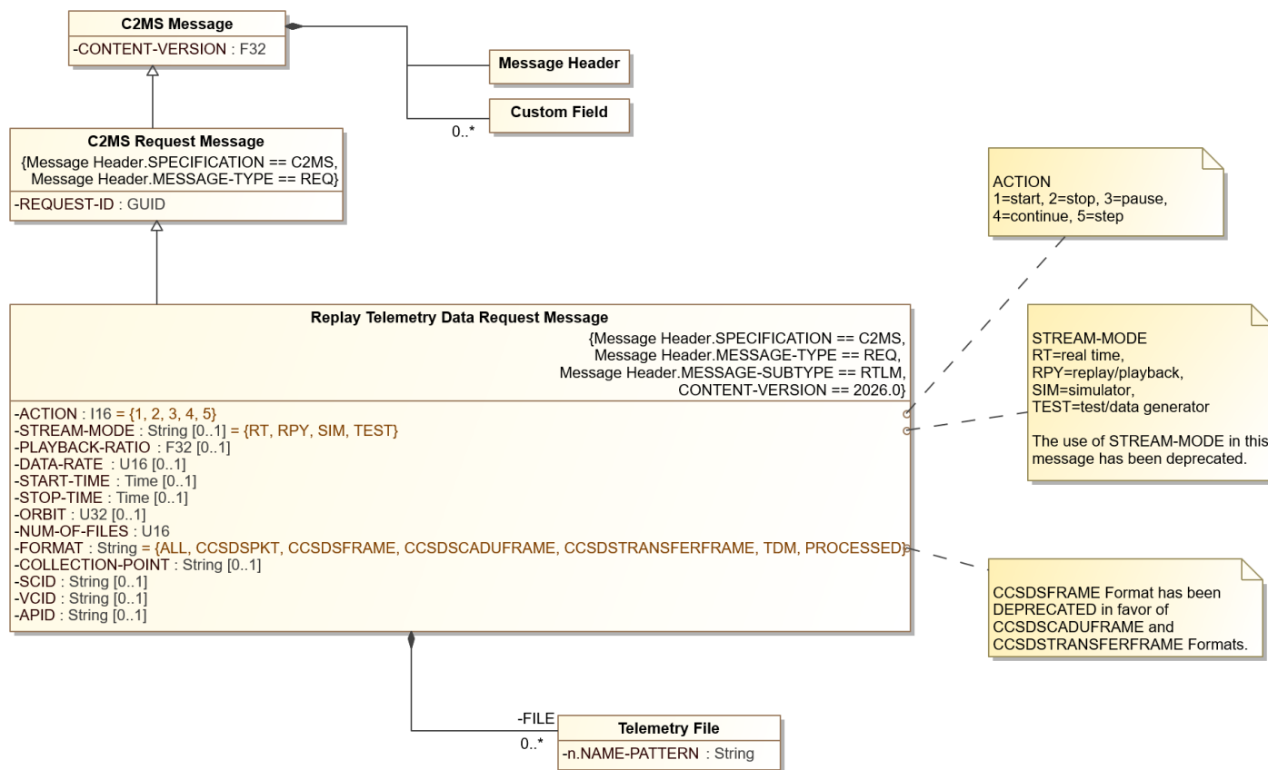
Figure 8.23: Replay Telemetry Data Request Message Diagram
