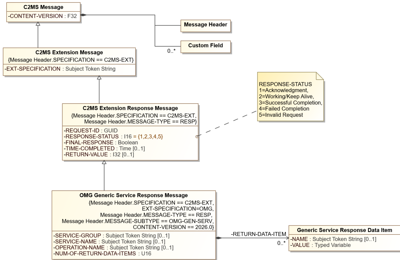
Figure 9.3: OMG Generic Service Response Message Diagram
