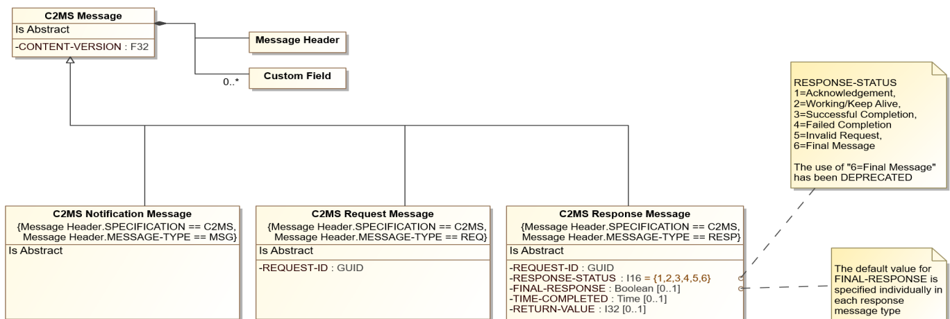
Figure 8.4: C2MS Message Hierarchy
