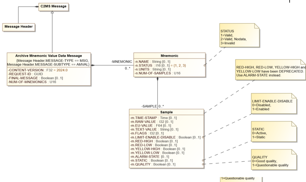
Figure 8-28. 8.32: Archive Mnemonic Value Data Message Diagram
