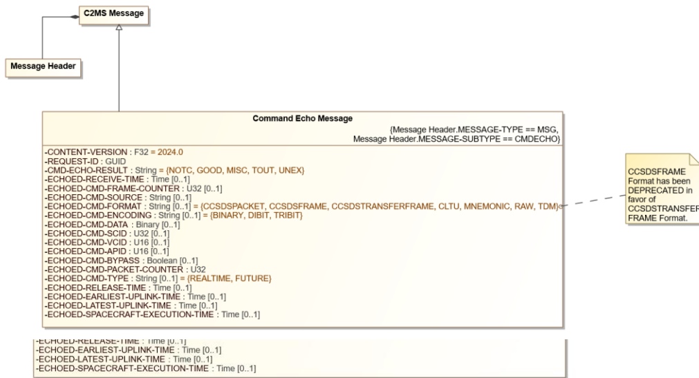
Figure 8-31. 8.34. 8.35. Command Echo Message Diagram
