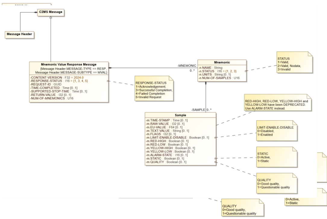
Figure 8-23. 8.27: Mnemonic Value Response Message Diagram
