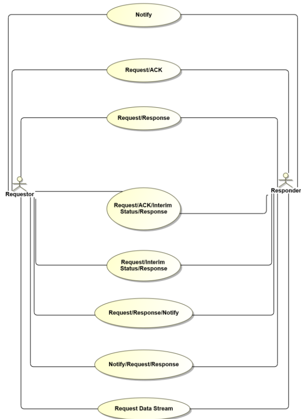
Figure 7-1. — 7.1: C2MS Message Exchange Patterns Diagram
