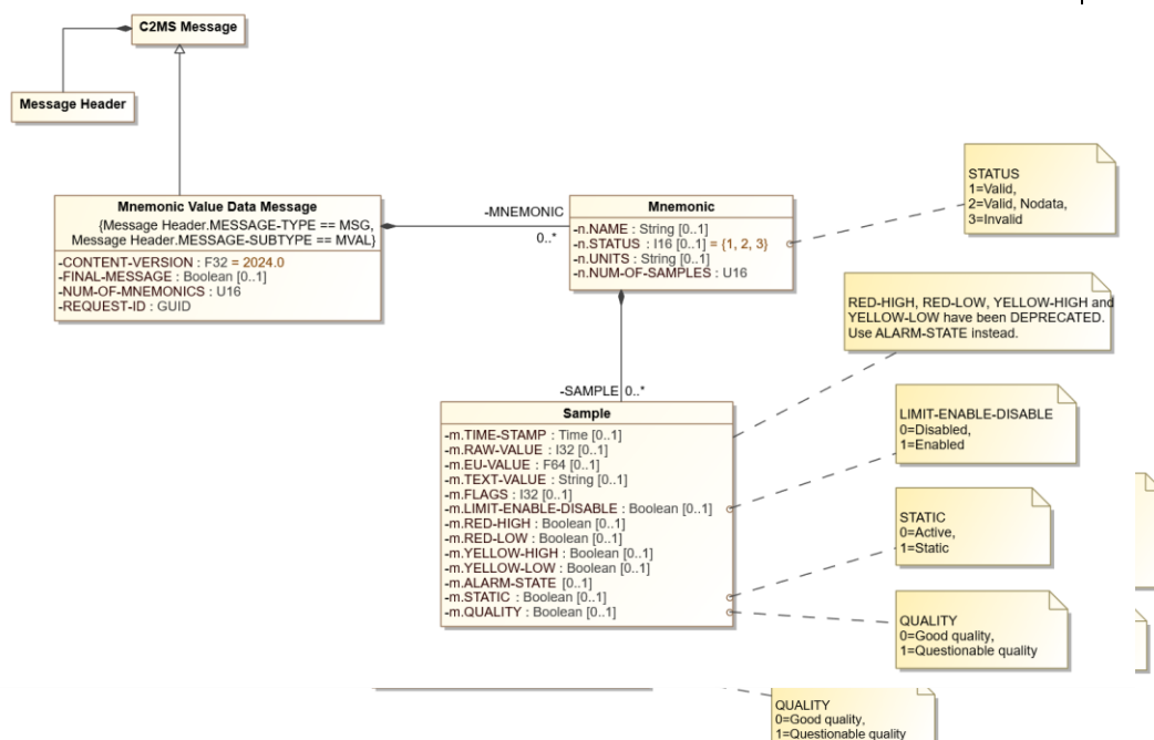
Figure 8-24. 8.28: Mnemonic Value Data Message Diagram
