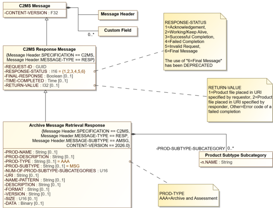
Figure 8.9: Archive Message Retrieval Response Diagram
