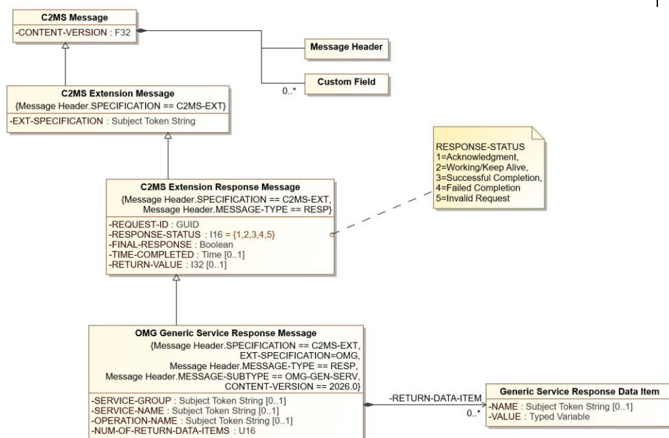
Figure 9.3: OMG Generic Service Response Message Diagram
