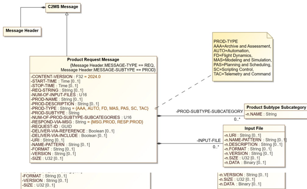
Figure 8-32. 8-38 Product Request Message Diagram
