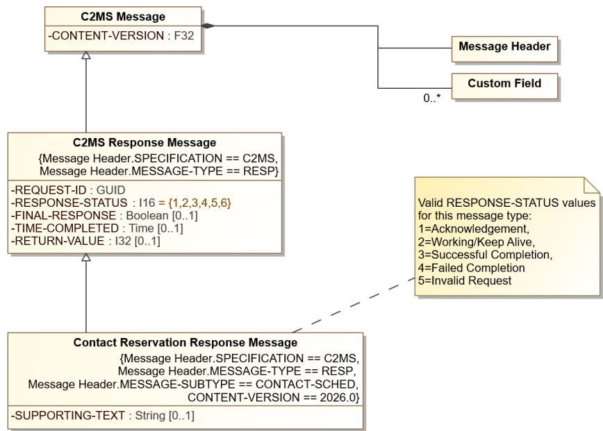
Figure 8.51: Contact Reservation Response Message Diagram
