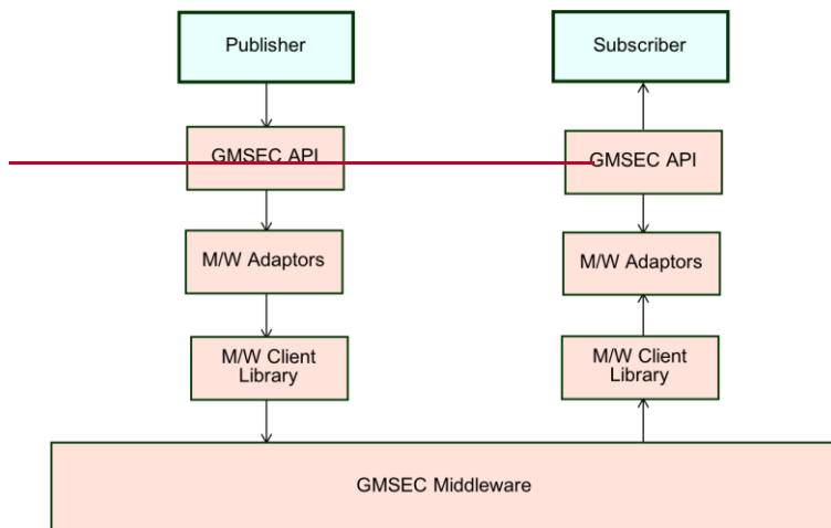
Figure I-3. GMSEC Middleware Abstraction Layers
