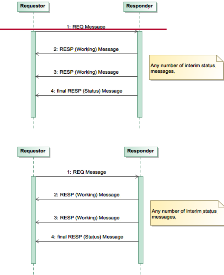
Figure 7-7. 7.7. Sequence Diagram of Request/Interim Status/Response Message Exchange Pattern
