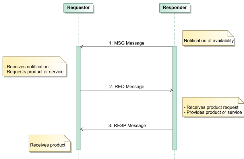
Figure 7.9. 7.9. Sequence Diagram of Triad 2: Publish Notify/Request/Response Message Exchange Pattern
