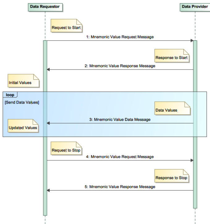
Figure 8-21. 8.25 Mnemonic Value Message Sequence Diagram
