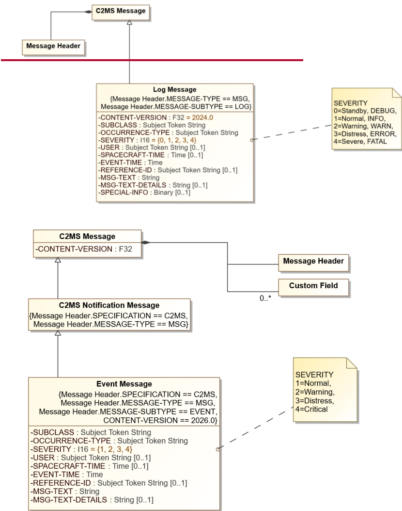
Figure 8-3. Log8.6: Event Message Diagram
