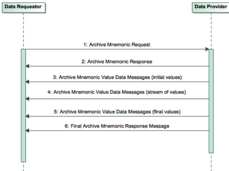
Figure 8-27. 8.31: Archive Mnemonic Value Message Sequence Diagram
