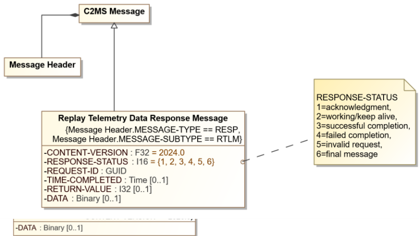
Figure 8-20. 8.24 Replay Telemetry Data Response Message Diagram
