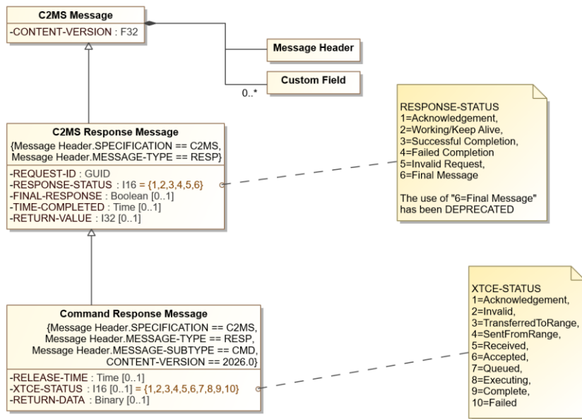
Figure 8-30. 8.34: Command Response Message Diagram
