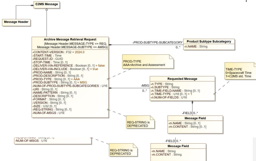
Figure 8-4. Figure 8.8: Archive Message Retrieval Request Diagram
