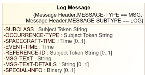
Figure 6-2. 6.1: Message Field Multiplicity
