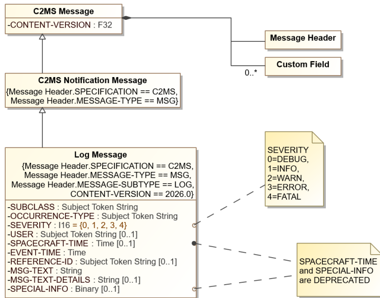
Figure 8.7: Log Message Diagram
