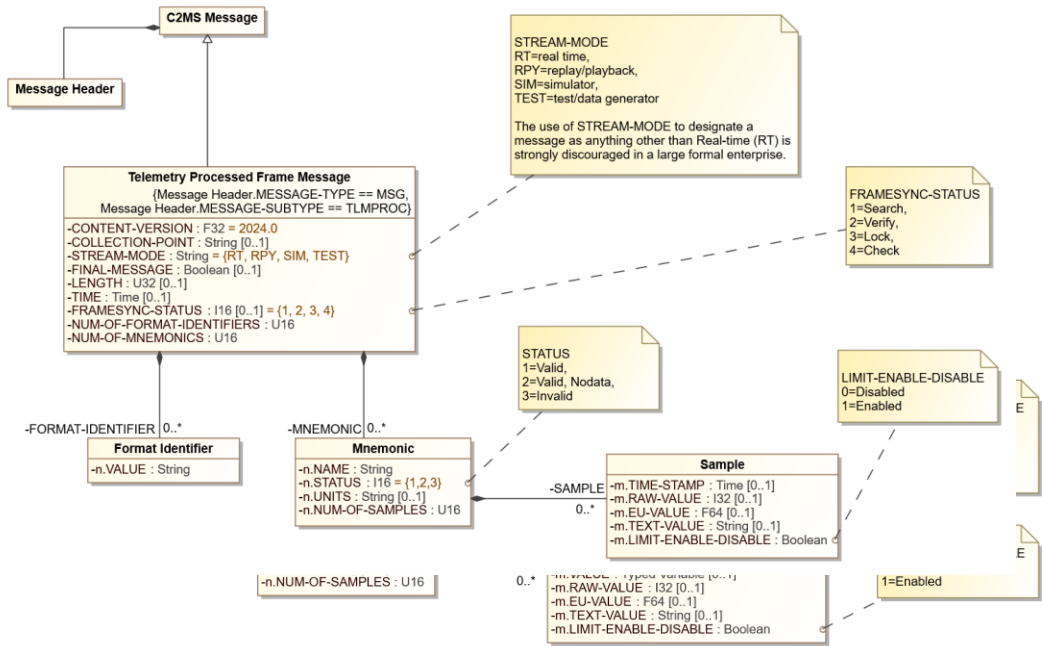
Figure 8.22: Telemetry Processed Frame Message Diagram
