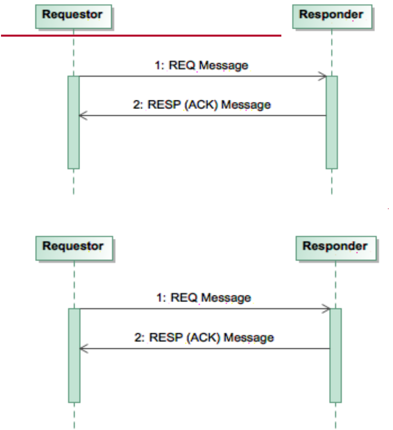
Figure 7.3. 7.3. Sequence Diagram of Request/ACK
