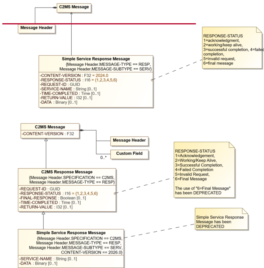
Figure 8-36.8.42: Simple Service Response Message Diagram
