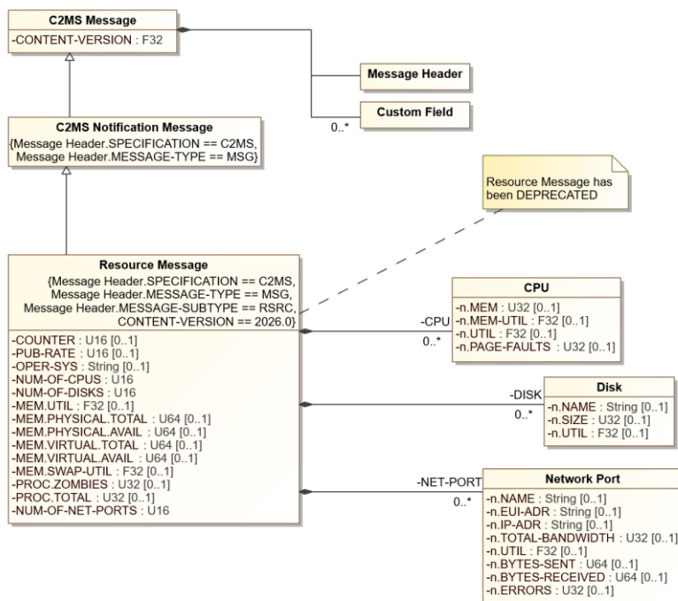
Figure 8-12. 8.16: Resource Message Diagram
