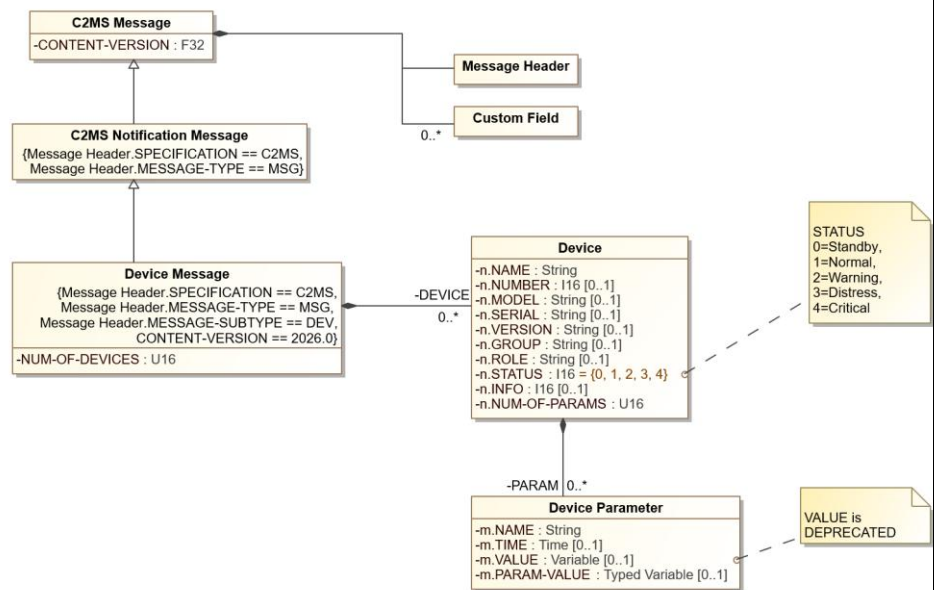
Figure 8.14: Device Message Diagram
