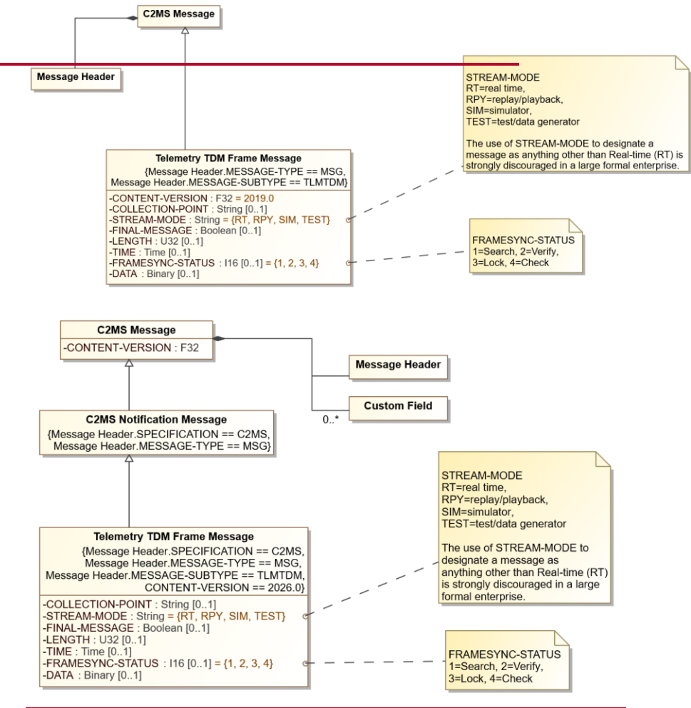
Figure 8-17. 8.21: Telemetry TDM Frame Message Diagram
