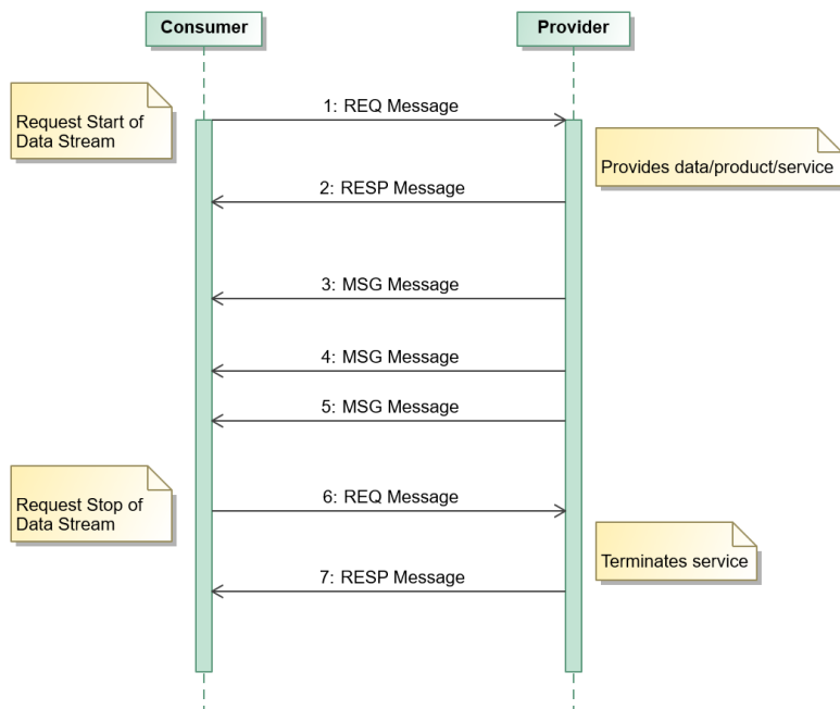
Figure 7-10. — 7.10: Sequence Diagram of Subscription Request Data Stream Message Exchange Pattern
