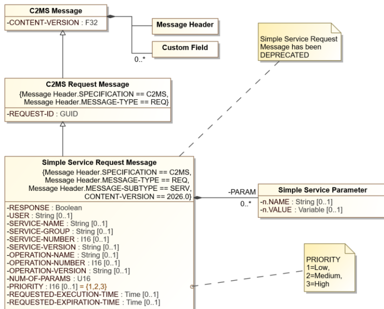
Figure 8-35.8.41: Simple Service Request Message Diagram
