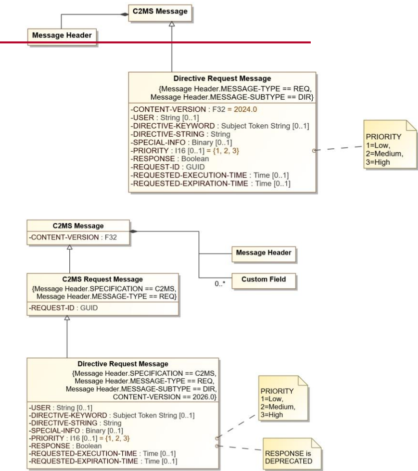
Figure 8-6. 8.10: Directive Request Diagram
