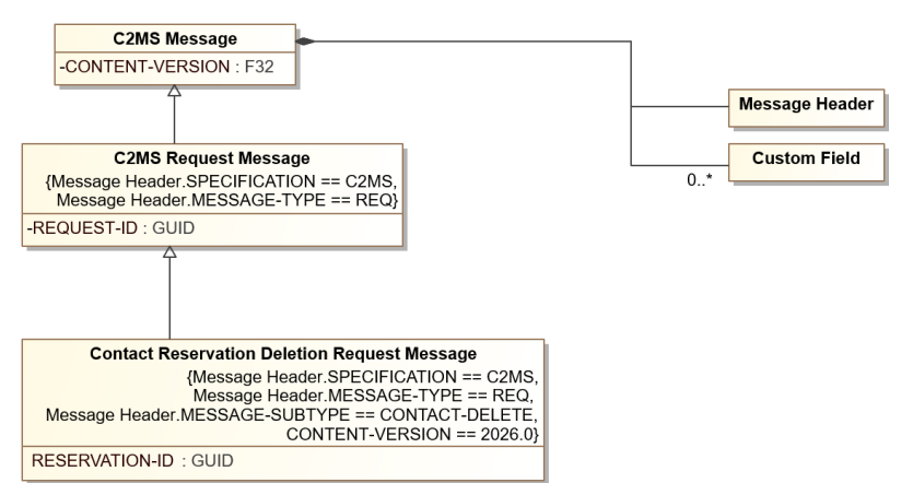
Figure 8.52: Contact Reservation Deletion Request Message Diagram
