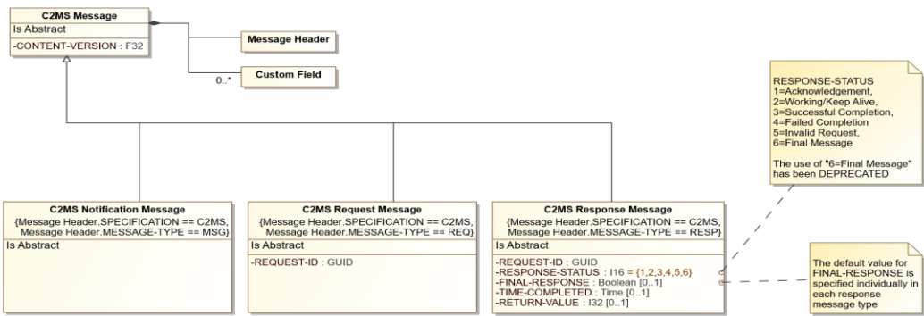
Figure 8.4: C2MS Message Hierarchy
