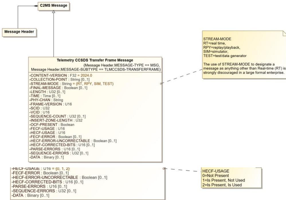
Figure 8-16. — 8.20: Telemetry CCSDS Transfer Frame Message Diagram
