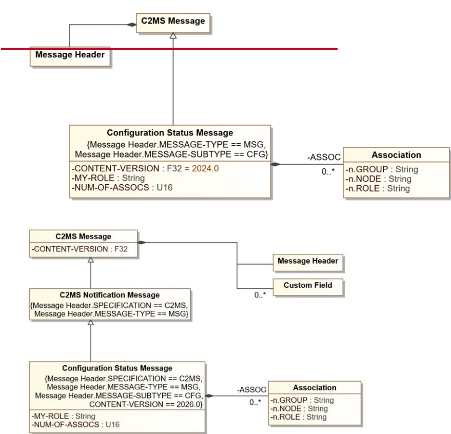
Figure 8-8. 8.12: Configuration Status Message Diagram
