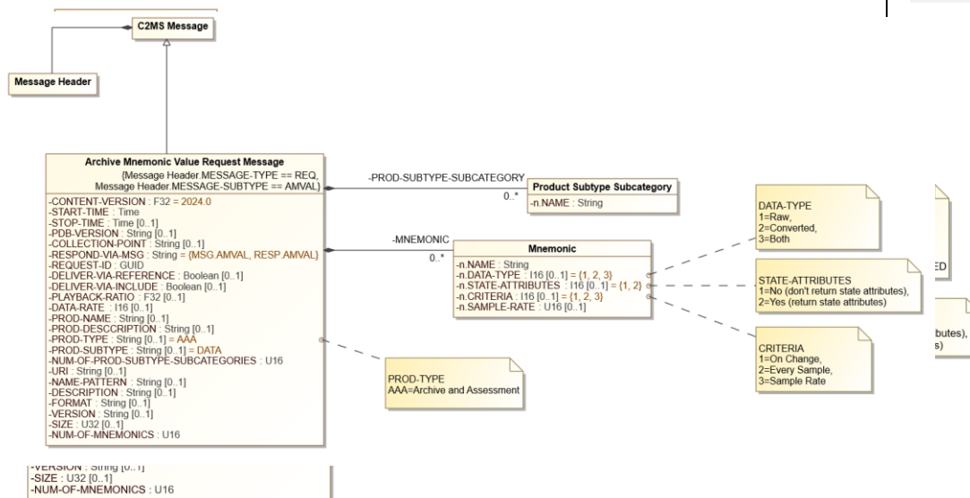
Figure 8-25. 8.29: Archive Mnemonic Value Request Message Diagram
