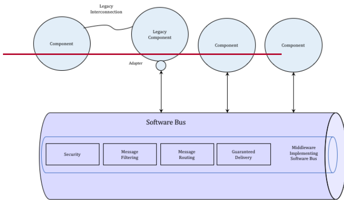
Figure I-1. Original GMSEC API/Bus Features
