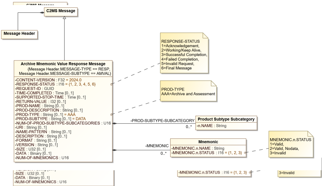
Figure 8-26. 8-30 Archive Mnemonic Value Response Message Diagram
