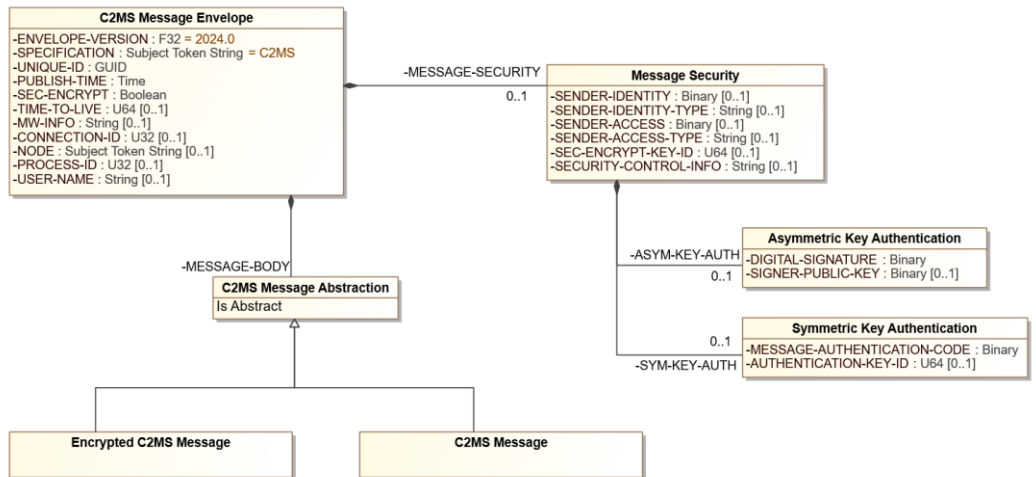
Figure 8-1. 8.1: C2MS Message Envelope Diagram
