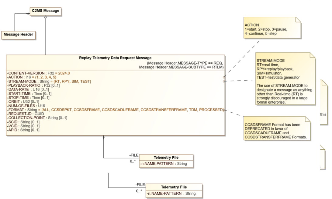
Figure 8-19. 8.23: Replay Telemetry Data Request Message Diagram
