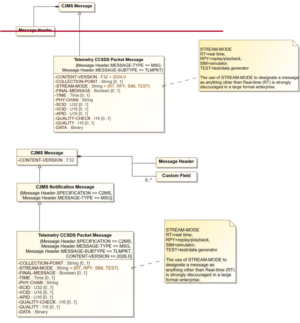
Figure 8-13. 8.17: Telemetry CCSDS Packet Message Diagram
