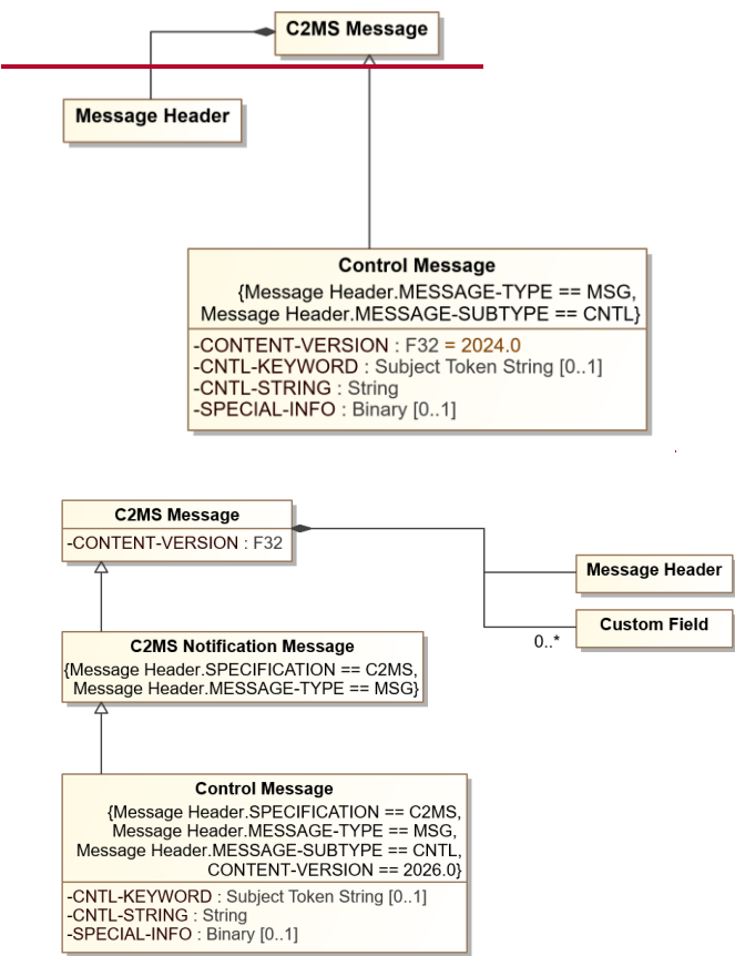
Figure 8-9. 8.13: Control Message Diagram
