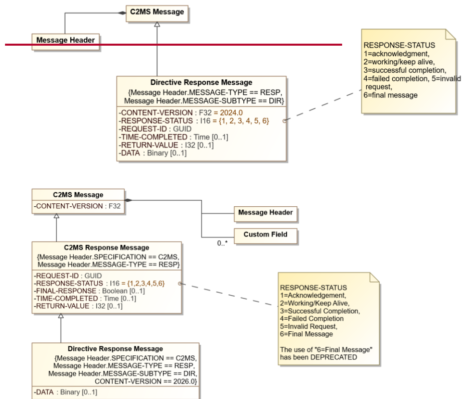
Figure 8-7. — 8.11: Directive Response Diagram
