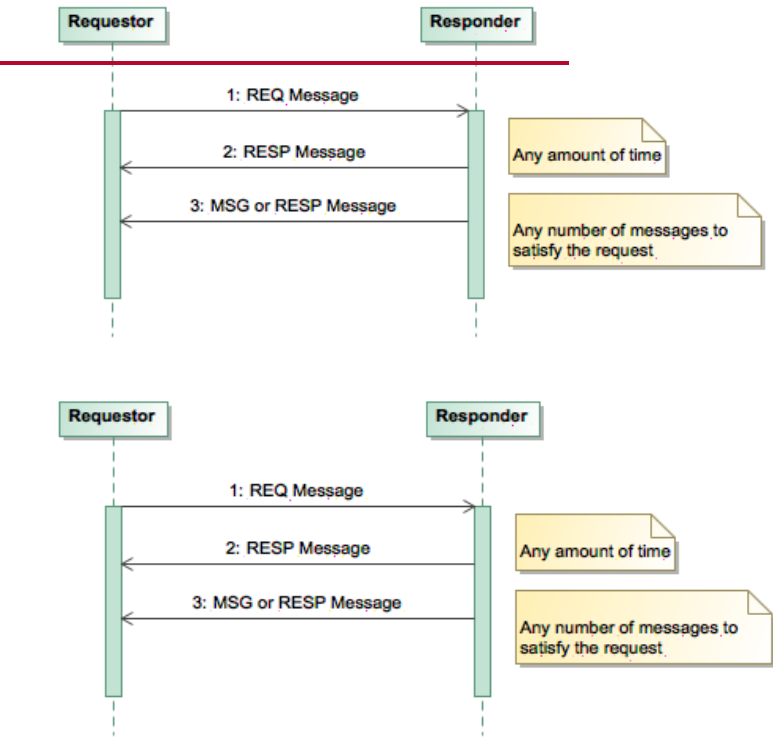
Figure 7-8. 7.8. Sequence Diagram of Triad 1: Request/Response/ Publish Notify Message Exchange Pattern
