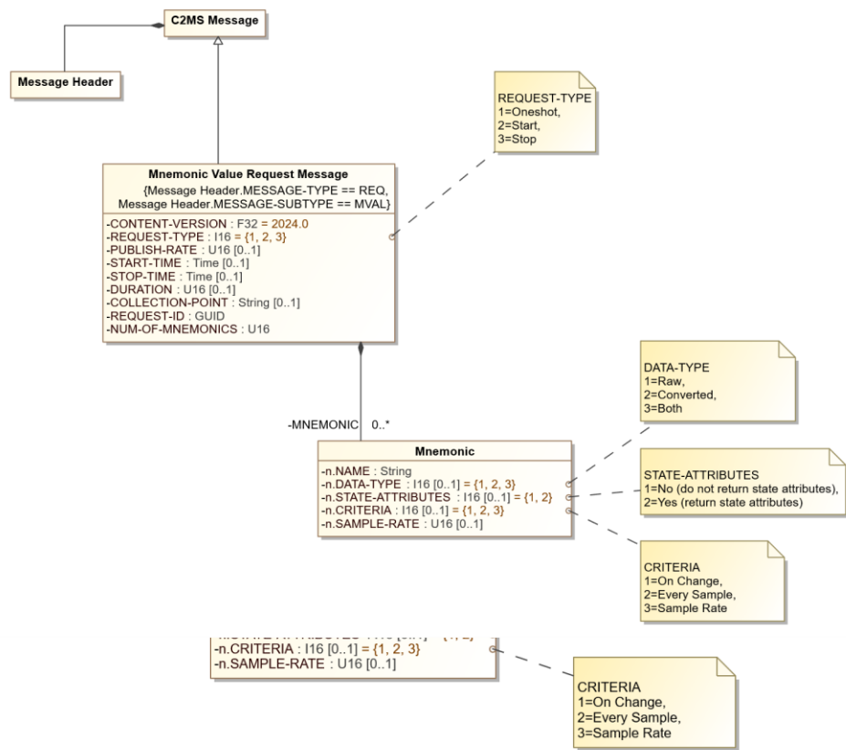
Figure 8-22. 8.26: Mnemonic Value Request Message Diagram
