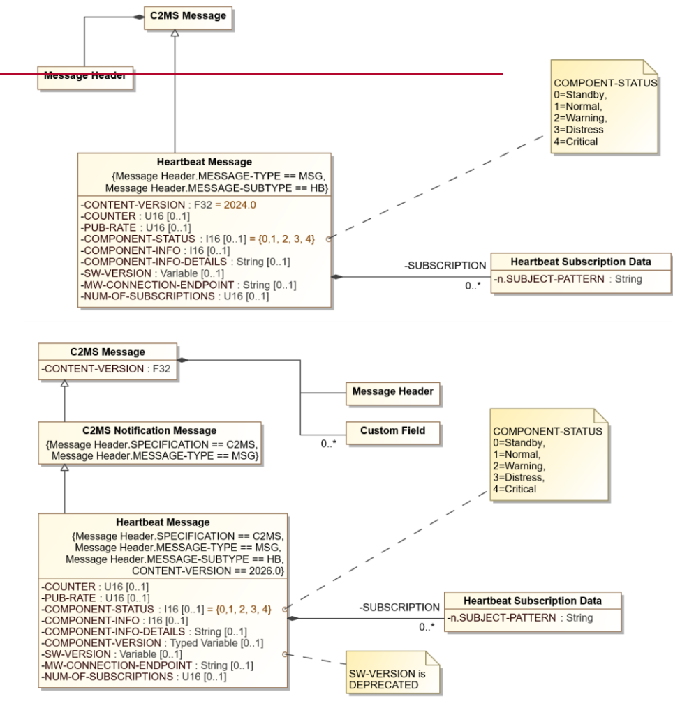
Figure 8-11. 8.15: Heartbeat Message Diagram
