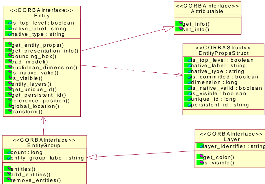
Figure 2-3 UML Diagram of CadFoundation Module
