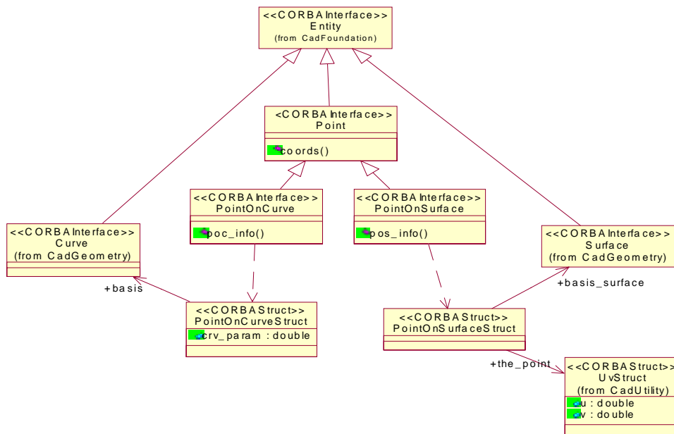
Figure 2-7 UML Diagram of CadGeometryExtens Interfaces and Data Structures
