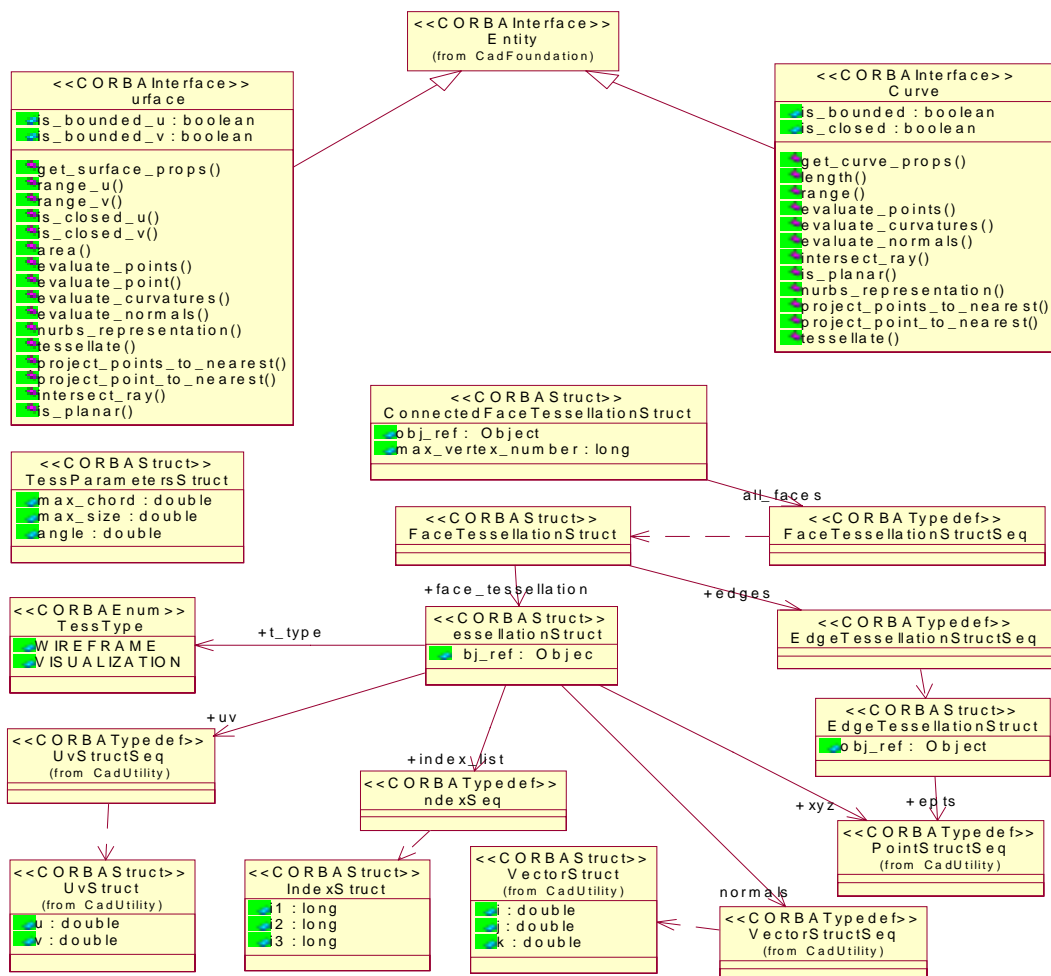
Figure 2-4 UML Diagram of CadGeometry Interfaces and Data Structures
