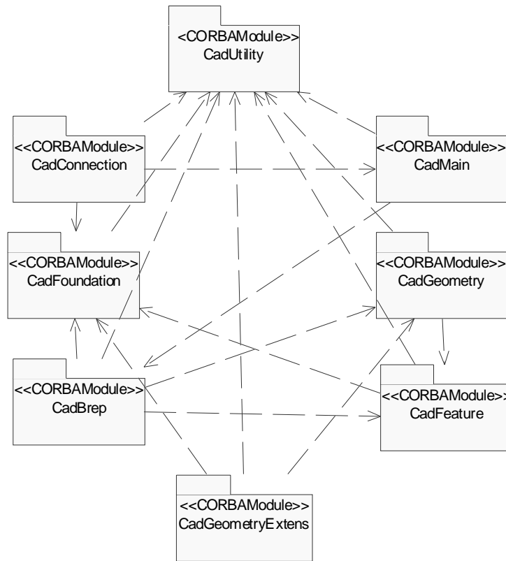
Figure 1-2 Module Interdependencies and Overall Module Structure
