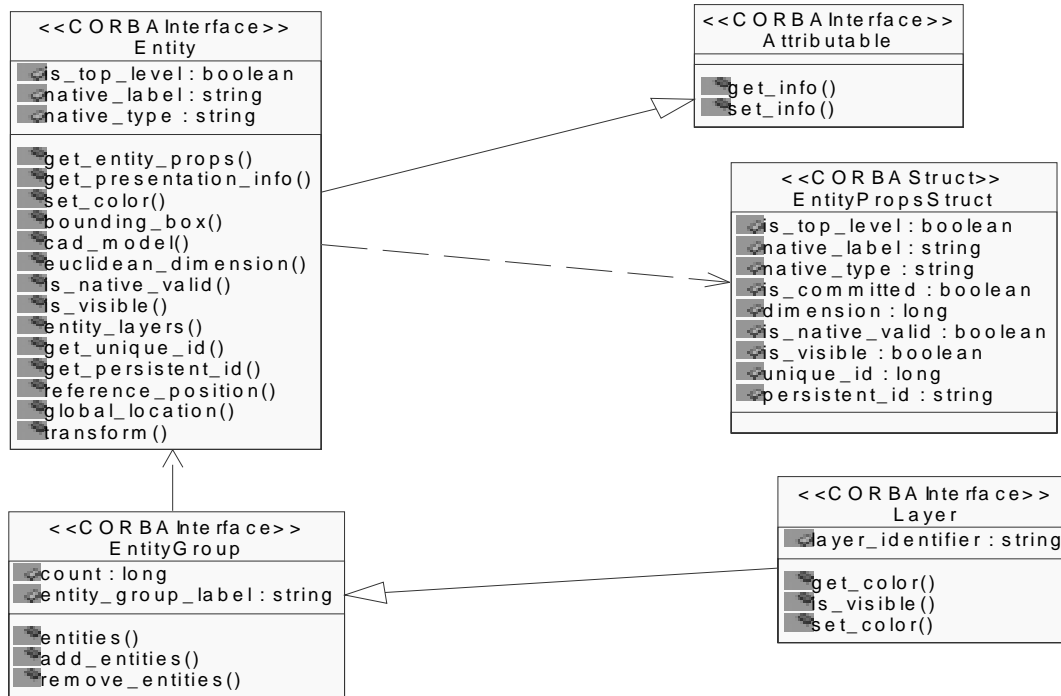
Figure 2-3 UML Diagram of CadFoundation Module
