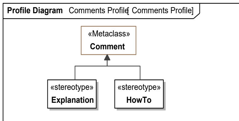
Figure 6: Comments Profile
