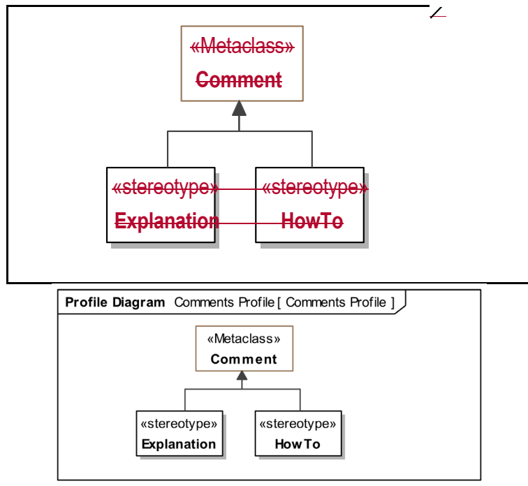
Figure 6-6: Comments Profile
