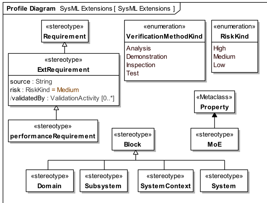
Figure 7-7: SysML Extensions
