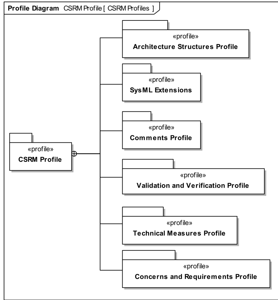
Figure 4-1: CSR Profiles
