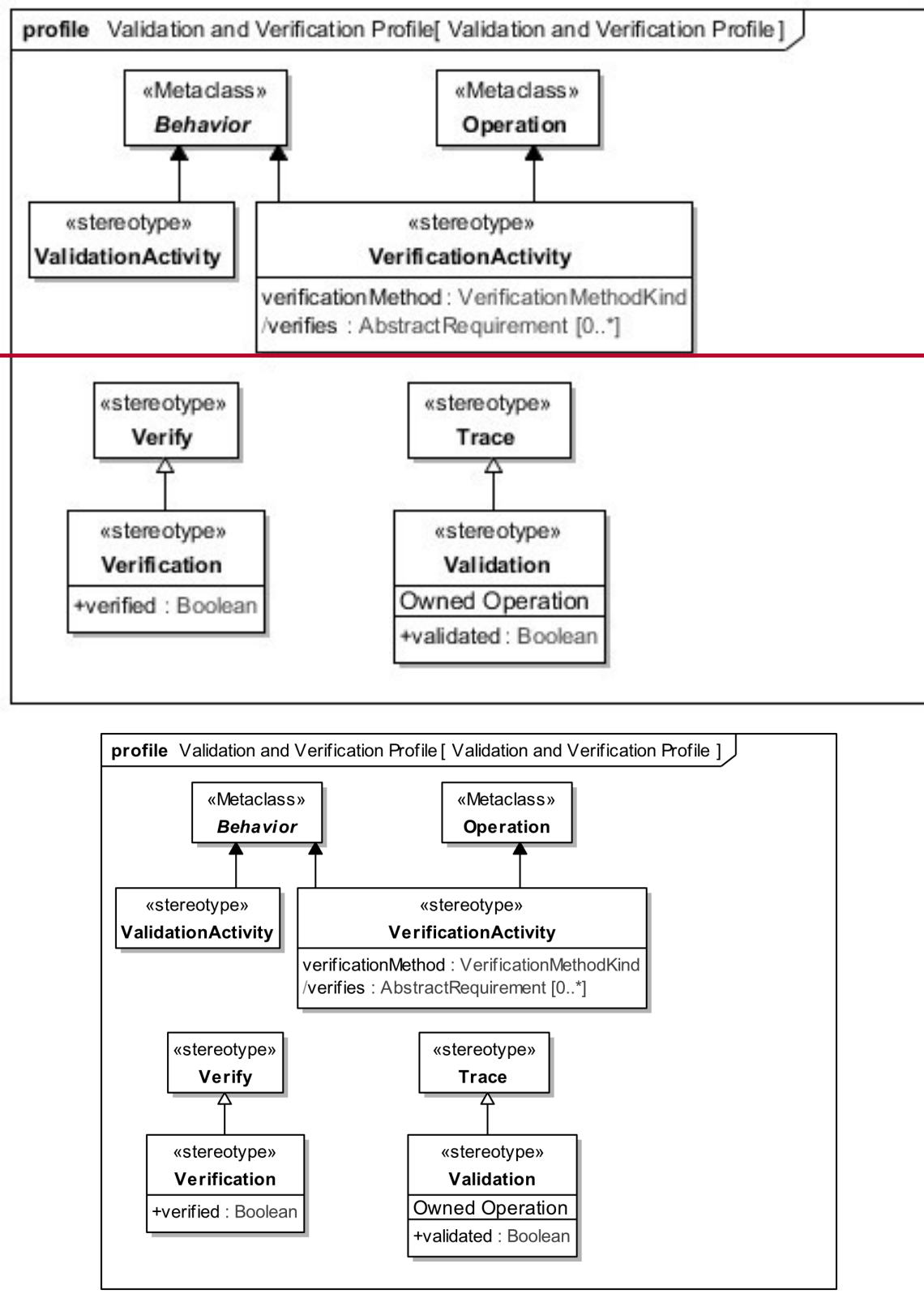
Figure 5-5: Validation and Verification Profile
