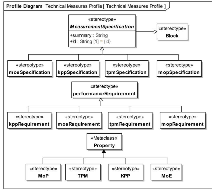
Figure 3-3: Technical Measures Profile
