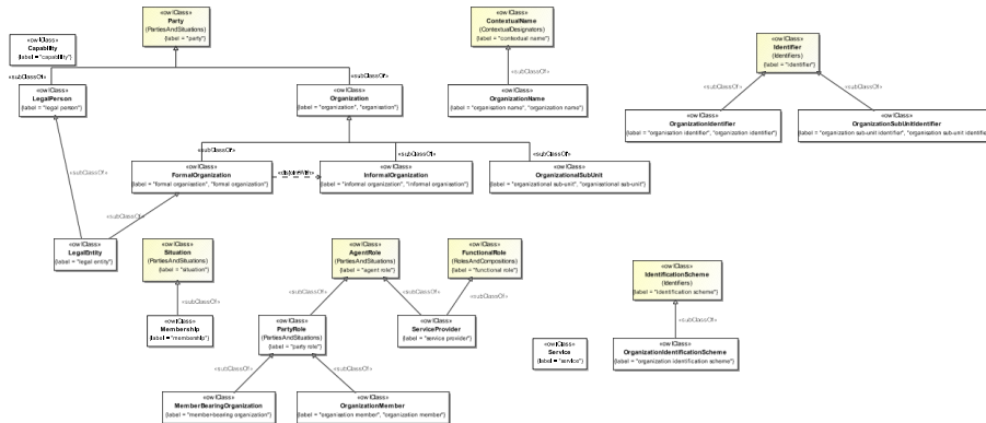
Figure 1416: Organizations Class Hierarchy
