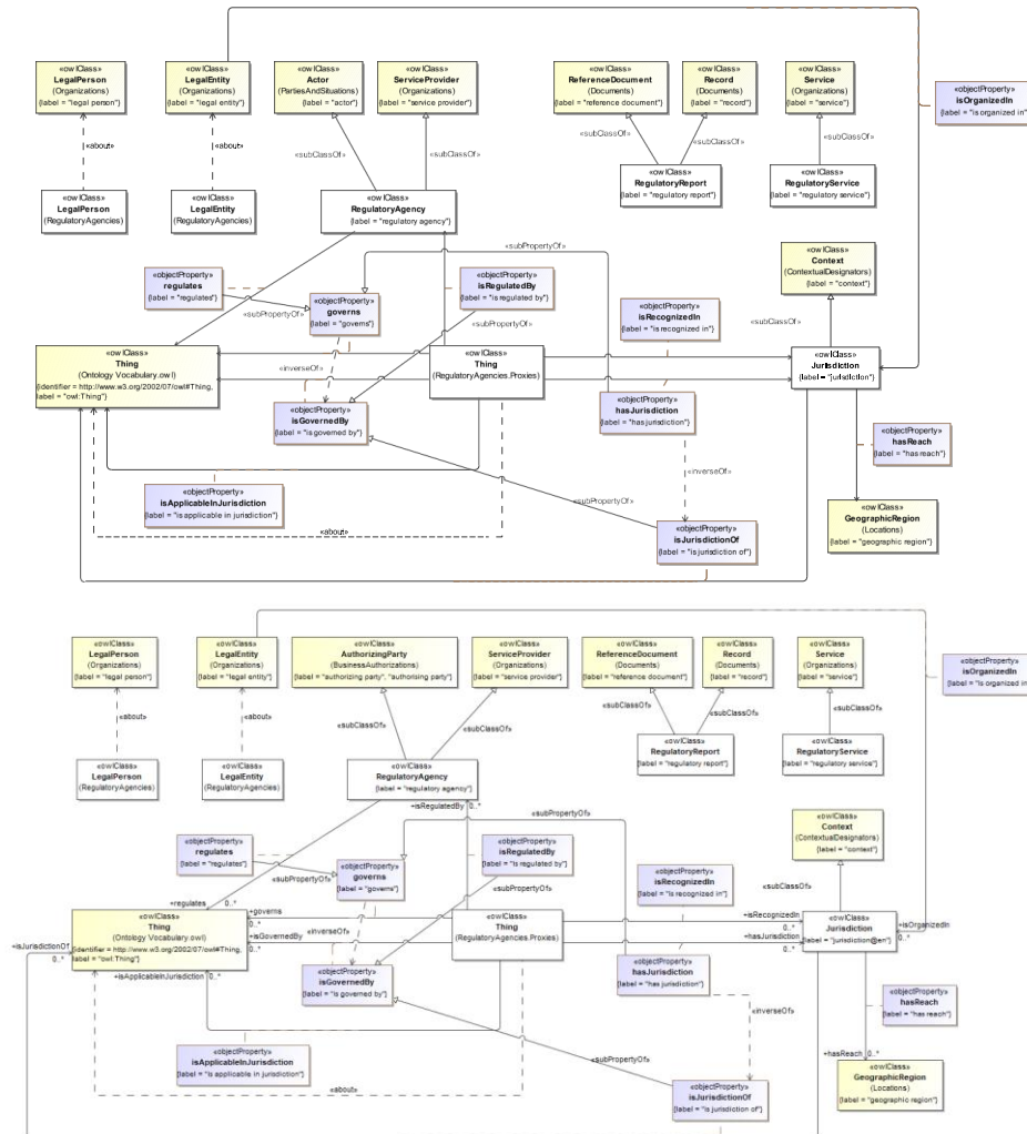
Figure 1820: Regulatory Agencies Ontology Overview
