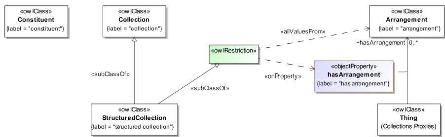
Figure 34: High-level Overview of the Collections Ontology
