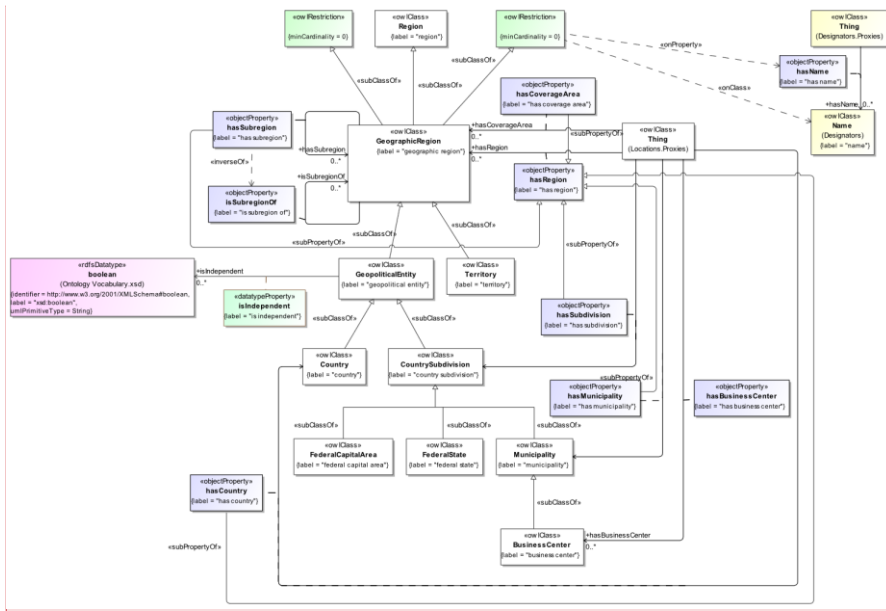
Figure 1214: Geographic Regions Overview
