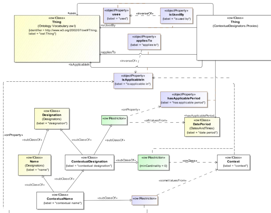
Figure 67: Overview of the Contextual Designations Ontology
