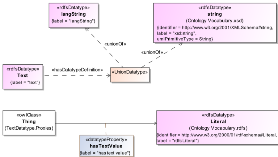
Figure 2424: Overview of the Text Datatype Ontology
