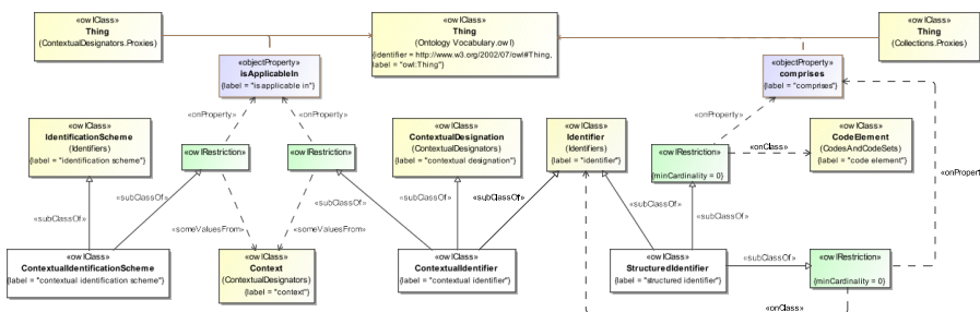
Figure 827: Overview of the Contextual Identifiers Ontology
