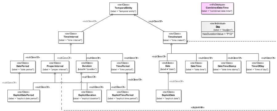
Figure 89: Class Hierarchy for the Dates and Times Ontology
