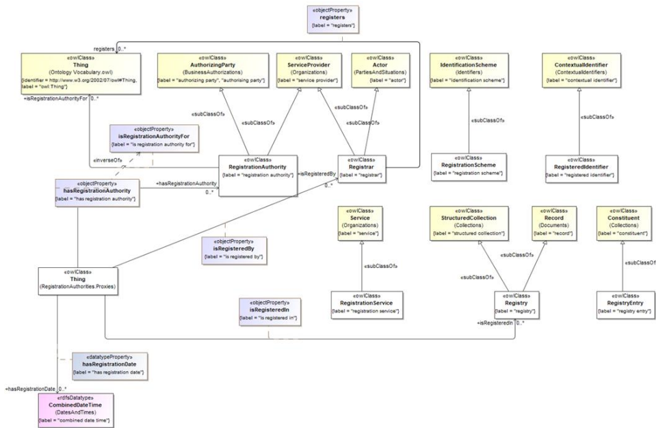
Figure 4719: Registration Authorities Ontology Overview
