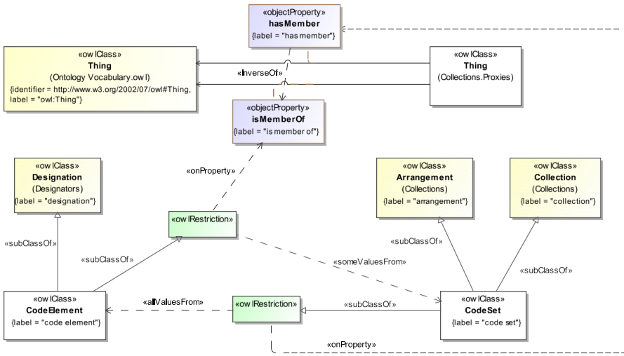
Figure 23: Overview of the Codes and Code Sets Ontology
