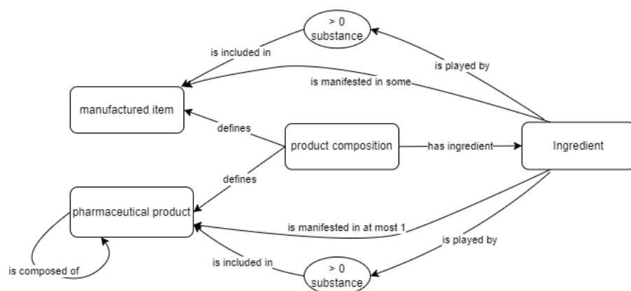
Figure 422: Example product composition
