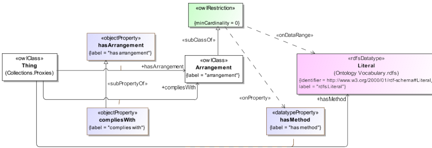
Figure 514: Expanded Arrangements Definitions
