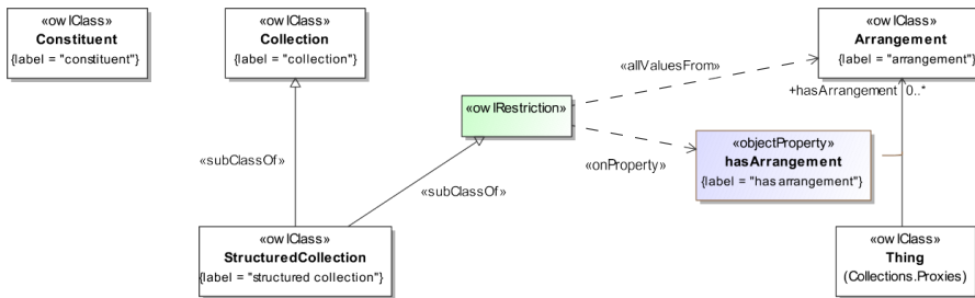
Figure 34: High-level Overview of the Collections Ontology
