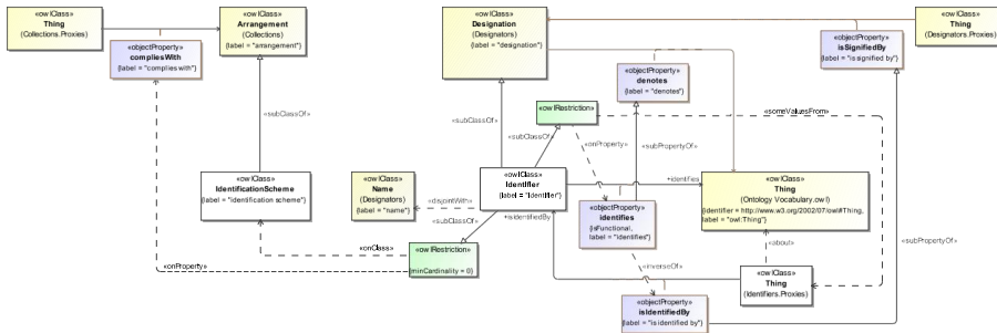
Figure 4412: Overview of the Identifiers Ontology
