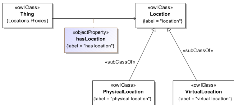
Figure 4315: Locations Class Hierarchy
