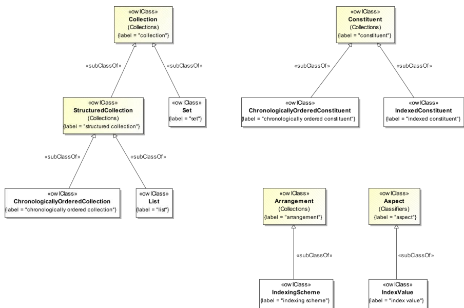
Figure 2023: Structured Collections Ontology Class Hierarchy
