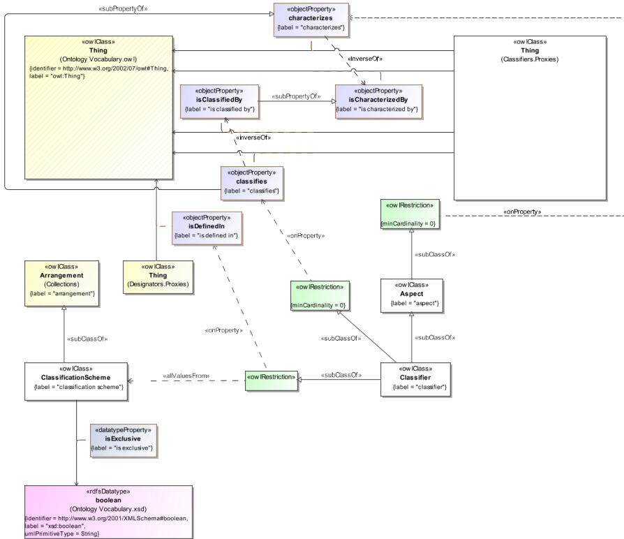
Figure 42: Overview of the Classifiers Ontology
