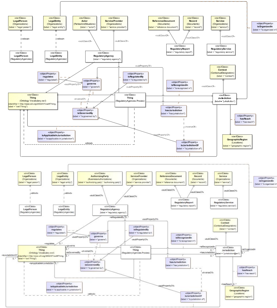
Figure 1820: Regulatory Agencies Ontology Overview
