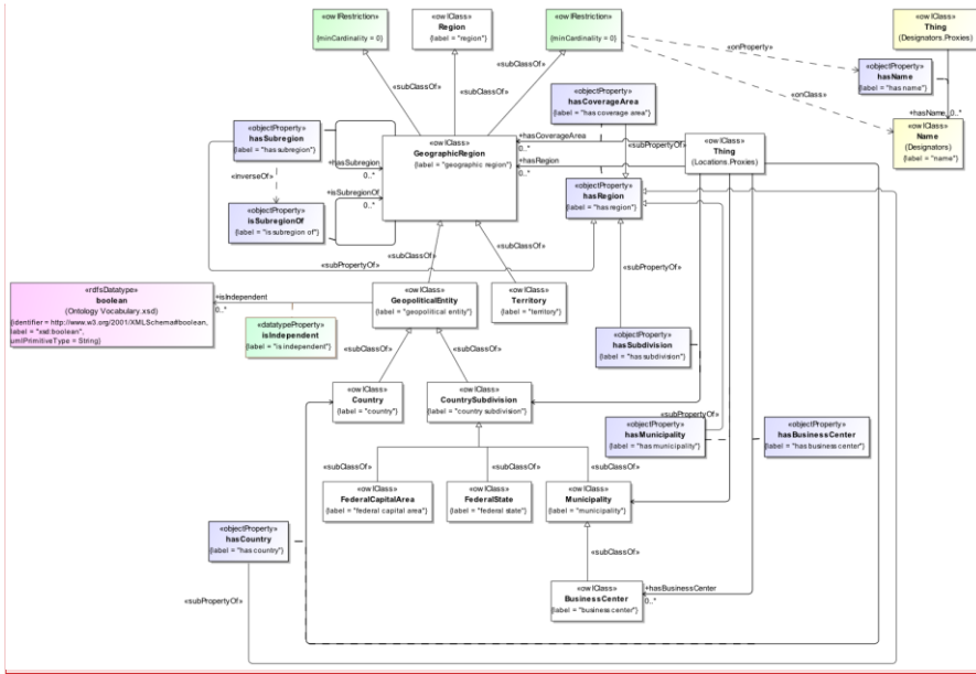
Figure 4214: Geographic Regions Overview
