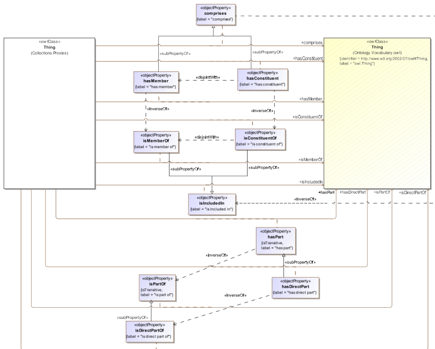
Figure 56: Mereological Relationships Defined in the Collections Ontology
