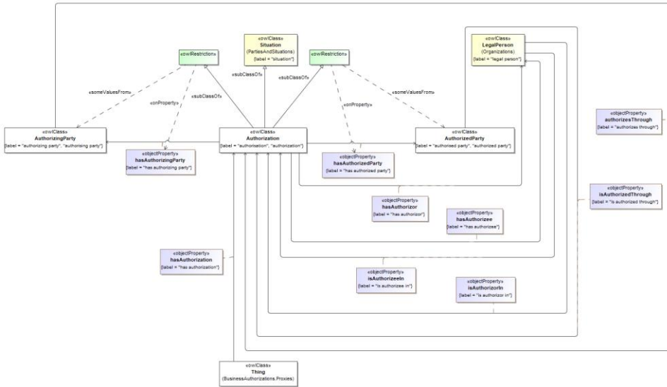
Figure 1: Business Authorizations Ontology Overview
