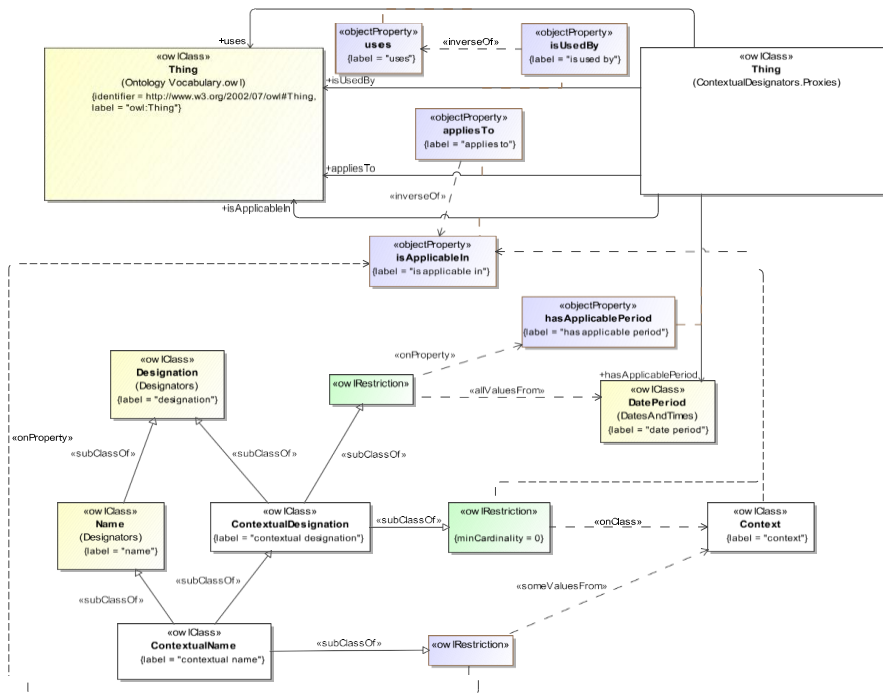
Figure 67: Overview of the Contextual Designators Ontology
