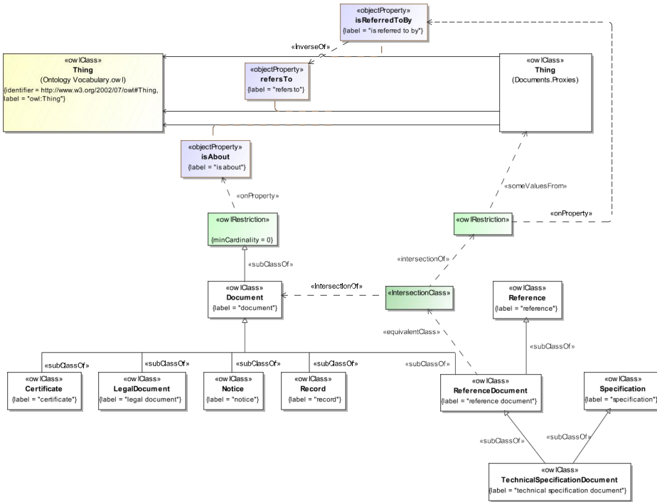
Figure 4911: Documents Ontology Overview
