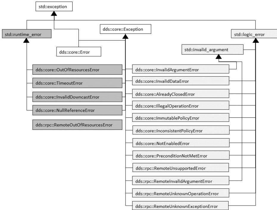
Figure 76: Inheritance Hierarchy of Local and Remote Exceptions
