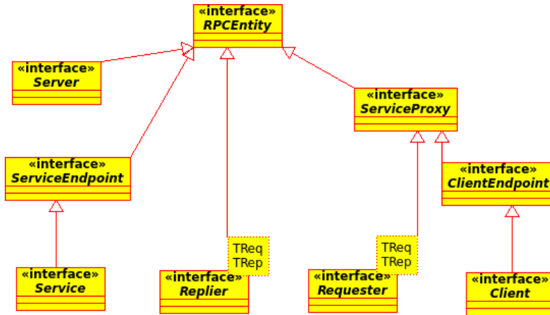
Figure 65: Inheritance Hierarchy of RPC Entities (TReq, TRep are type parameters)
