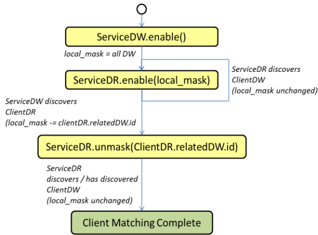
Figure 43: The service-side client matching algorithm
