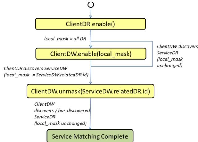
Figure 54: The client-side service matching algorithm
