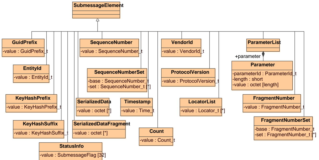
Figure 8.12 - RTPS SubmessageElements
