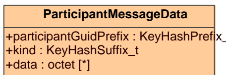
Figure 8.26 - ParticipantMessageData
