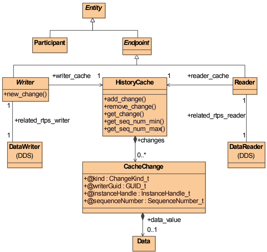
Figure 8.1 - RTPS Structure Module
