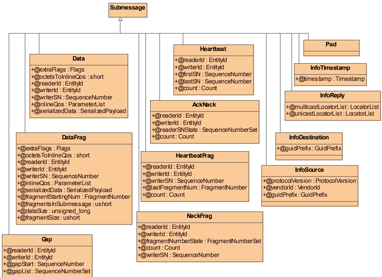
Figure 8.13 - RTPS Submessages
