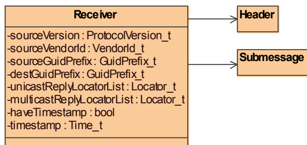
Figure 8.11 - RTPS Receiver
