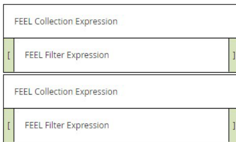
Figure 10-18: Filter expression
