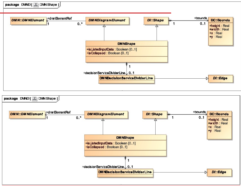
Figure 13-4-4: DMNShape
