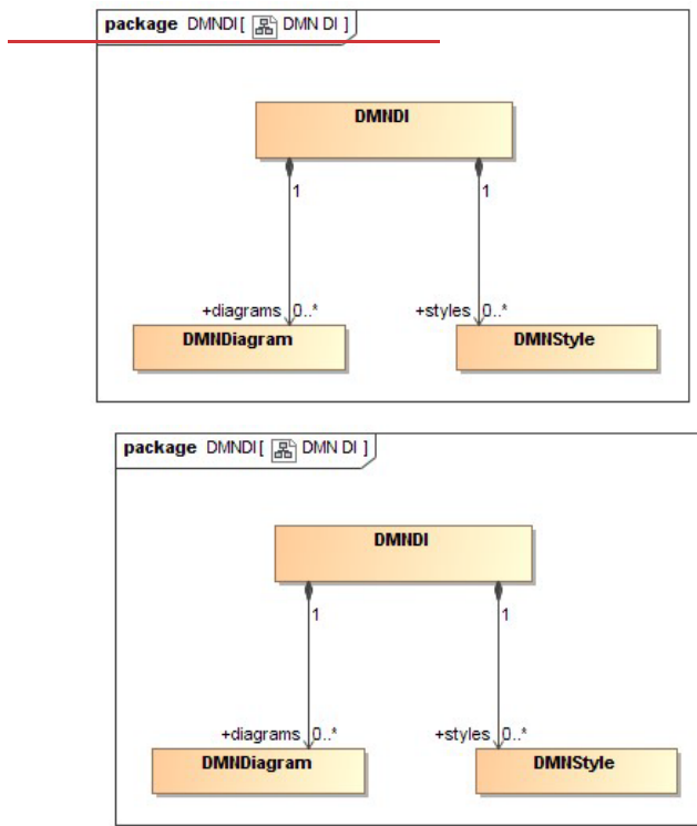
Figure 13-4-1: DMNDI
