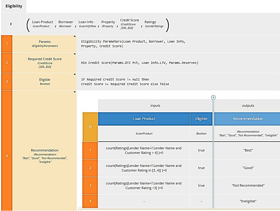
Figure 11-50-50: Eligibility (top)
