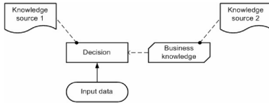
Figure 5-4: Knowledge sources
