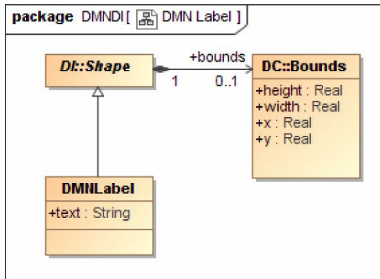
Figure 13-6-6: DMNLabel
