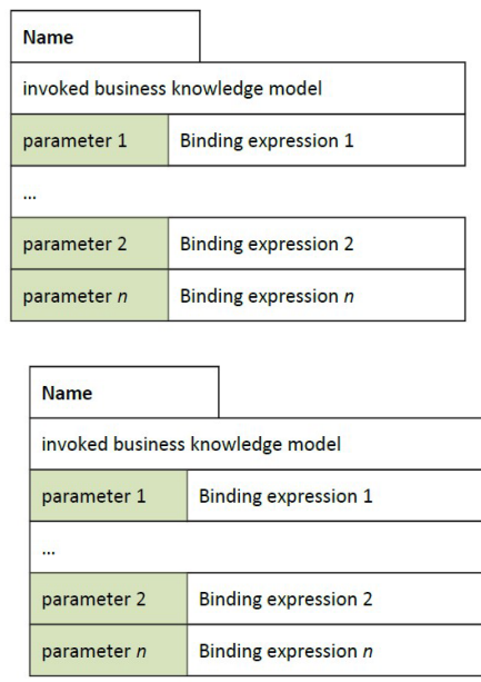
Figure 7-5-5: Boxed invocation
