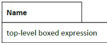
Figure 7-4-1: Boxed Expression
