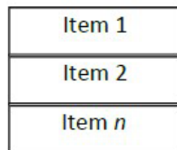
Figure 10-12: Vertical list
