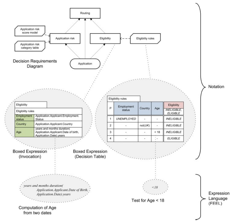
Figure 5-2-2: DMN Constructs
