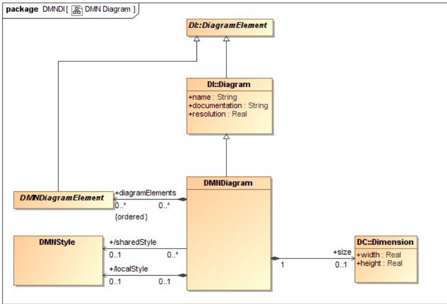
Figure 13-2--2: DMNDiagram
