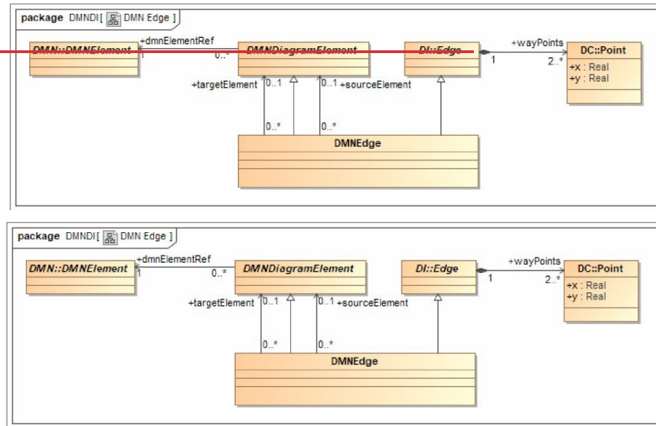
Figure 13-5-5: DMNEdge
