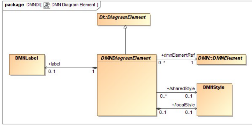
Figure 13-3-3: DMNDiagramElement
