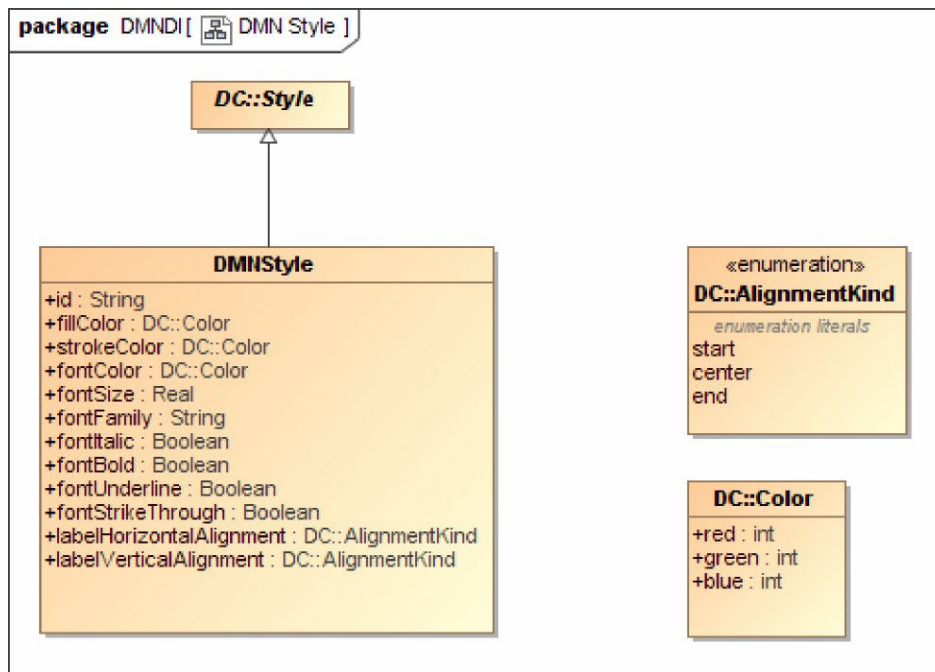
Figure 13-7-7: DMNStyle
