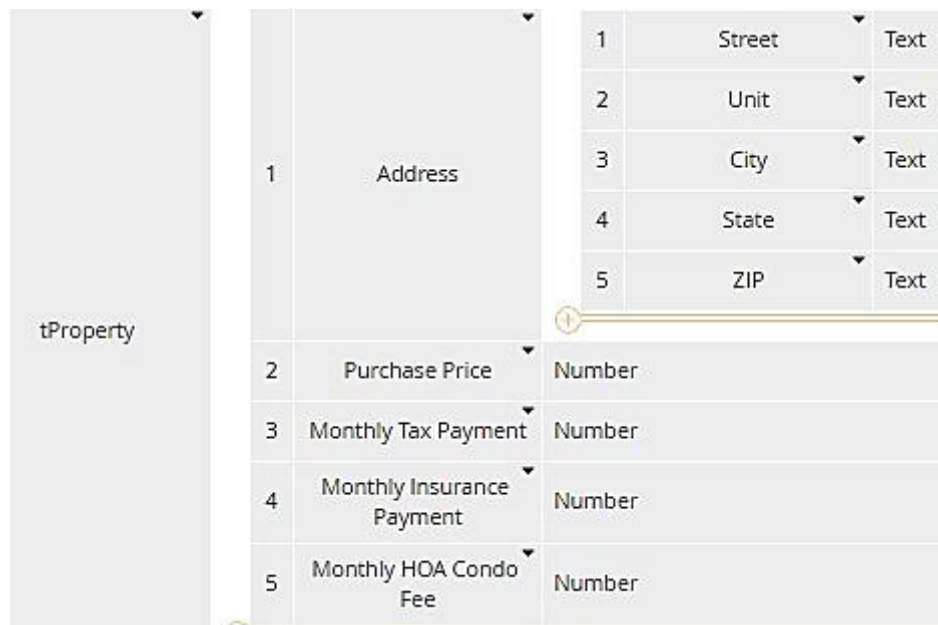
Figure 12-35: Type tProperty (non-normative representation)
