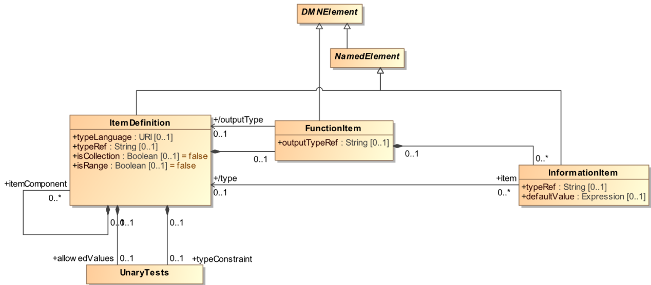
Figure 7-7: ItemDefinition class diagram
