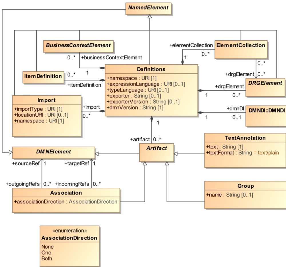
Figure 6-12: Definitions Class Diagram
