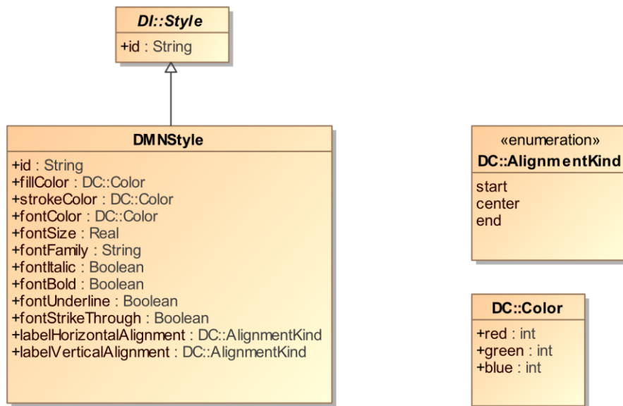
Figure 14-7: DMNStyle
