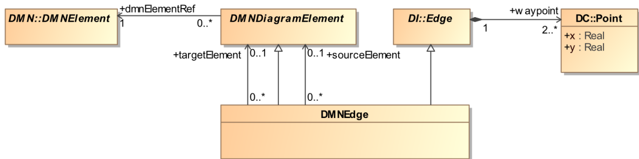
Figure 14-5: DMNEdge
