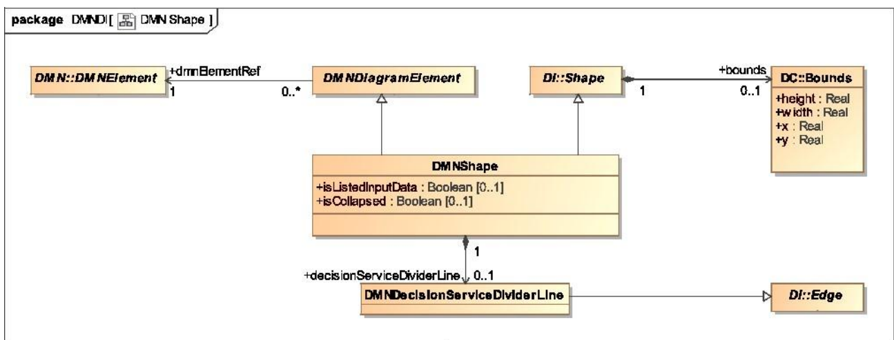
Figure 14-4: DMNShape
