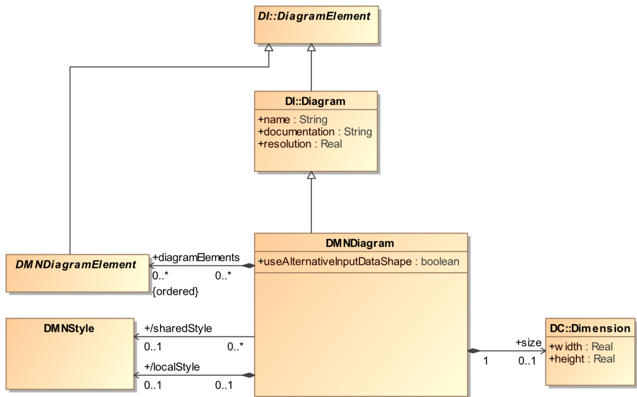
Figure 14-2: DMNDiagram
