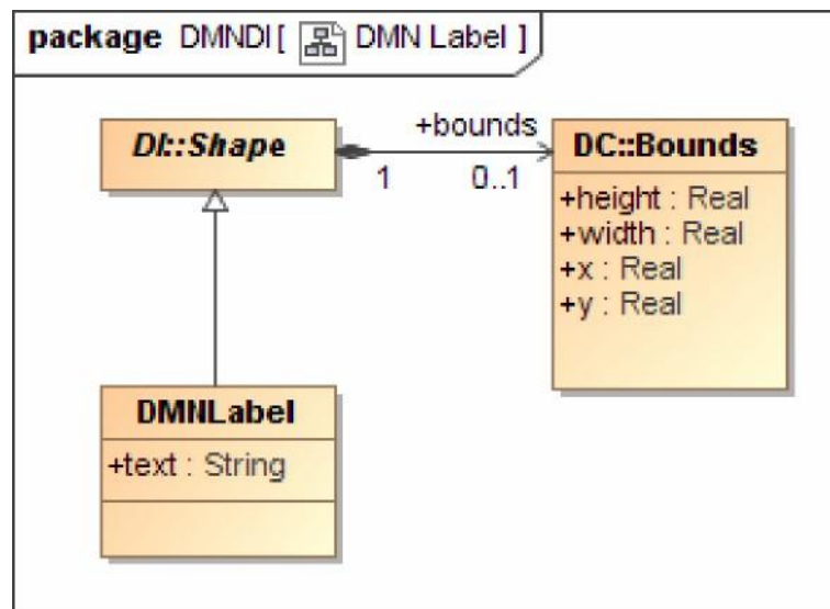
Figure 14-6: DMNLabel
