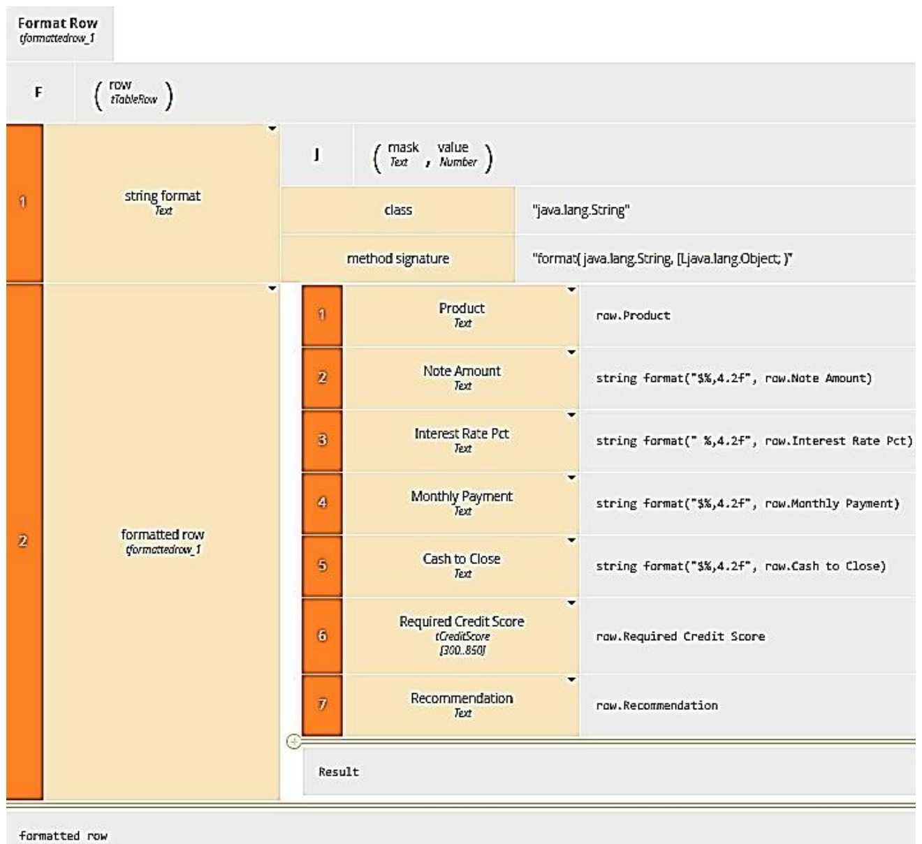
Figure 12-54: Format Row
