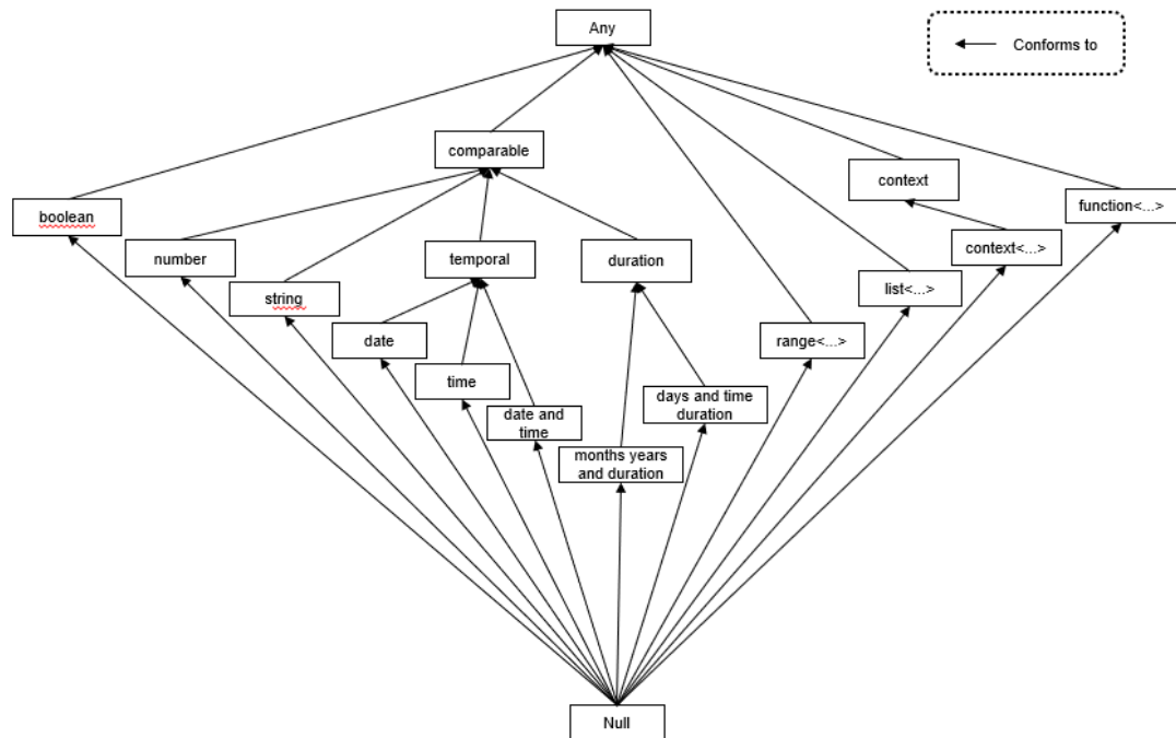
Figure 10-26: FEEL type lattice
