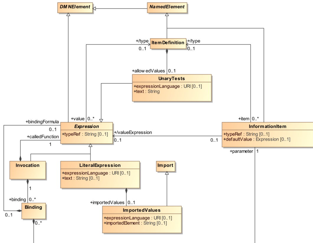
Figure 7-6: Expression class diagram
