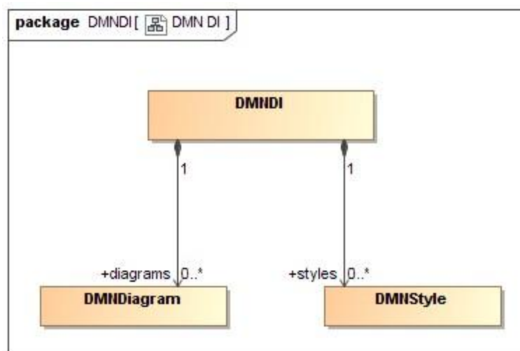
Figure 14-1: DMNDI
