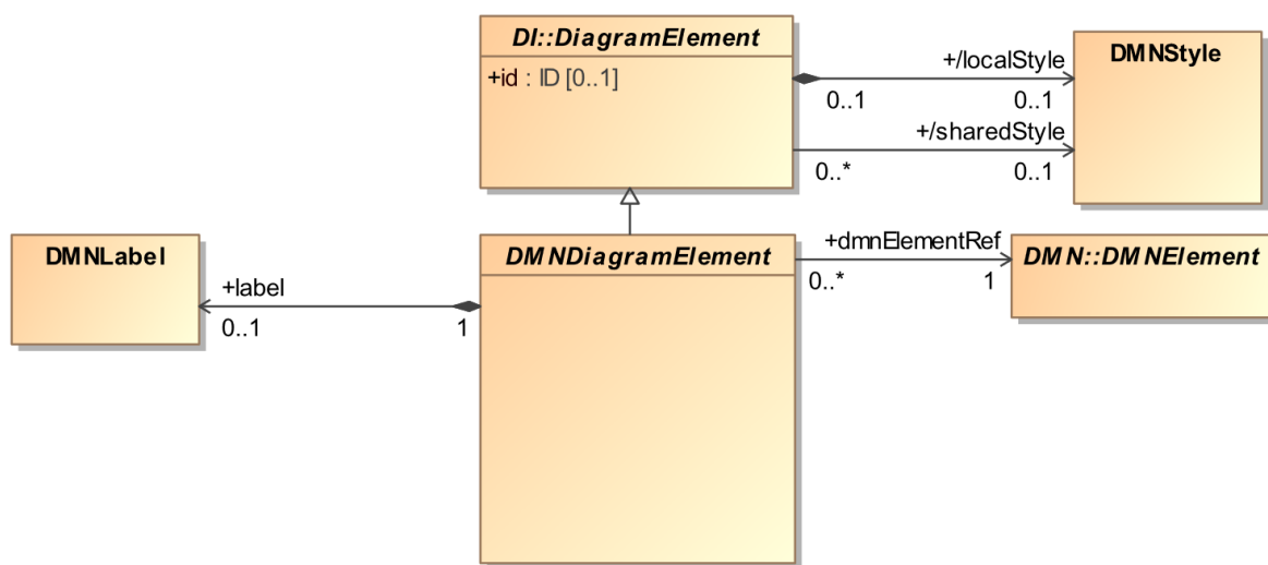
Figure 14-3: DMNDiagramElement
