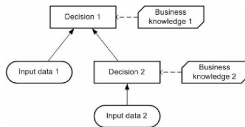
Figure 5-5: A simple Decision Requirements Diagram (DRD)
