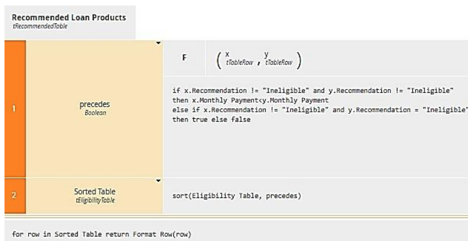
Figure 12-53: Recommended Loan Products
