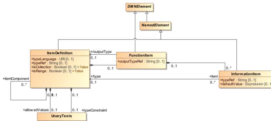
Figure 7-7: ItemDefinition class diagram
