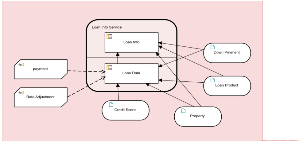
Figure 12-41: DRD of imported Loan Info Service
