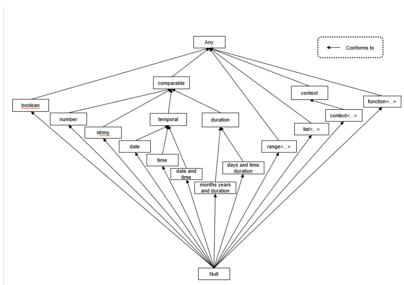
Figure 10-26: FEEL type lattice type
