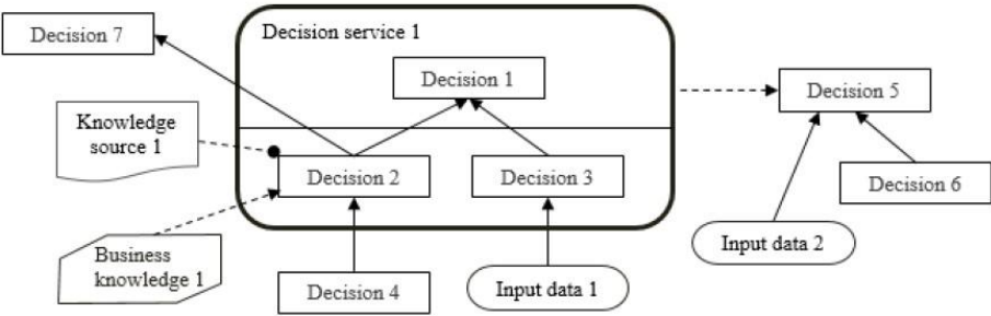
Figure 6-9: A decision service defined as an overlay
