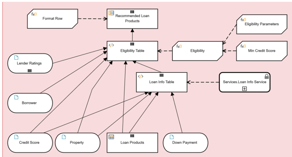
Figure 12-34: DRD for Recommended Loan Products
