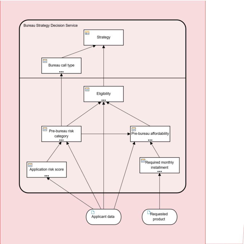
Figure 12-7: Bureau Strategy Decision Service
