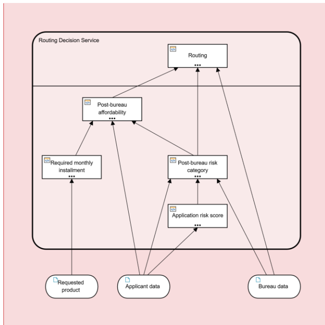
Figure 12-8: Routing Decision Service
