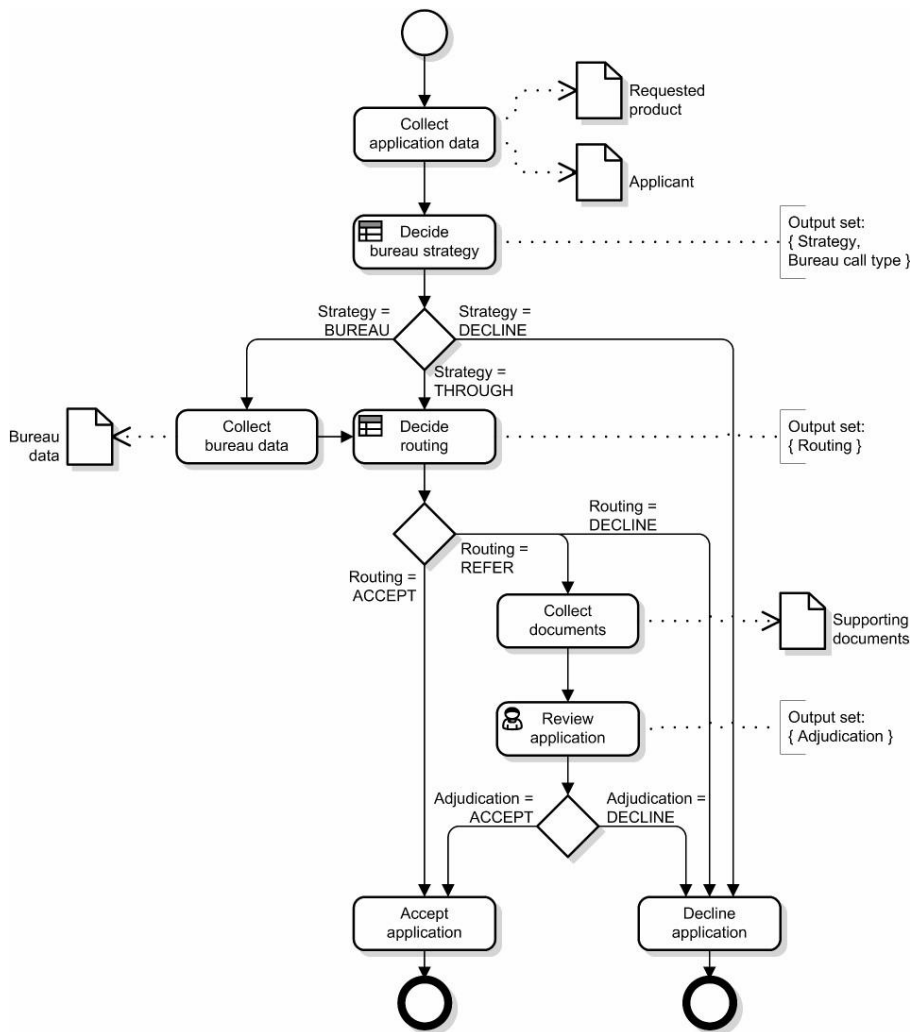
Figure 12-1: Example business process
