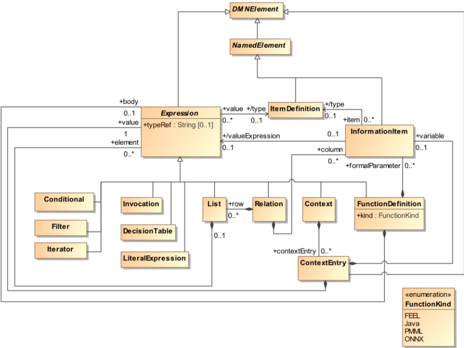
Figure 10-27: Expression class diagram
