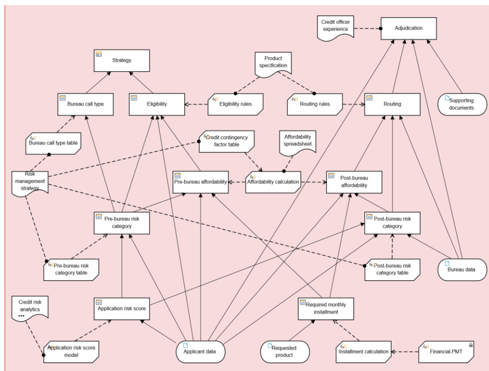
Figure 12-2: DRD of all automated decision-making
