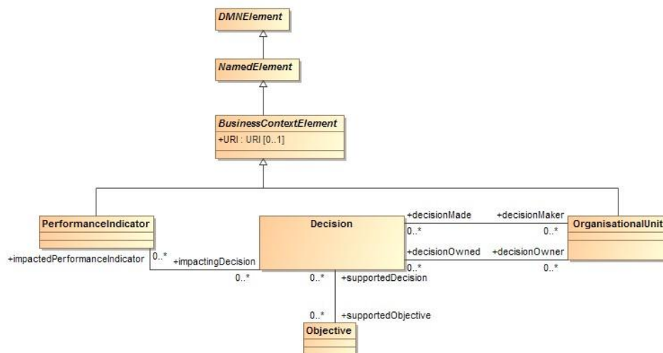
Figure 6-14: BusinessContextElement class diagram
