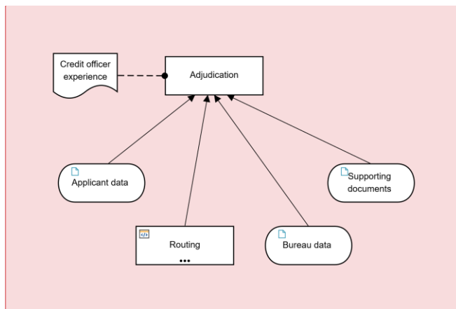
Figure 12-5: DRD for Review application decision point
