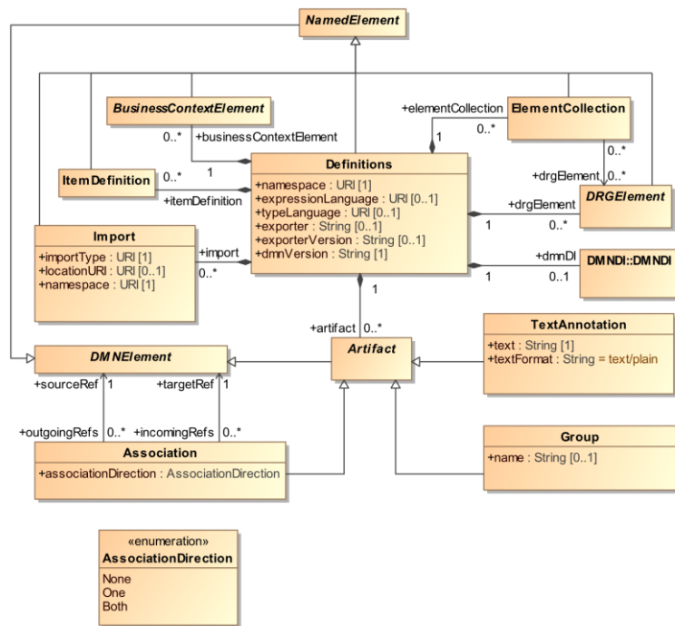
Figure 6-12: Definitions Class Diagram
