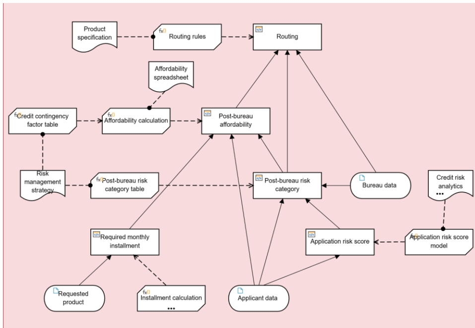
Figure 12-4: DRD for Decide routing decision point
