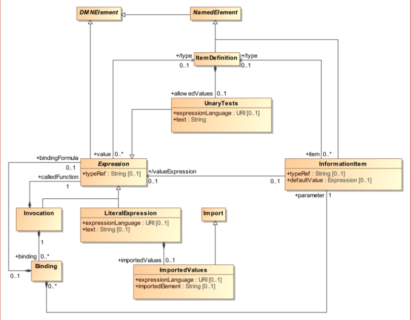
Figure 7-6: Expression class diagram
