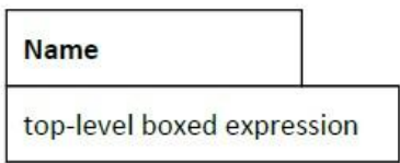
Figure 7-1: Boxed Expression
