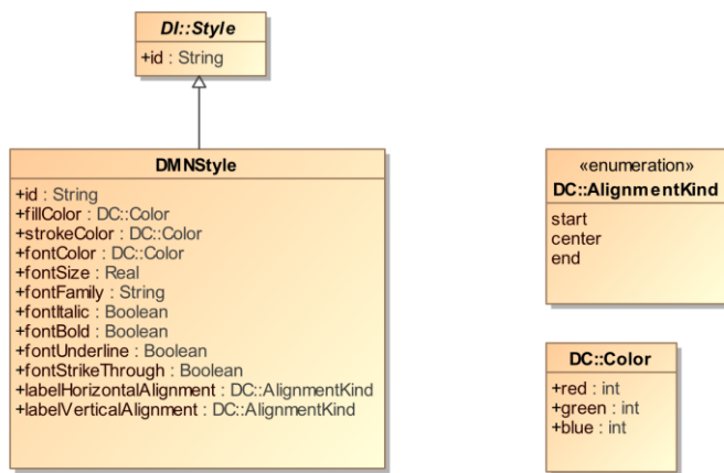
Figure 14-7: DMNStyle
