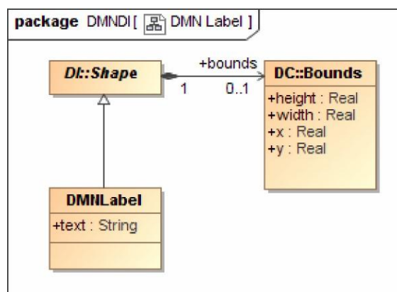
Figure 14-6: DMNLabel
