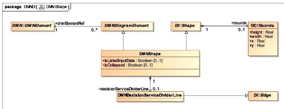
Figure 14-4: DMNShape
