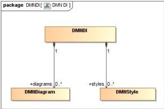
Figure 14-1: DMNDI
