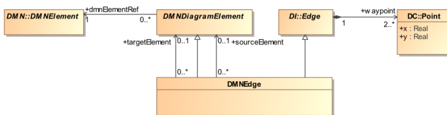
Figure 14-5: DMNEdge
