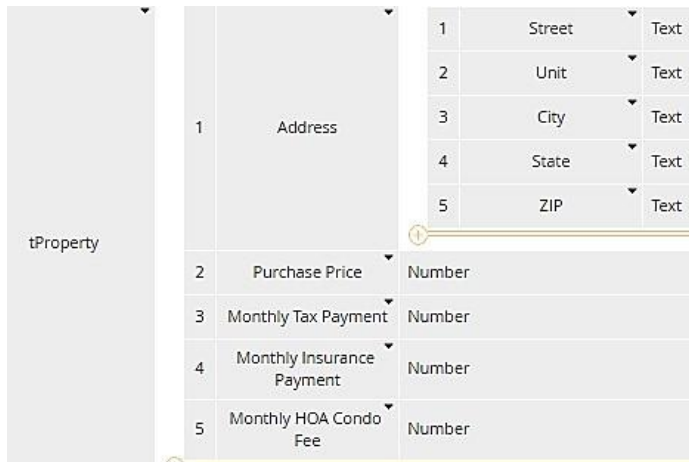
Figure 12-35: Type tProperty (non-normative representation)
