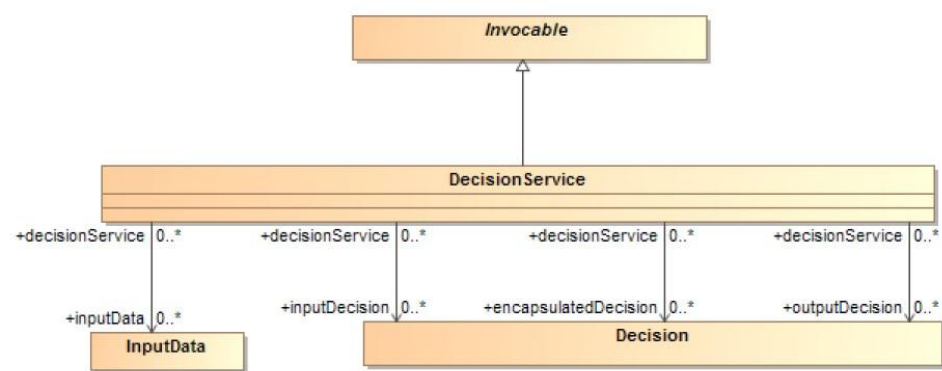
Figure 6-16: DecisionService class diagram
