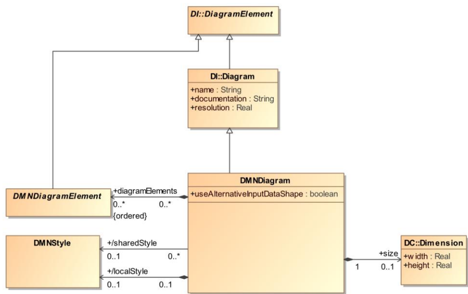
Figure 14-2: DMNDiagram
