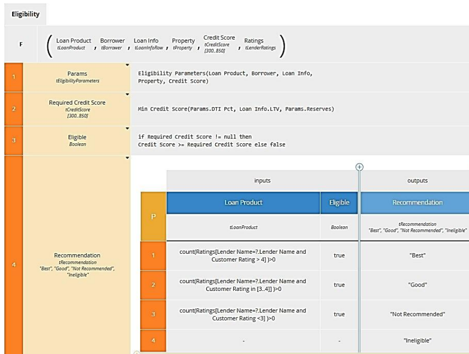
Figure 12-50: Eligibility (top)
