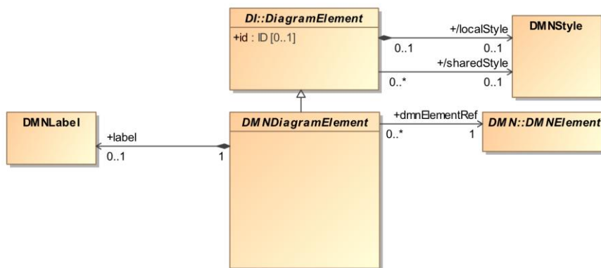
Figure 14-3: DMNDiagramElement
