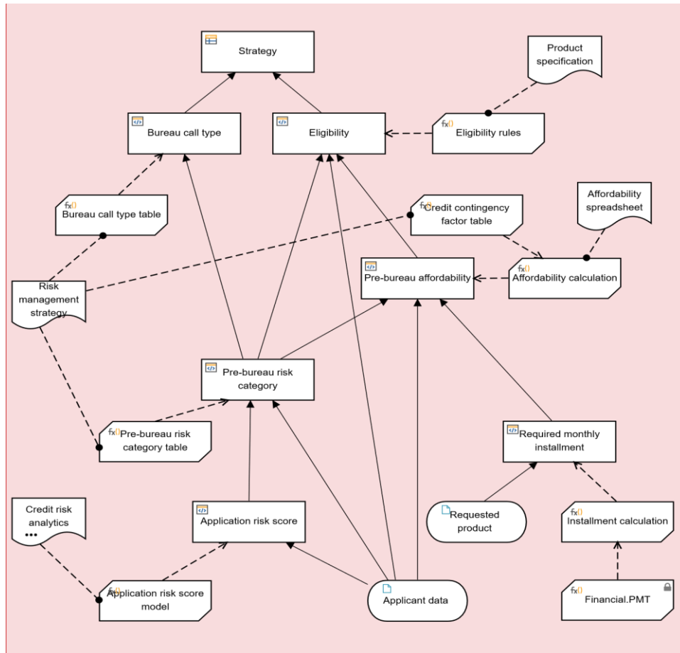
Figure 12-3: DRD for Decide bureau strategy decision point
