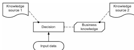
Figure 5-4: Knowledge sources
