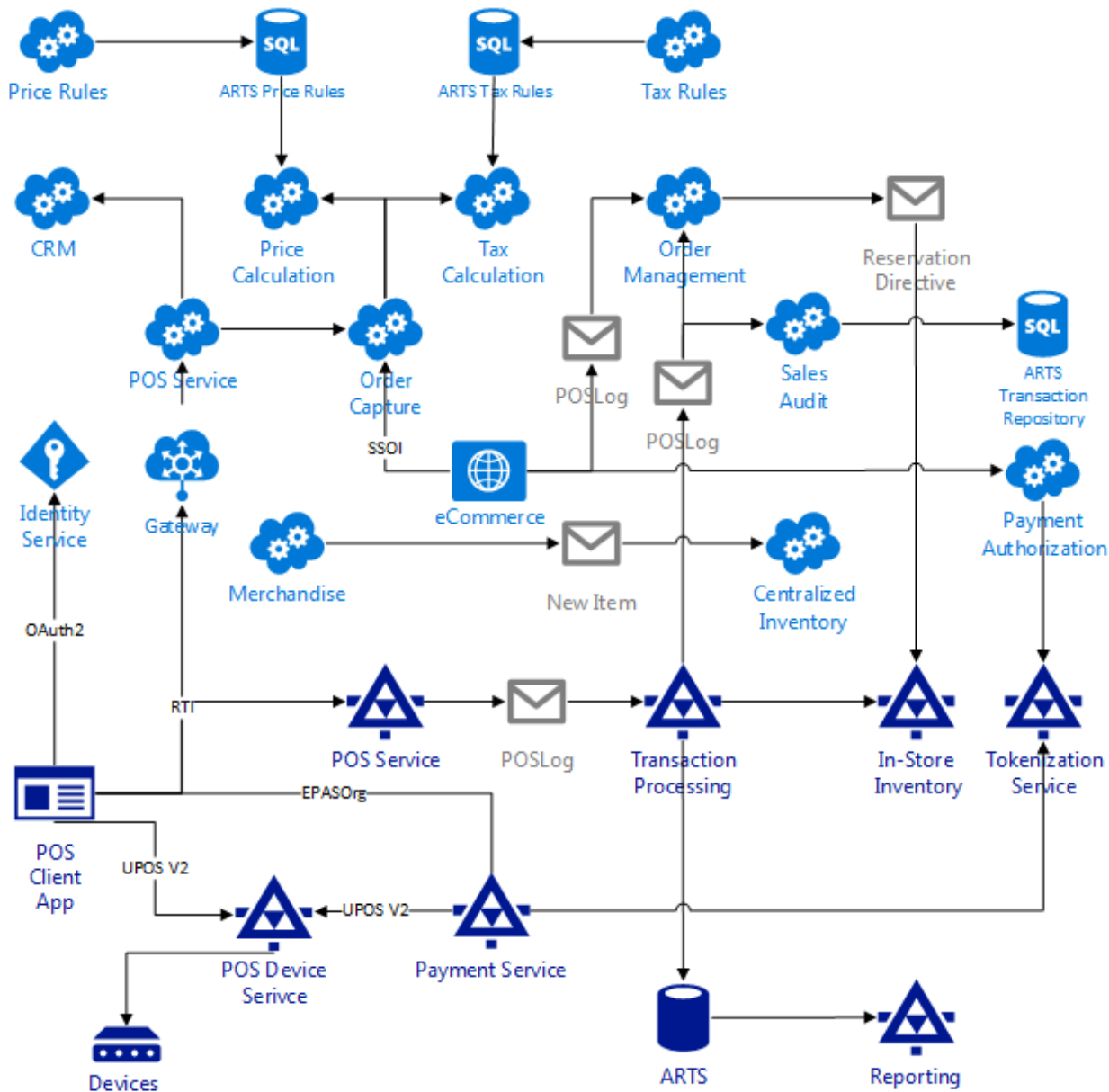
Figure 6.11 Shared Database in Cloud
