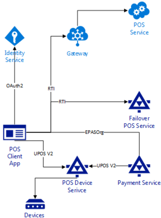
Figure 6.3 RPC from Store to Cloud
