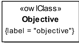
Figure 10.19 - Objectives Concepts
