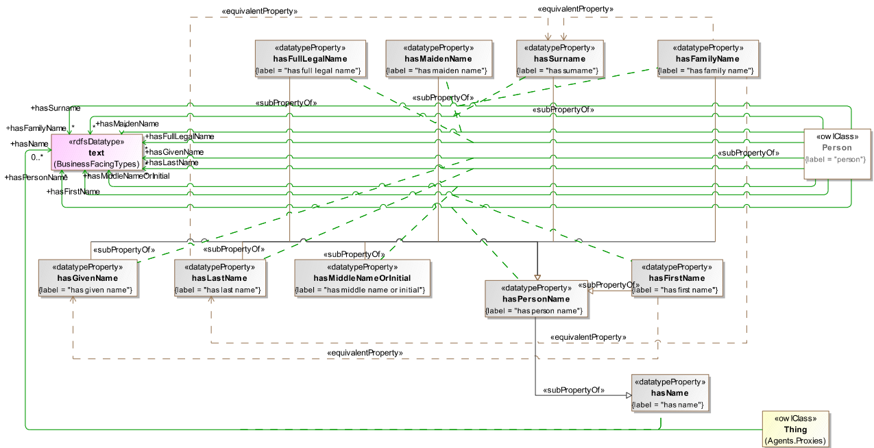
Figure 10.33 - People Names
