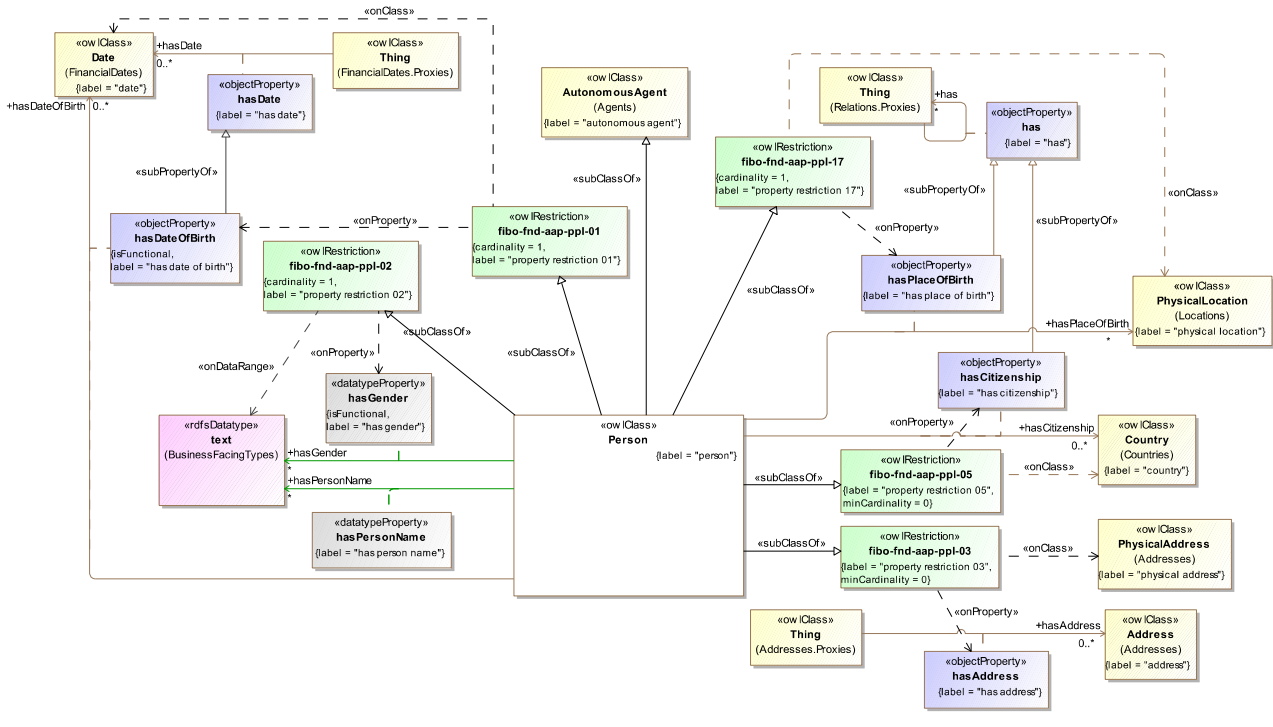
Figure 10.31 - Person Fundamentals
