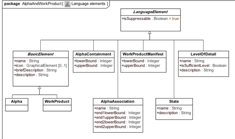
Figure 9.8 – AlphaAndWorkProduct::Language elements
