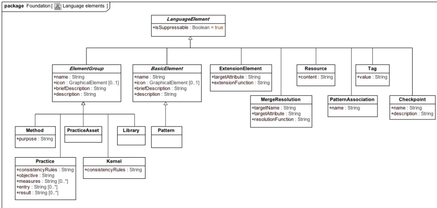
Figure 9.5 – Foundation::Language elements
