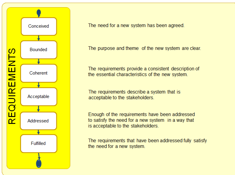
Figure 8.7 – The states of the Requirements
