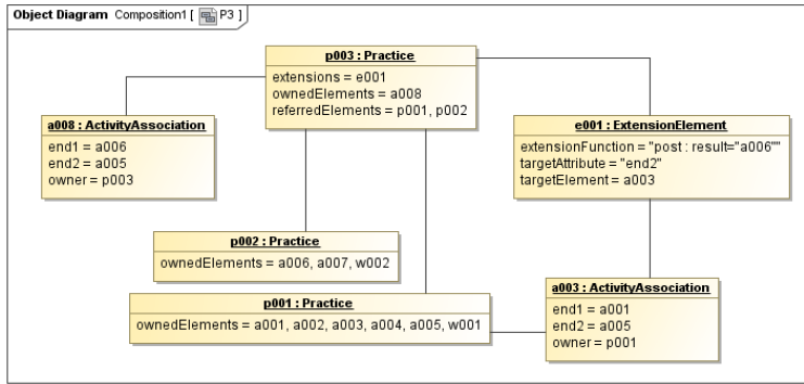
Figure 9.19 – Partial object diagram for P3
