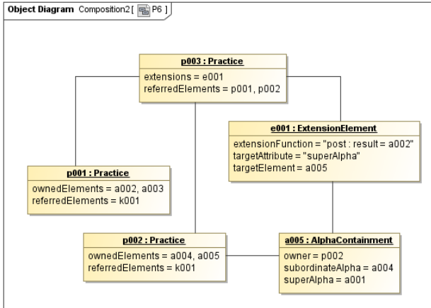
Figure 9.21 – Partial object diagrams for P6
