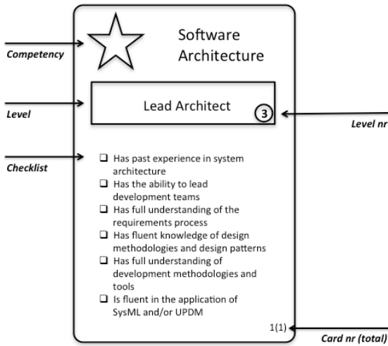
Figure 87 – Software Architect Lead Architect Detail Card
