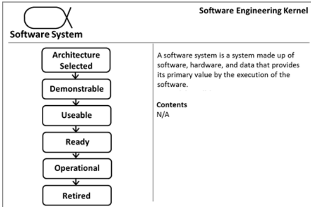
Figure 9.38 – Software System Alpha Definition Card
