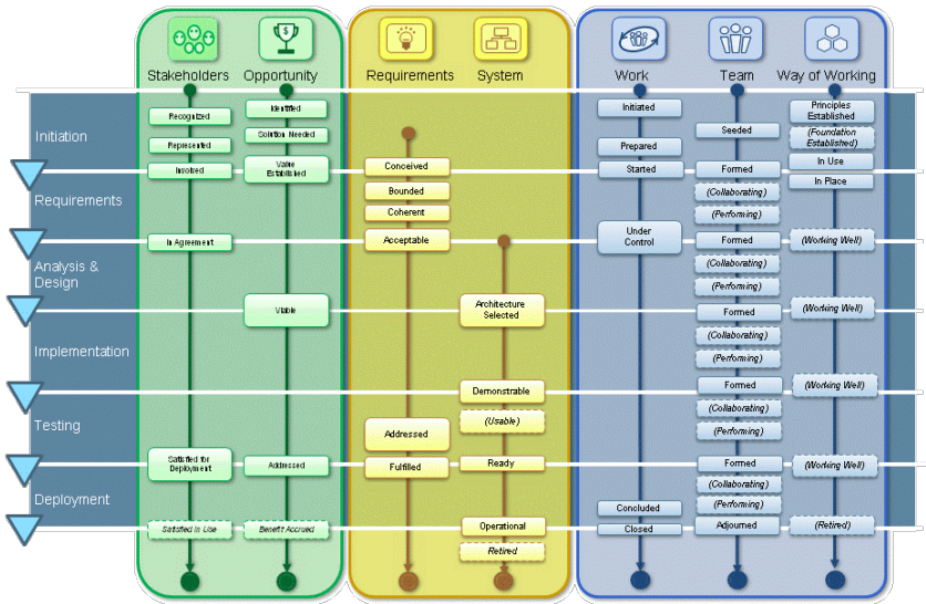
Figure E.27 – A Waterfall lifecycle
