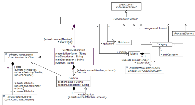
Figure C.1 – SPEM Describable Element parts and subclasses
