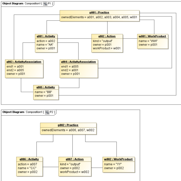
Figure 9.18 – Object diagrams for P1 and P2
