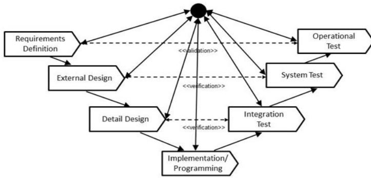
Figure E.19 – Multi-phase Waterfall Practice Activities Flow
