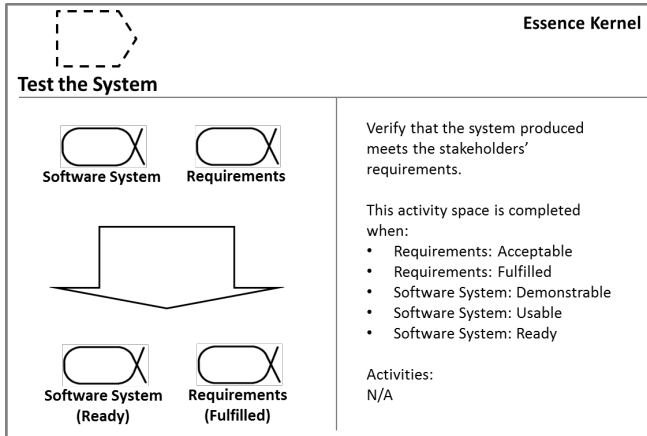
Figure 9.74 – Test the System Activity Space definition card
