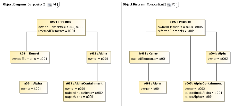
Figure 9.20 – Object diagrams for P4 and P5
