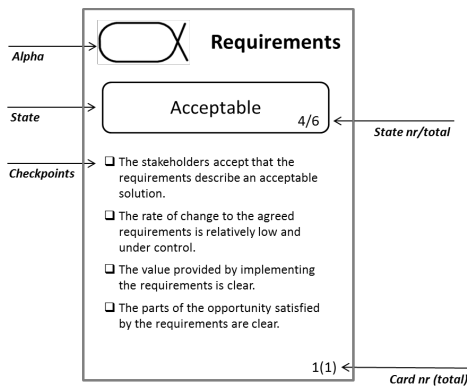
Figure 9.40 – Software System Alpha Definition Card
