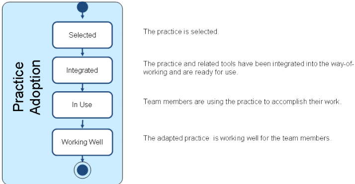
Figure A.15 – The states of Practice Adoption
