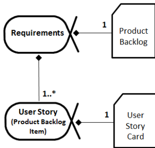
Figure E.35 – Scrum with User Story
