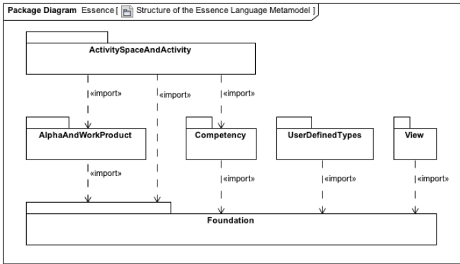
Figure 9.3 – Structure of the Essence Language metamodel
