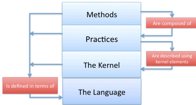
Figure 7.1 – Method architecture
