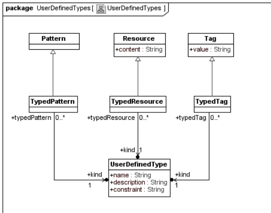
Figure 9.14 – UserDefinedTypes::UserDefinedTypes
