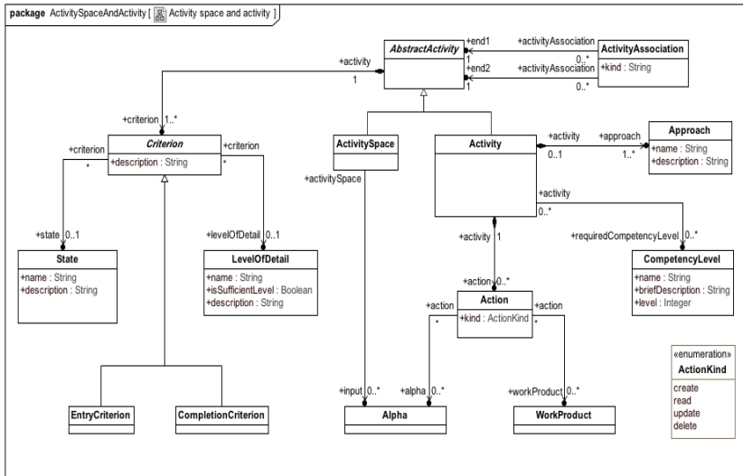
Figure 9.11 – ActivitySpaceAndActivity::Activity space and activity
