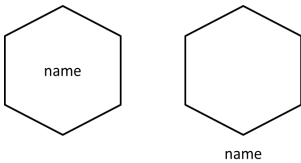
Figure 9.52 – Practice symbol
