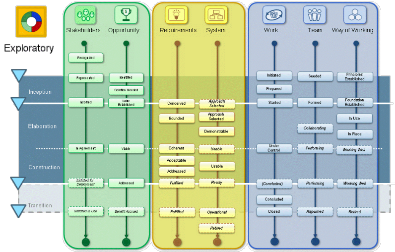
Figure E.30 – The Exploratory lifecycle
