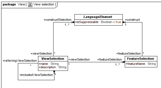
Figure 9.16 – View::View selection
