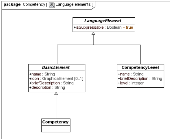
Figure 9.12 – Competency::Language elements
