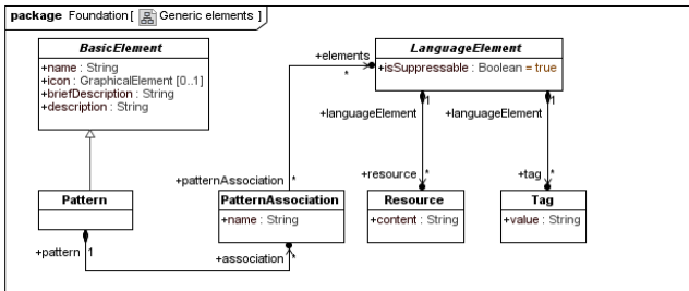
Figure 9.7 – Foundation::Generic elements
