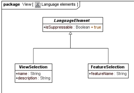
Figure 9.15 – View::Language elements
