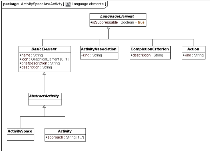
Figure 9.10 – ActivitySpaceAndActivity::Language elements
