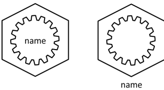
Figure 9.30 – Kernel symbol
