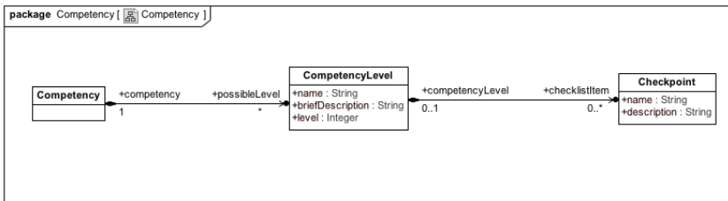
Figure 9.13 – Competency::Competency
