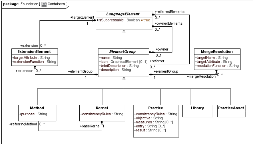
Figure 9.6 – Foundation::Containers
