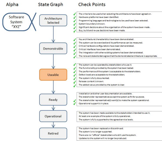
Figure 9.23 – Determination of State using Check Points
