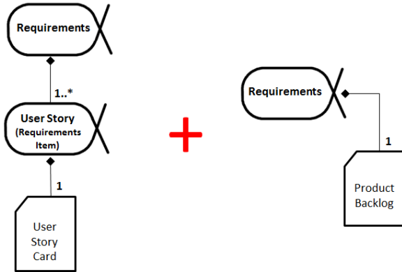
Figure E.34 – Merging User Story with Scrum
