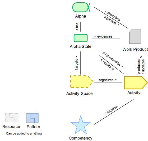
Figure 9.1 – Conceptual Overview of the Language
