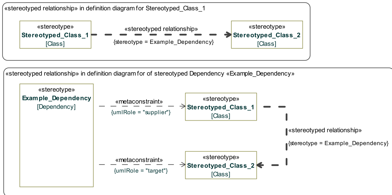
Figure 6-4 Uses of «stereotyped relationship» dependency
