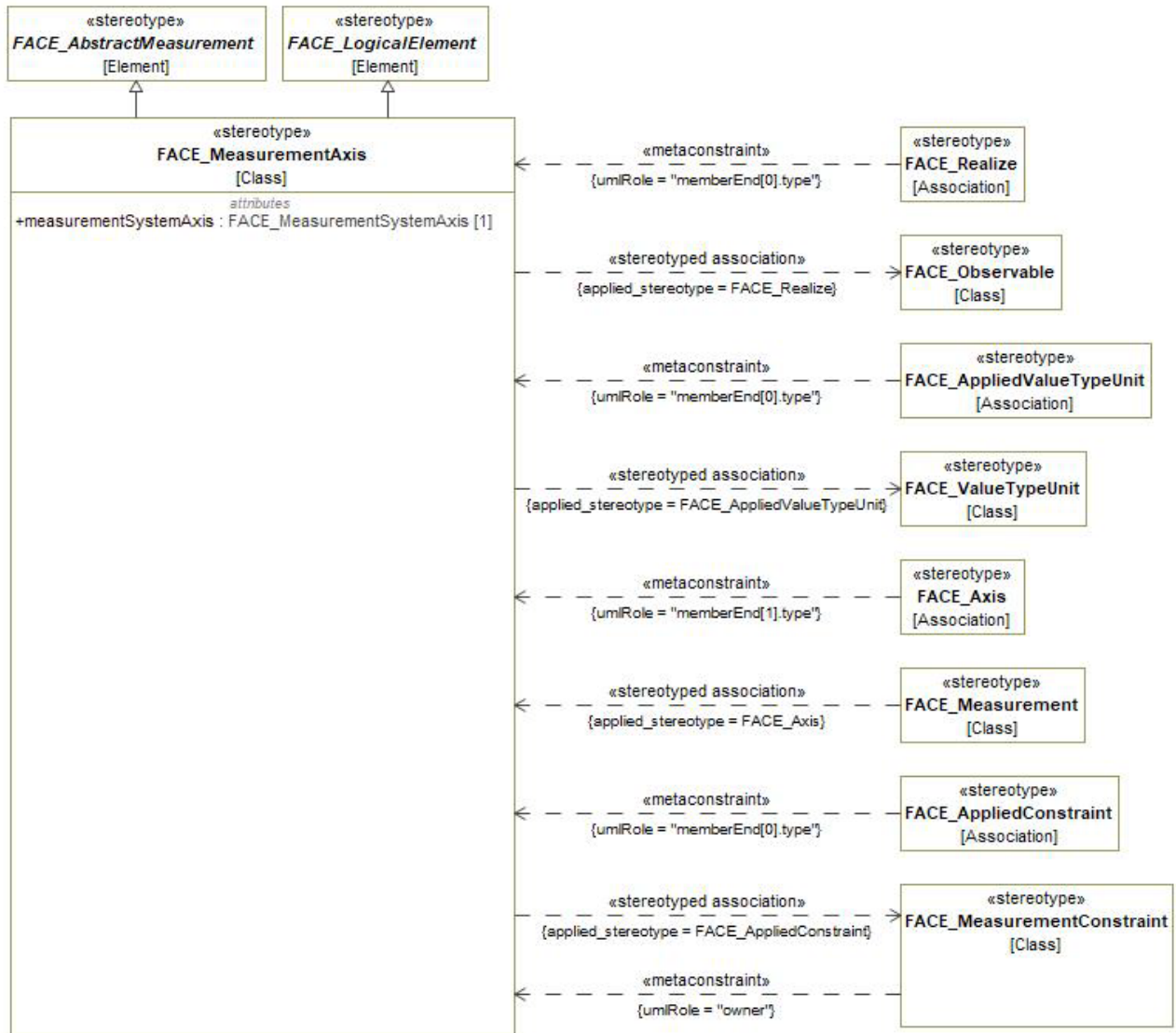
Figure 7-68: FACE_MeasurementAxis
