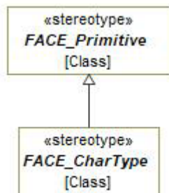
Figure 7-90: abstract FACE_CharType
