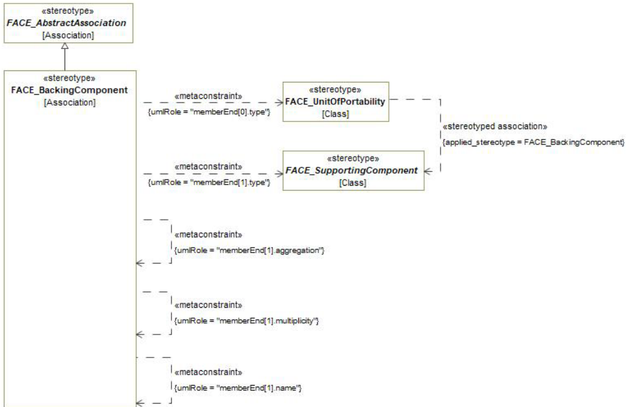
Figure 7-163: FACE_BackingComponent
