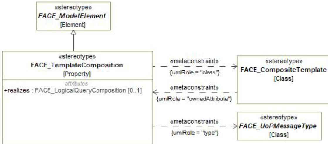
Figure 7-189: FACE_TemplateComposition
