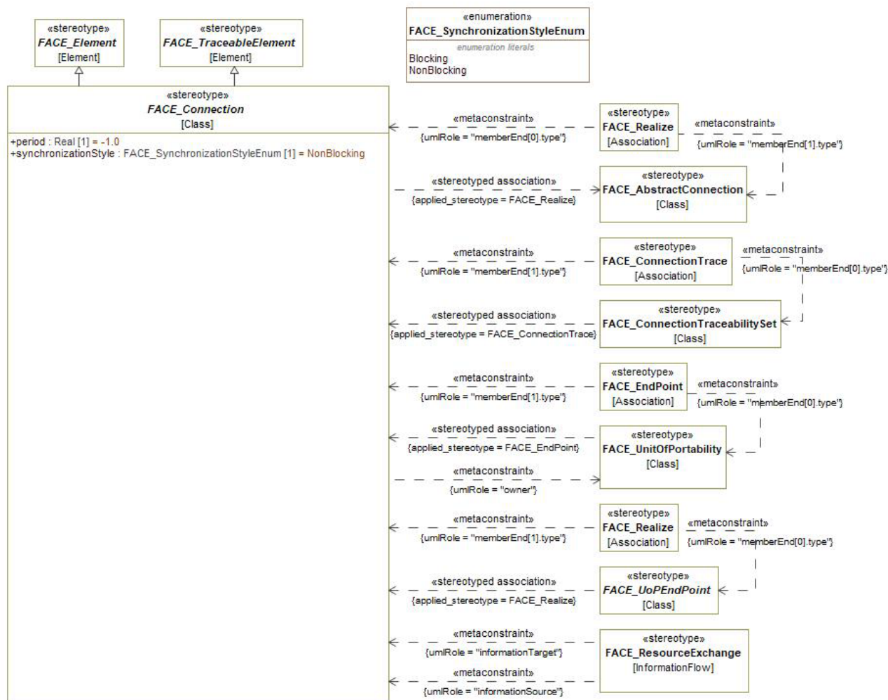
Figure 7-170: abstract FACE_Connection
