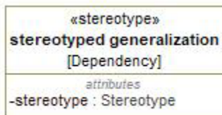
Figure 6-7: stereotyped generalization
