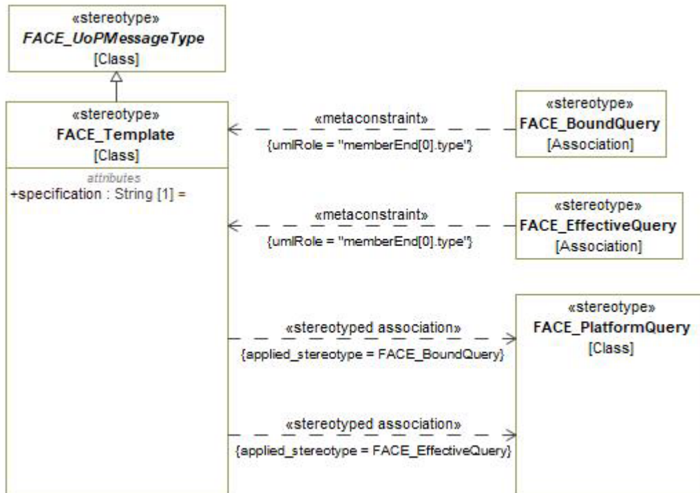
Figure 7-188: FACE_Template
