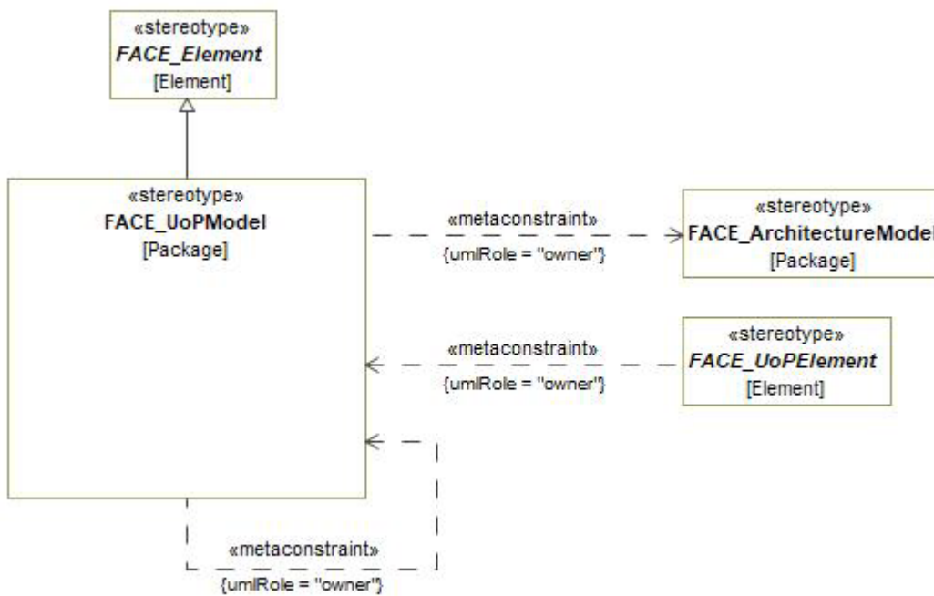
Figure 7-13: FACE_UoPModel
