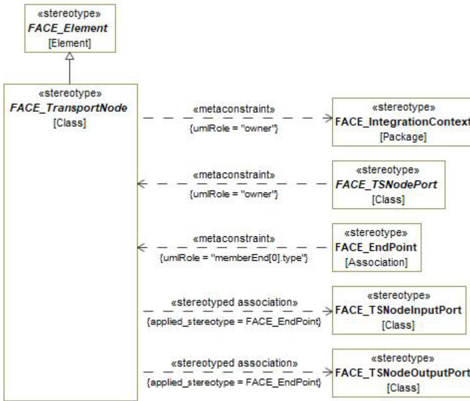
Figure 7-128: abstract FACE_TransportNode
