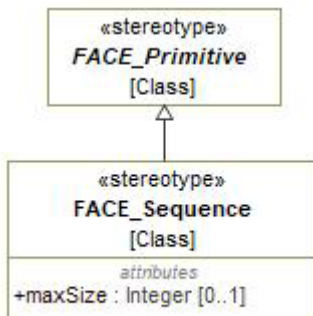
Figure 7-115: FACE_Sequence
