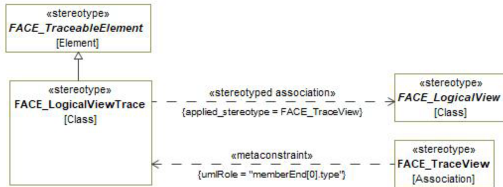
Figure 7-150: FACE_LogicalViewTrace
