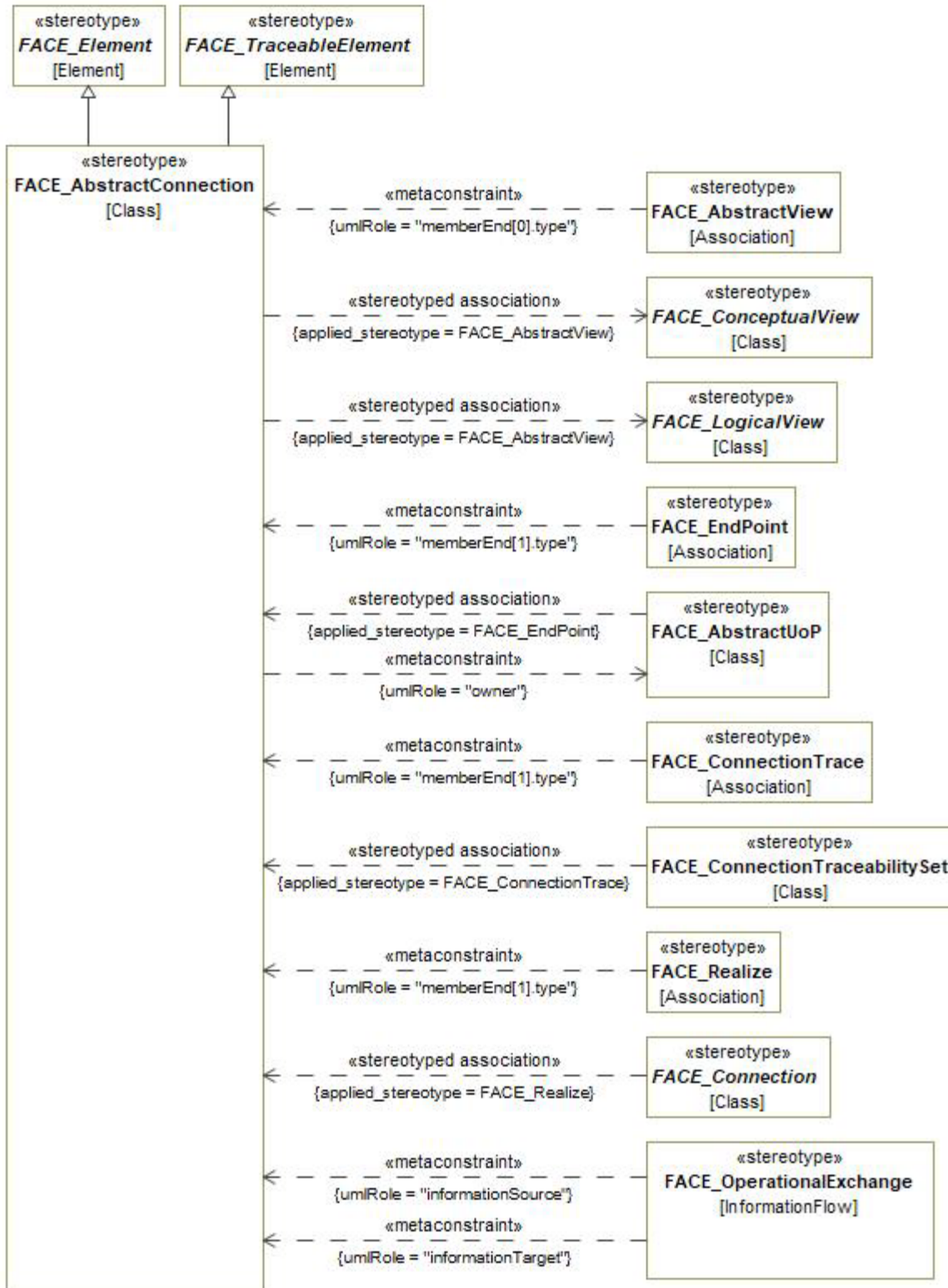
Figure 7-160: FACE_AbstractConnection
