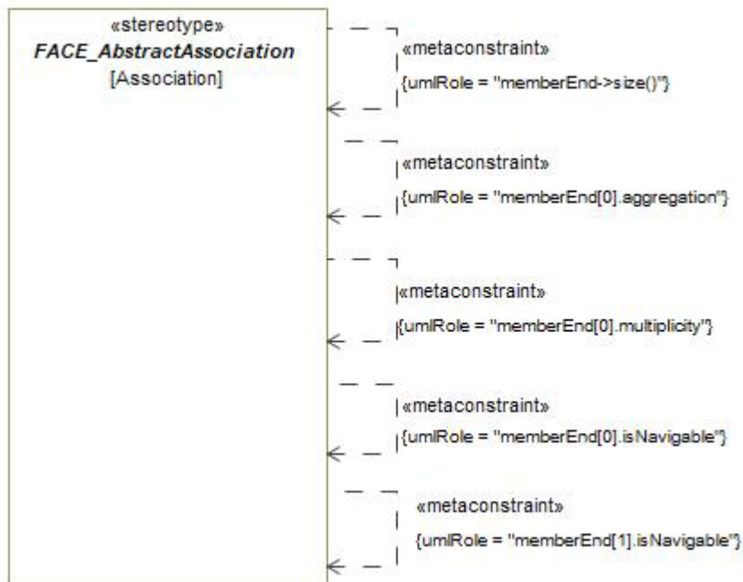
Figure 7-3: abstract FACE_AbstractAssociation
