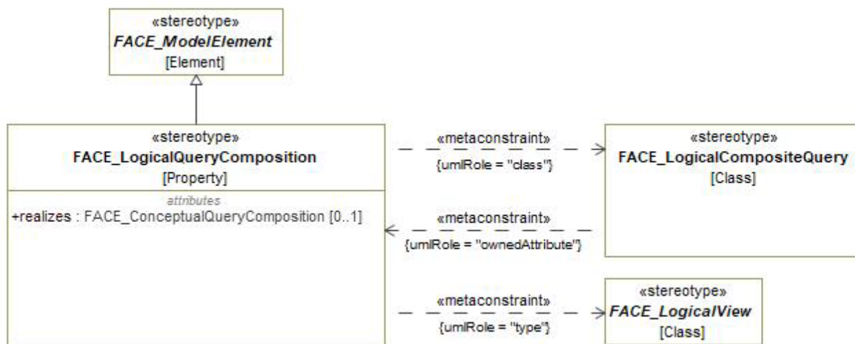
Figure 7-63: FACE_LogicalQueryComposition
