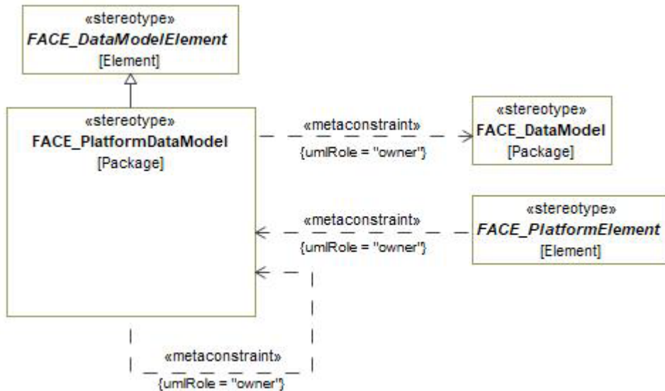
Figure 7-17: FACE_PlatformDataModel
