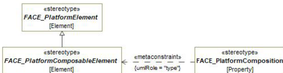
Figure 7-103: abstract FACE_PlatformComposableElement
