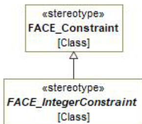
Figure 7-51: abstract FACE_IntegerConstraint
