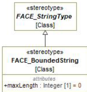
Figure 7-87: FACE_BoundedString
