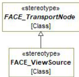
Figure 7-141: FACE_ViewSource
