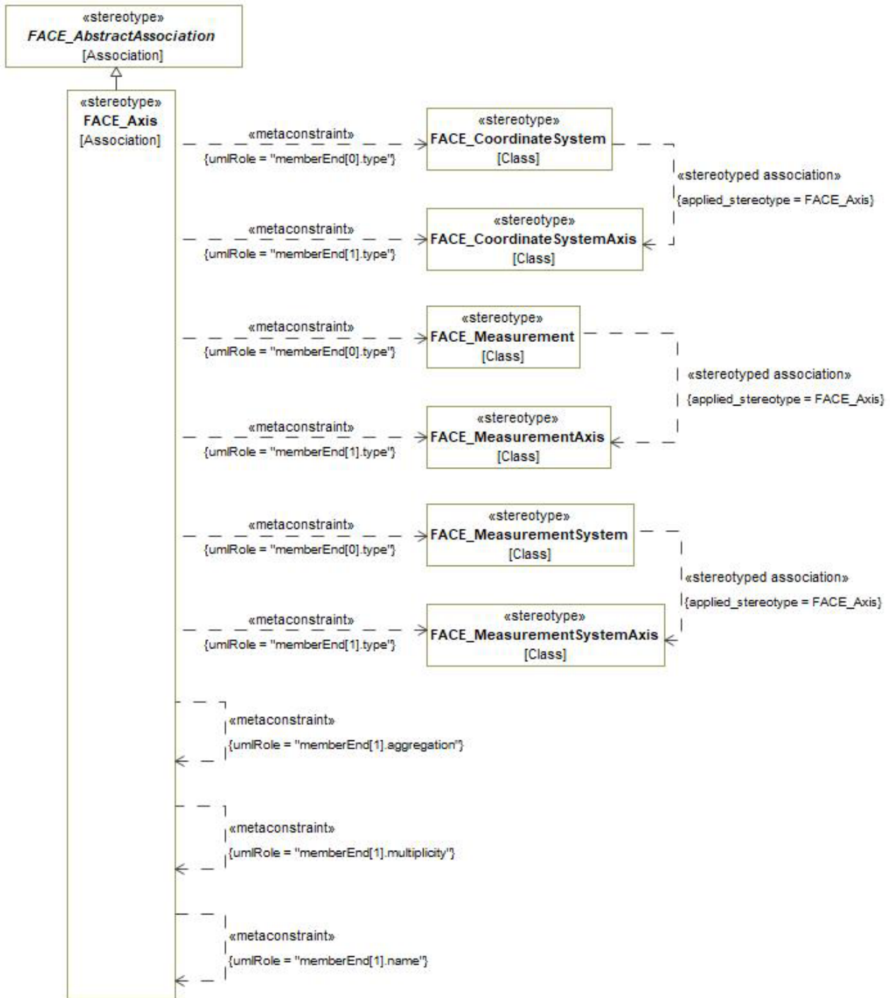
Figure 7-41: FACE_Axis
