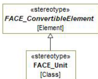
Figure 7-82: FACE_Unit
