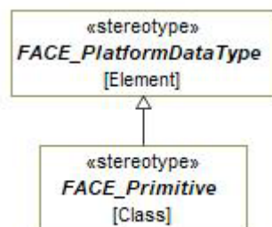
Figure 7-113: abstract FACE_Primitive
