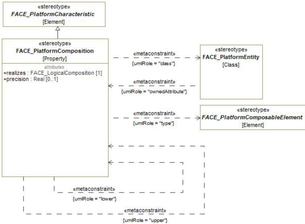
Figure 7-105: FACE_PlatformComposition
