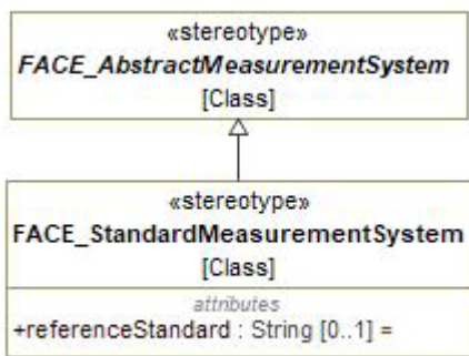
Figure 7-80: FACE_StandardMeasurementSystem
