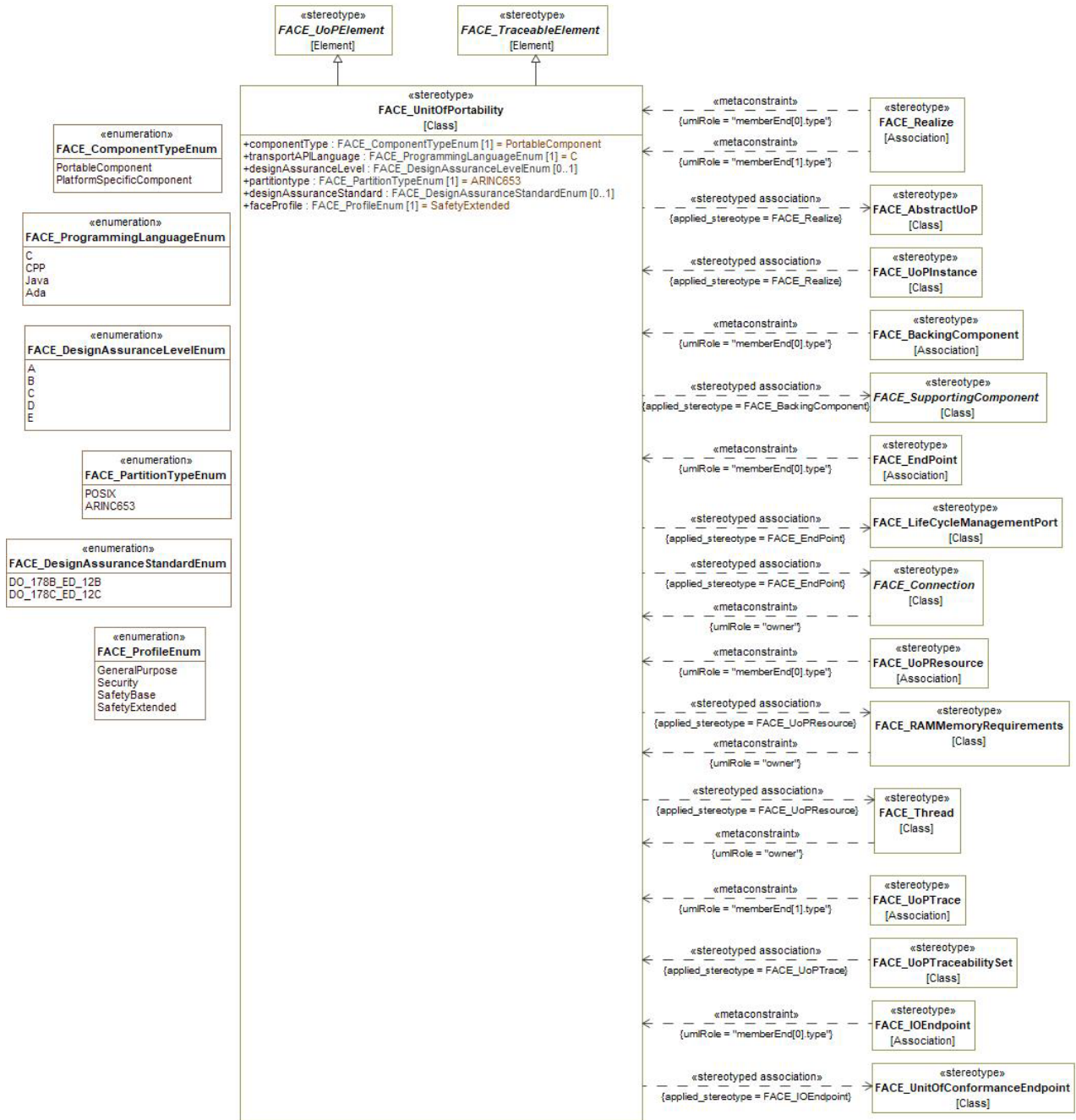
Figure 7-192: FACE_UnitOfPortability
