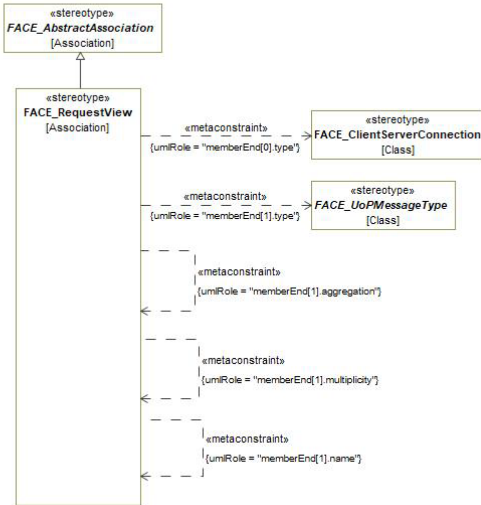
Figure 7-183: FACE_RequestView
