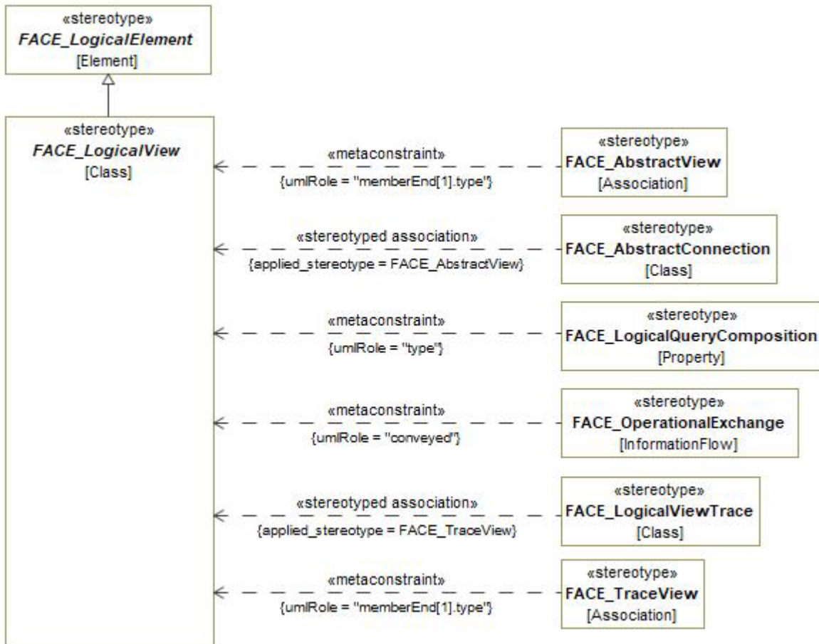
Figure 7-65: abstract FACE_LogicalView
