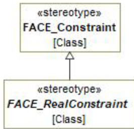
Figure 7-74: abstract FACE_RealConstraint
