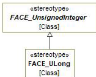
Figure 7-121: FACE_ULong
