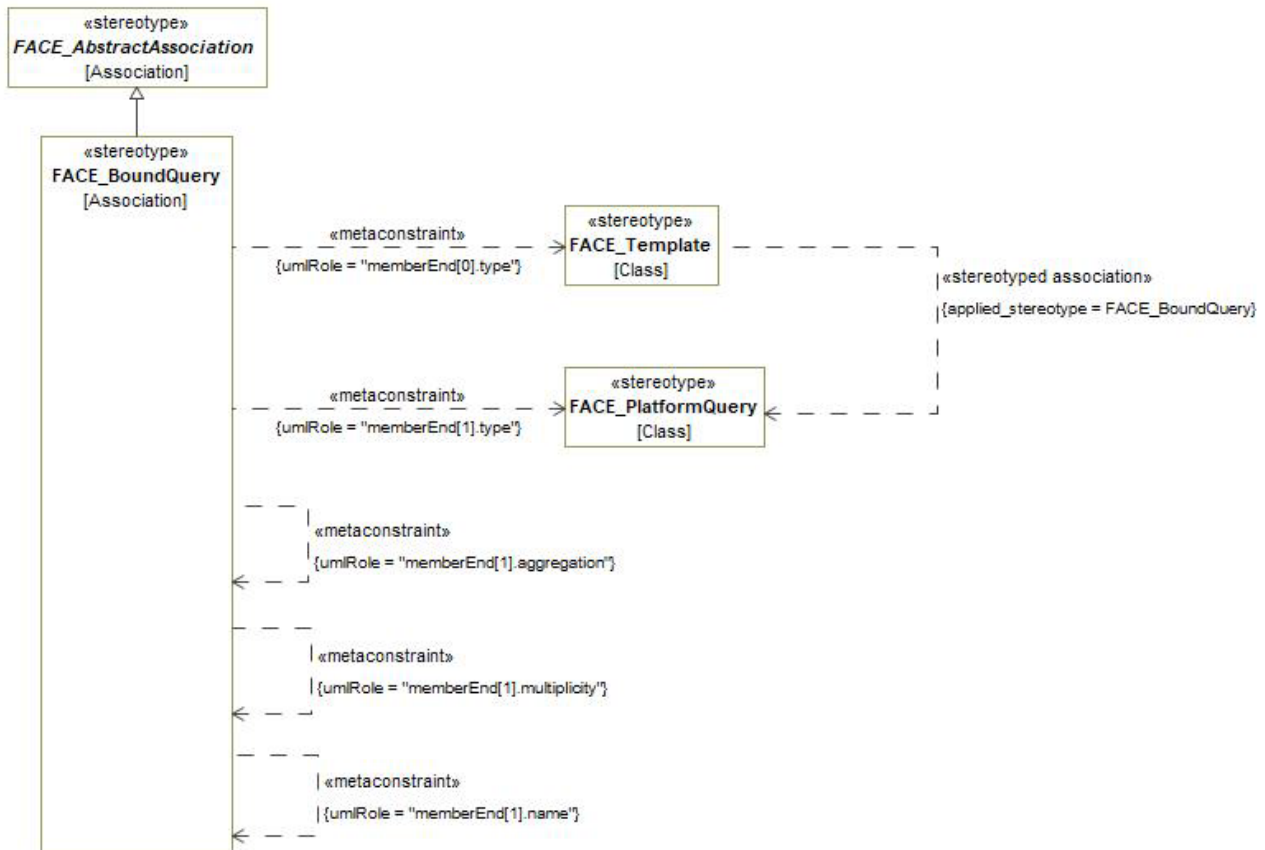
Figure 7-164: FACE_BoundQuery
