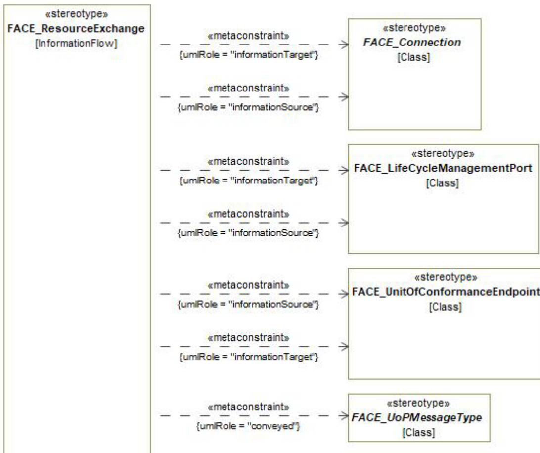
Figure 7-198: FACE_ResourceExchange
