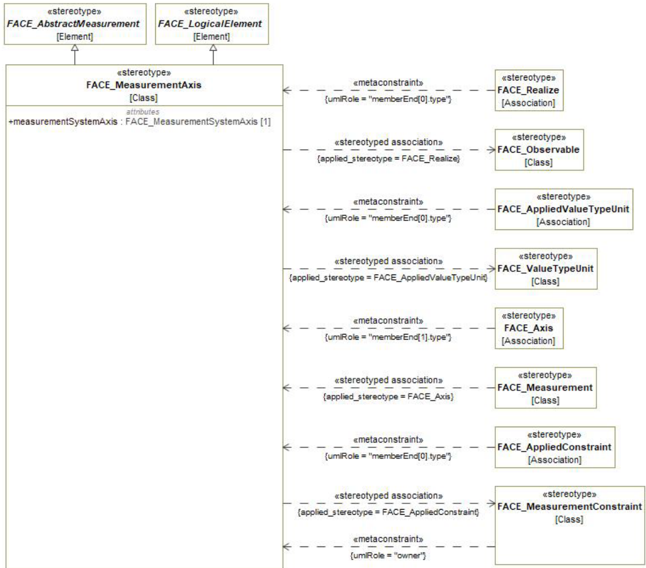
Figure 7-68: FACE_MeasurementAxis
