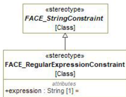
Figure 7-78: FACE_RegularExpressionConstraint
