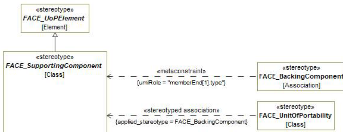
Figure 7-174: FACE_LanguageRunTime
