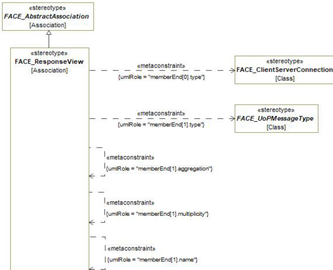
Figure 7-184: FACE_ResponseView
