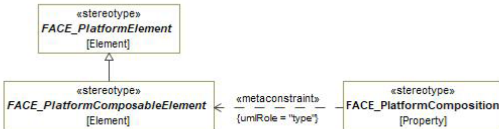
Figure 7-103: abstract FACE_PlatformComposableElement
