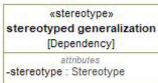
Figure 6-7: stereotyped generalization
