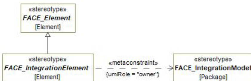
Figure 7-126: abstract FACE_IntegrationElement
