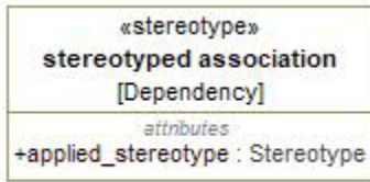
Figure 6-5: stereotyped association
