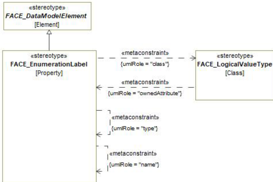
Figure 7-49: FACE_EnumerationLabel
