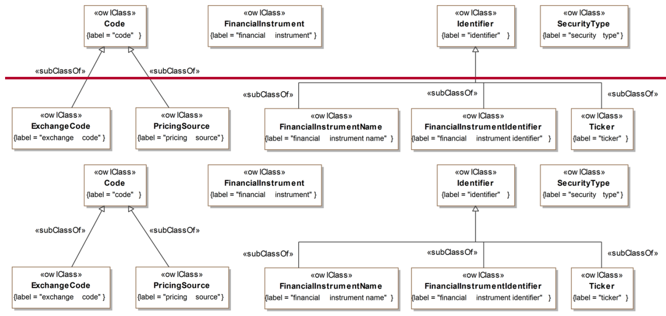
Figure 8.1-1: Top-Level Class Hierarchy
