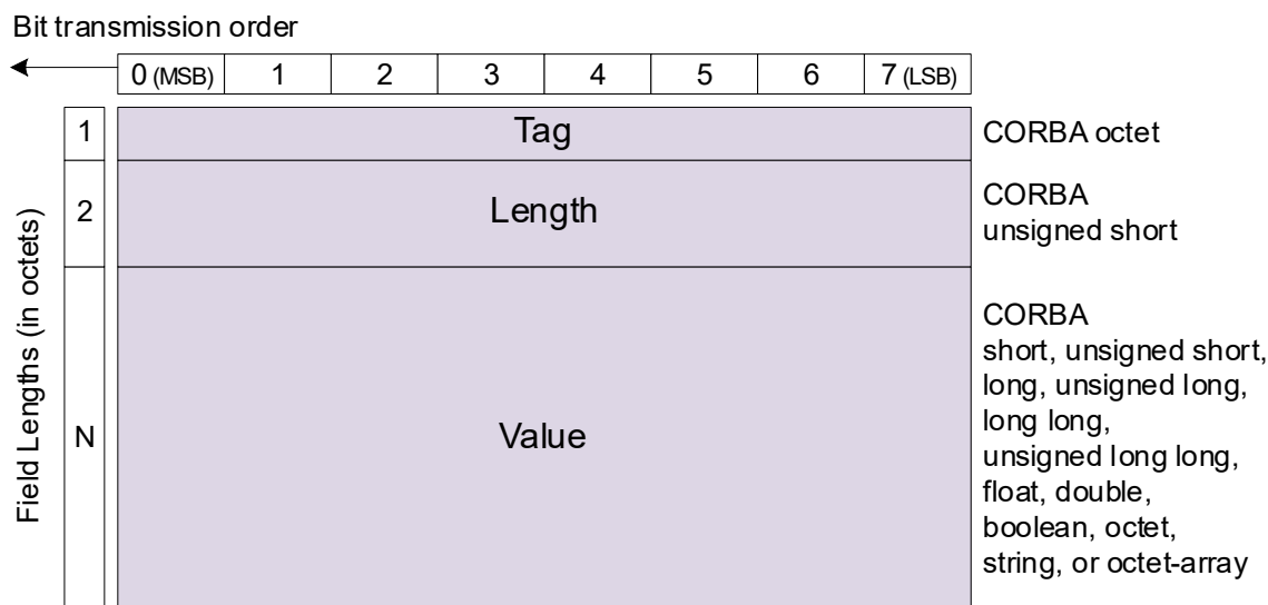
Figure 11 – TLV Triplet: CORBA Encoded Format
