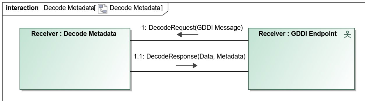
Figure 4 - Decode Metadata Use Case
