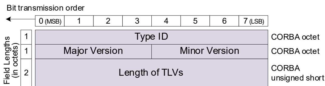
Figure 10 - Type Header: CORBA Encoded Format
