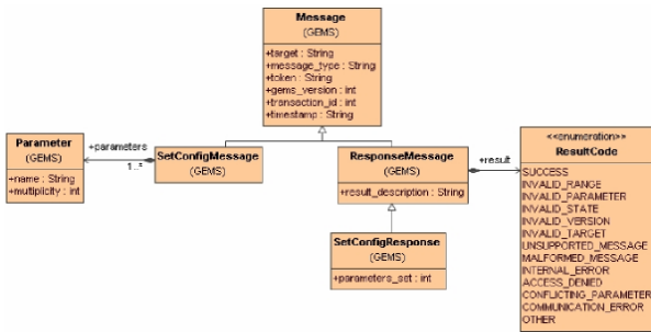
Figure 6.8 - Set Configuration Message Classes
