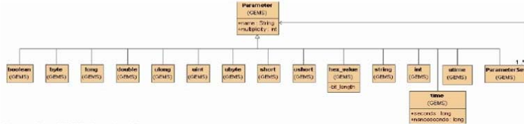
Figure 6.4 - GEMS Standard Types
