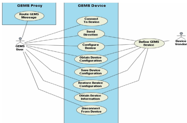
Figure 6.1 - GEMS Use Cases
