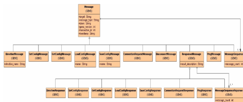
Figure 6.5 - GEMS Message Classes
