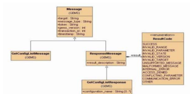
Figure 6.12 - Get Configuration List UML
