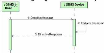
Figure 6.13 - GEMS Directive Sequence
