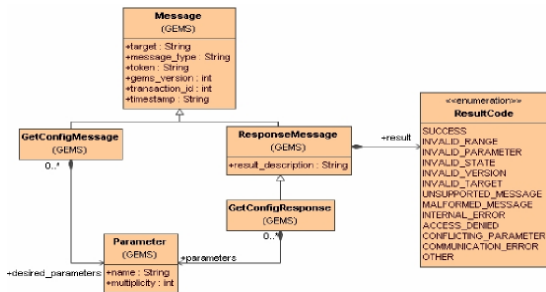
Figure 6.10 - Save Configuration UML
