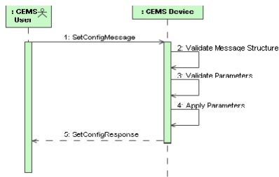
Figure 6.7 - Set Configuration Sequence
