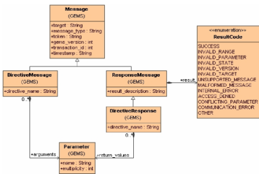
Figure 6.14 - Directive UML
