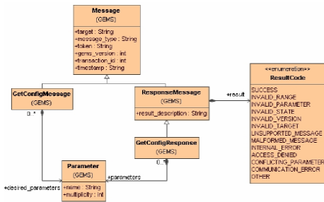
Figure 6.9 - GetConfigMessage UML
