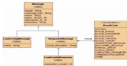
Figure 6.11 - Load Configuration UML
