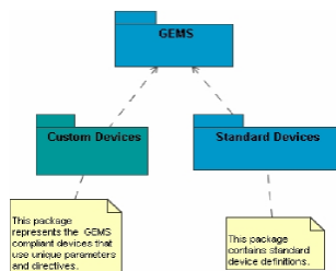
Figure 6.2 - GEMS Packages
