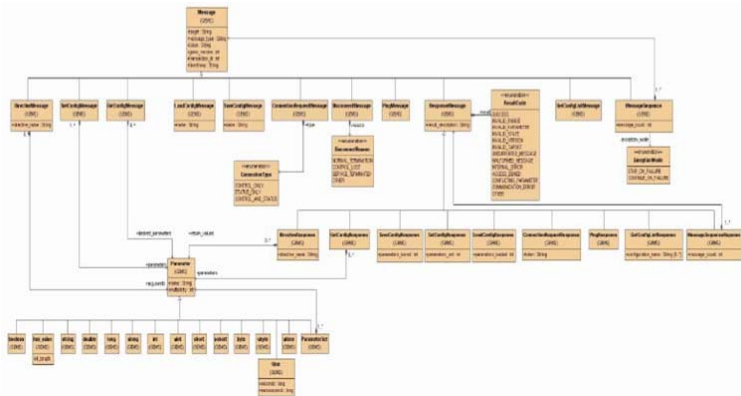
Figure 6.3 - GEMS UML
