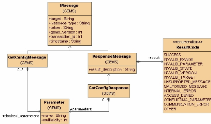
Figure 6.9 - GetConfigMessage UML
