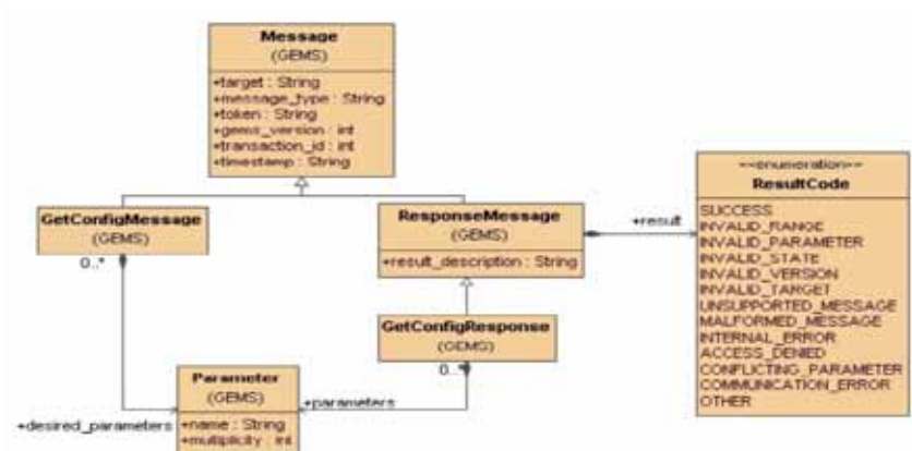
Figure 6.10 - Save Configuration UML
