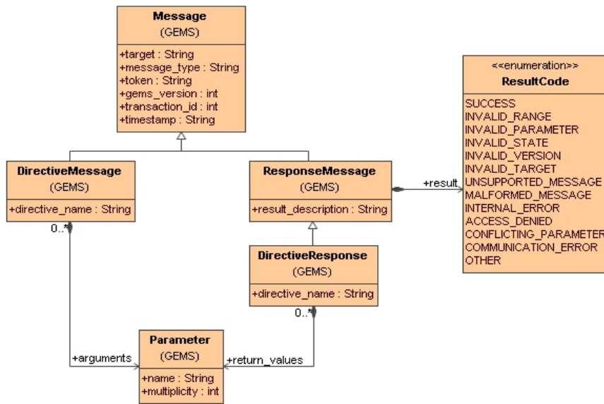
Figure 6.14 - Directive UML
