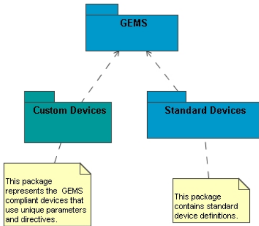
Figure 6.2 - GEMS Packages
