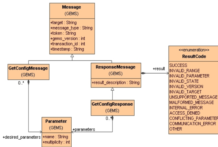
Figure 6.9 - GetConfigMessage UML
