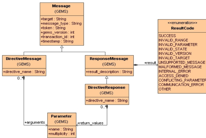
Figure 6.14 - Directive UML
