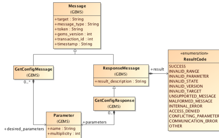
Figure 6.15 GetConfigMessage classes
