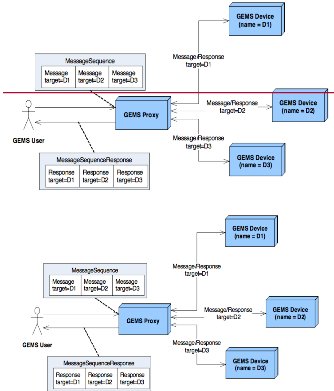
Figure 6.6 Message routing
