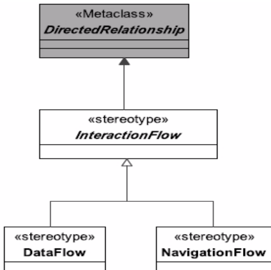
Figure 11.8 - InteractionFlow stereotypes
