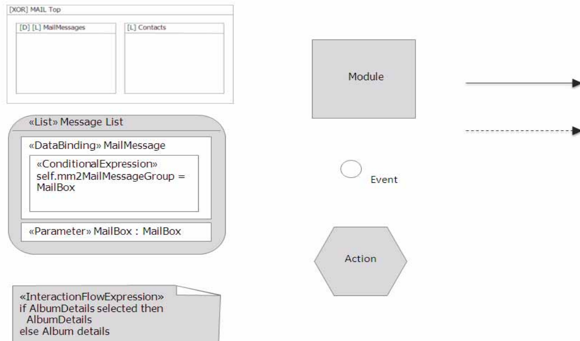
Figure 10.3 - Notational patterns
