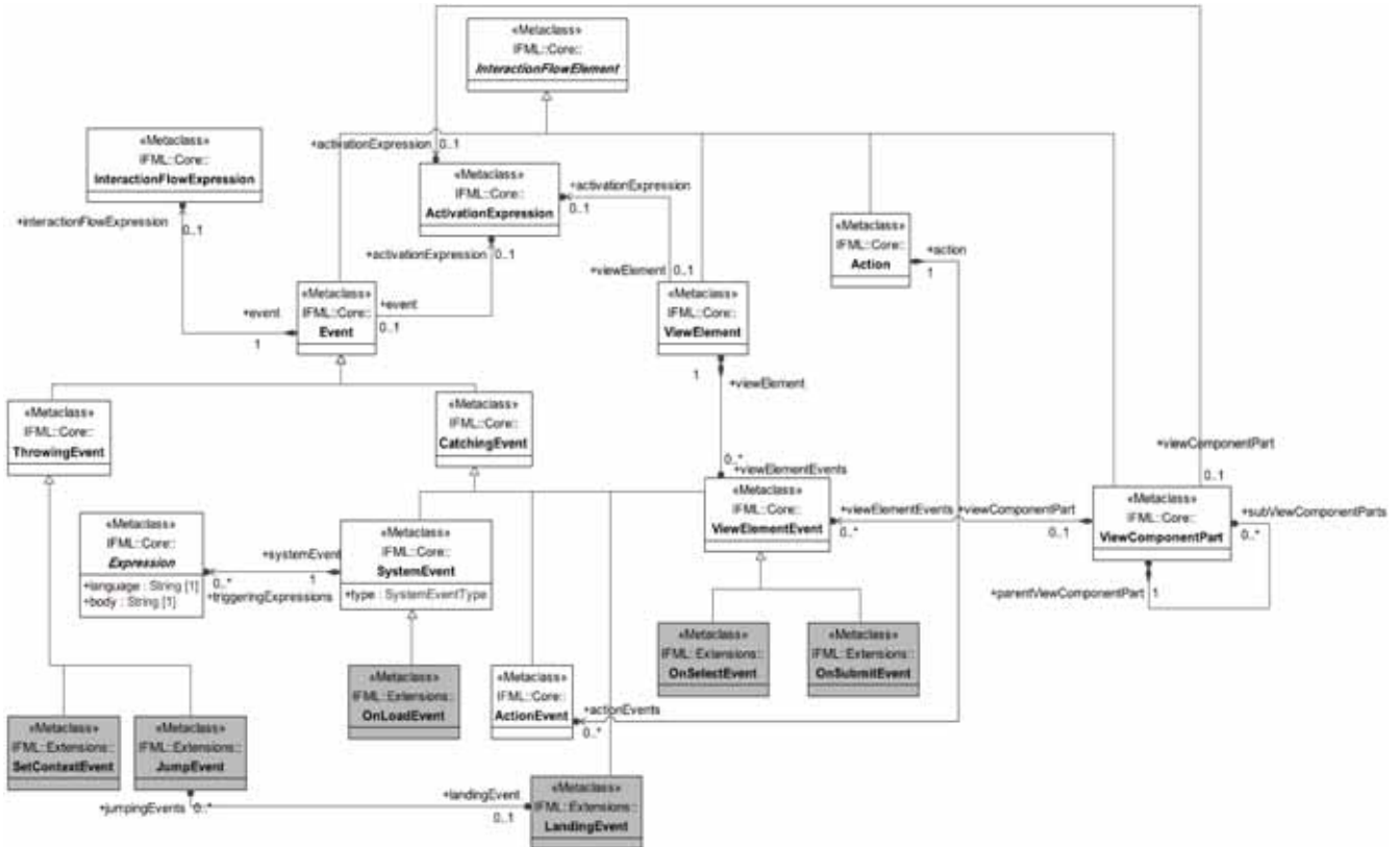
Figure 8.6 - Events
