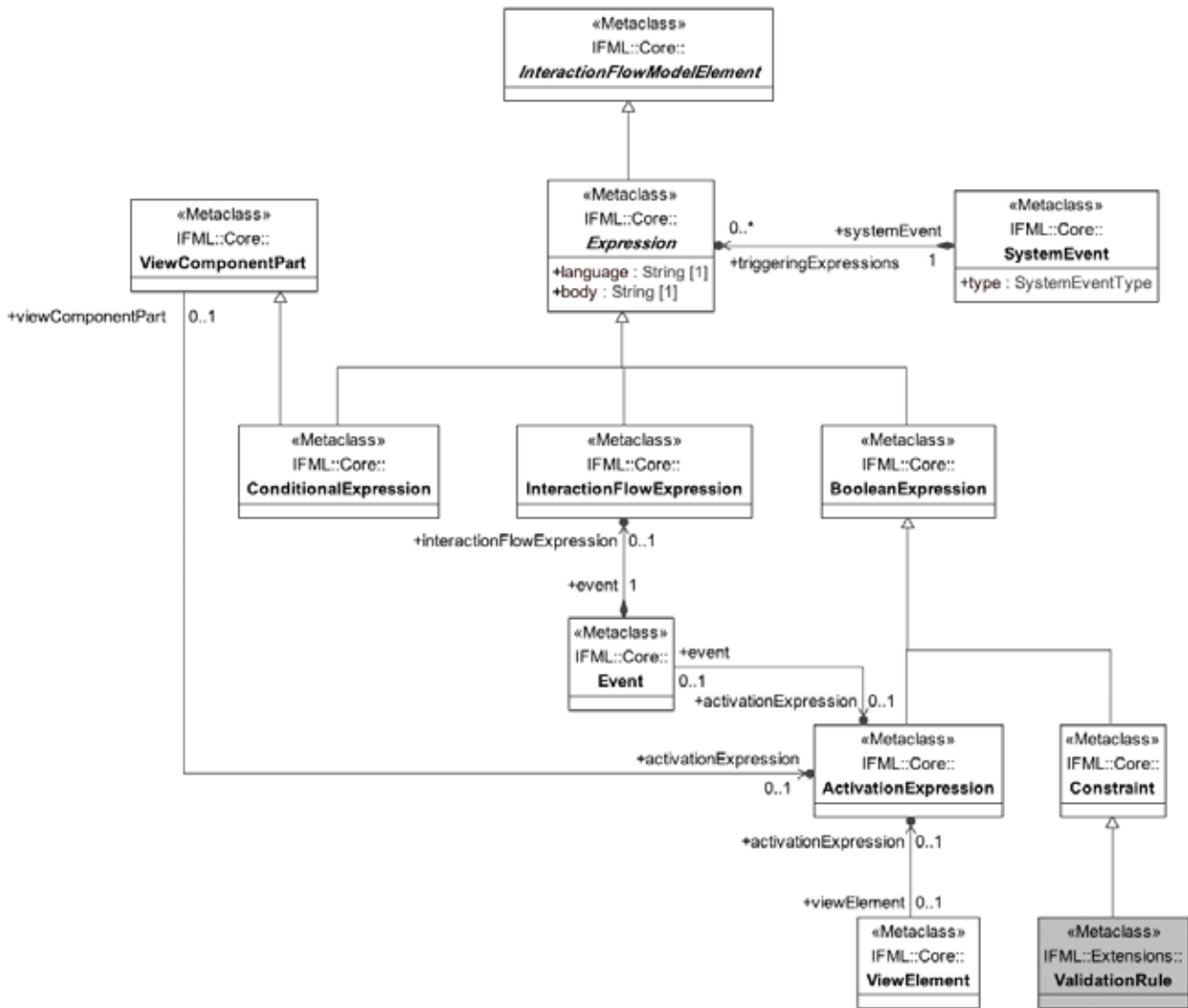
Figure 8.7 - Expressions
