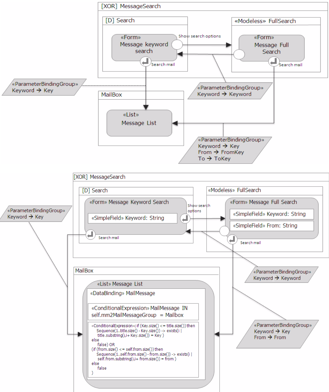
Figure A.20 - The model of the message search functionality (top). The same model refined with the use of the extended view components «Form» and «List» (bottom).
