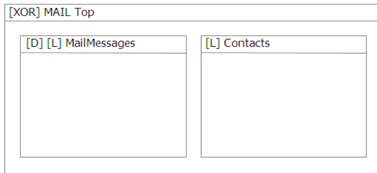
Figure A.5 - IFML model of the Top Container of the email application
