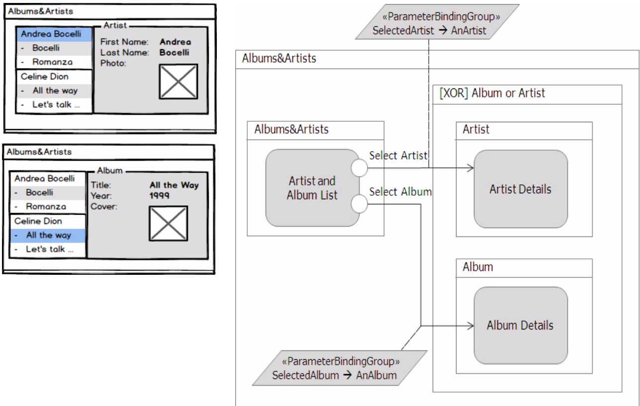
Figure 7.2 - Example of user interface (left) and corresponding IFML model (right). One top-level container comprises three view containers: one with a list of artists and of their albums, one with the details of an artist, and one with the details of an album. The latter two view containers are mutually exclusive: only one at a time is displayed.
