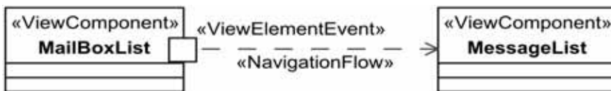
Figure 11.11 - Stereotyped UML diagram with IFML Core
