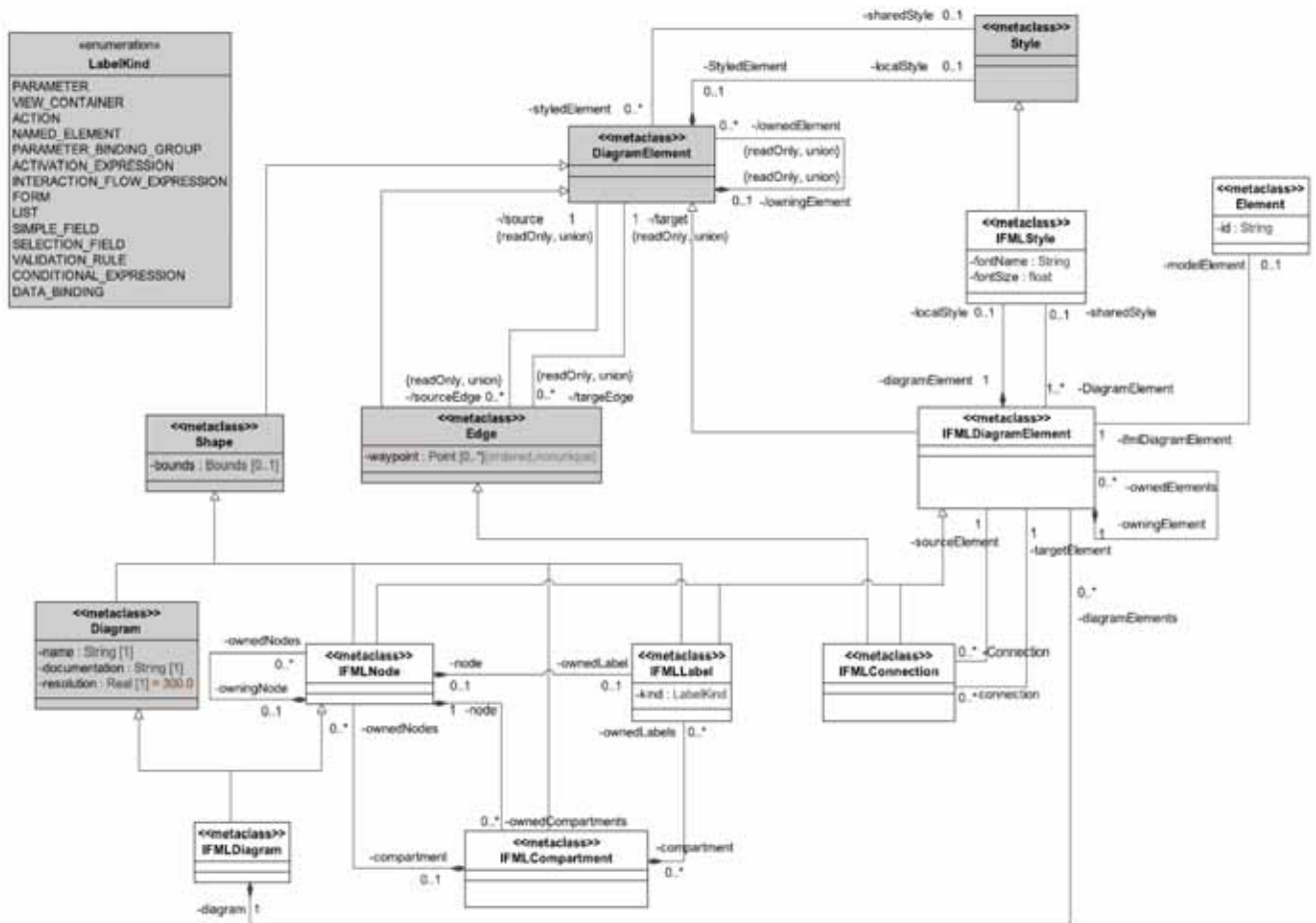
Figure 10.2 - Diagram Interchange (DI) Meta-model
