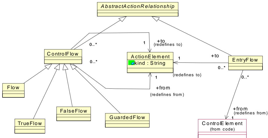
Figure 13.3 - ActionFlow Class Diagram
