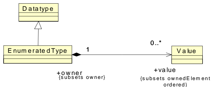
Figure 12.8 - EnumeratedTypes Class Diagram
