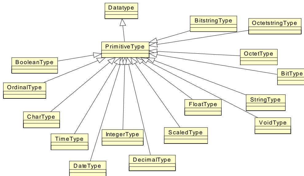
Figure 12.7 - PrimitiveTypes Class Diagram
