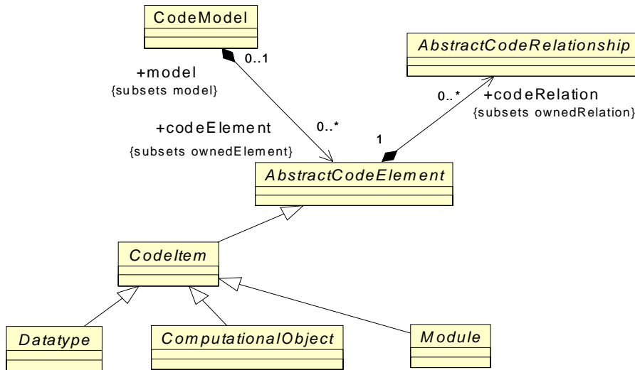
Figure 12.1 - CodeModel Class Diagram
