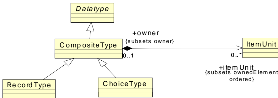
Figure 12.9 - CompositeTypes Class Diagram
