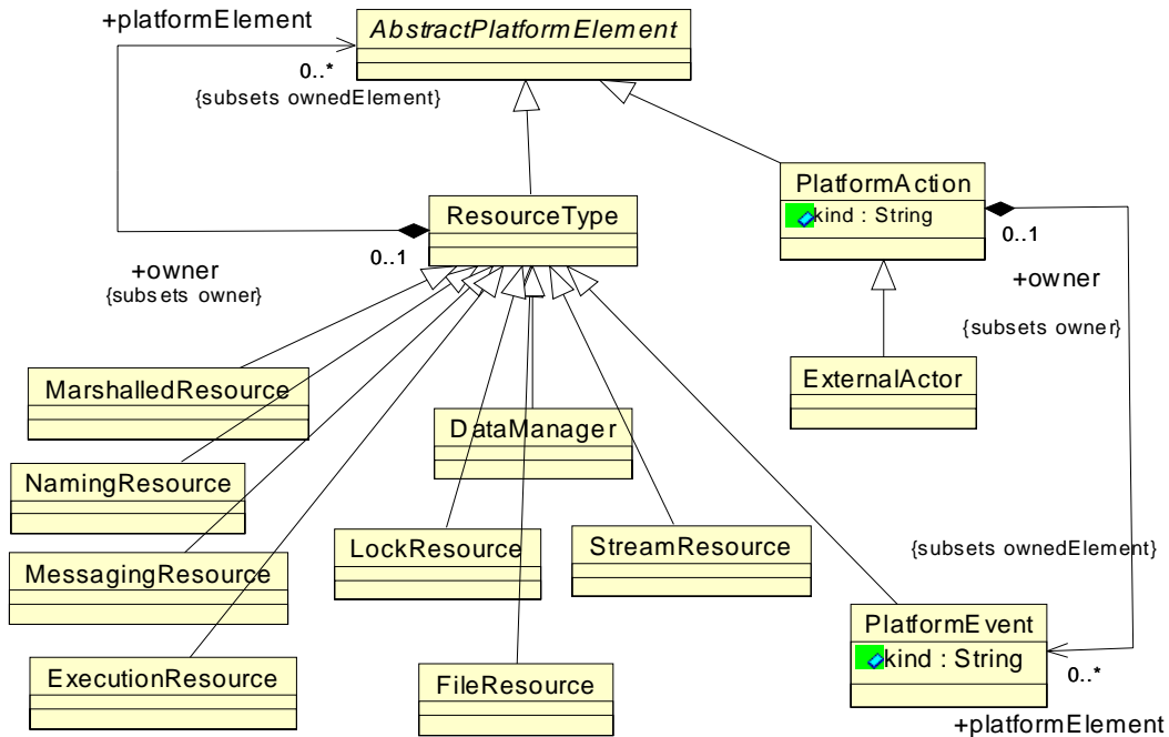
Figure 15.2 - PlatformResources Class Diagram
