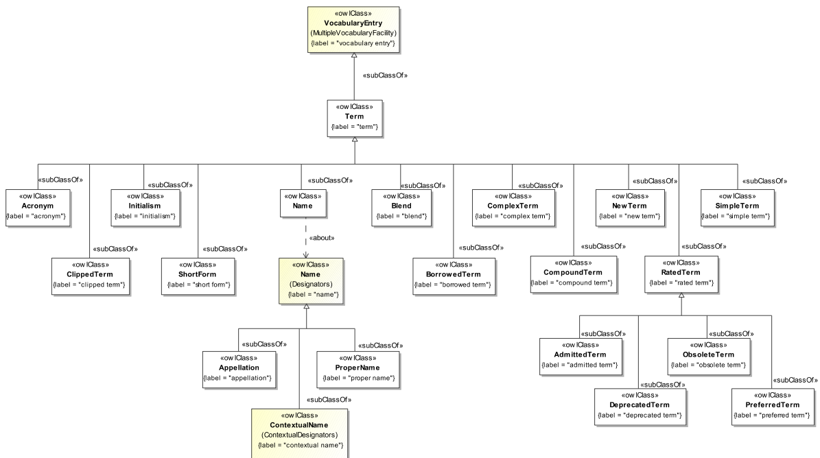
Figure 10.6: ISO 1087 Term Class Hierarchy
