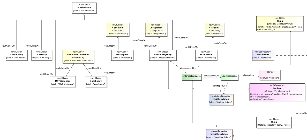
Figure 10.1: MVF Class Hierarchy / Overview
