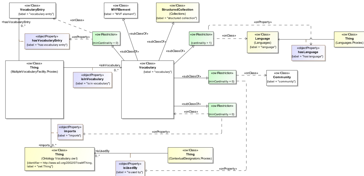
Figure 10.4: MVF Vocabulary Class Diagram
