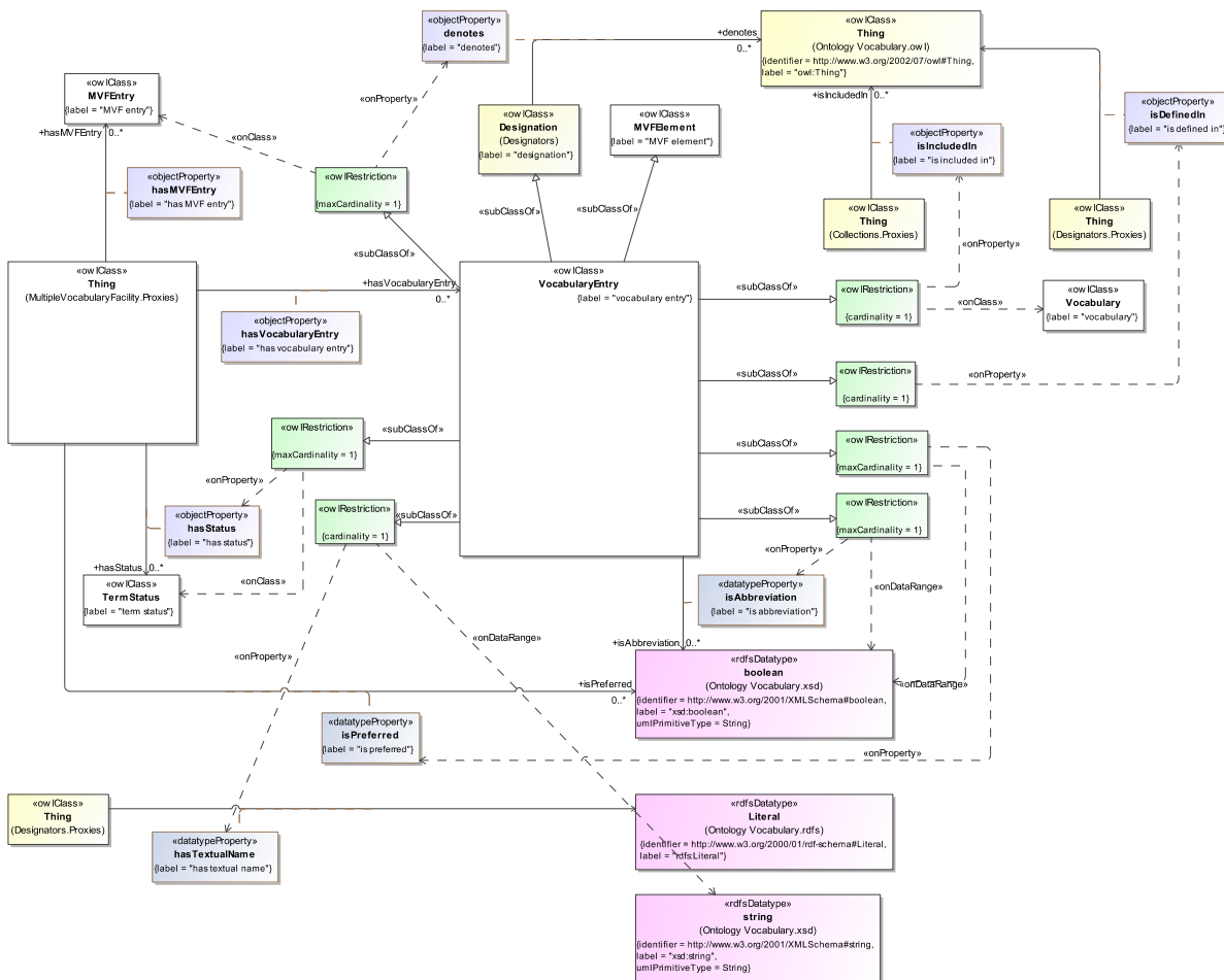
Figure 10.5: MVF Vocabulary Entry Class Diagram
