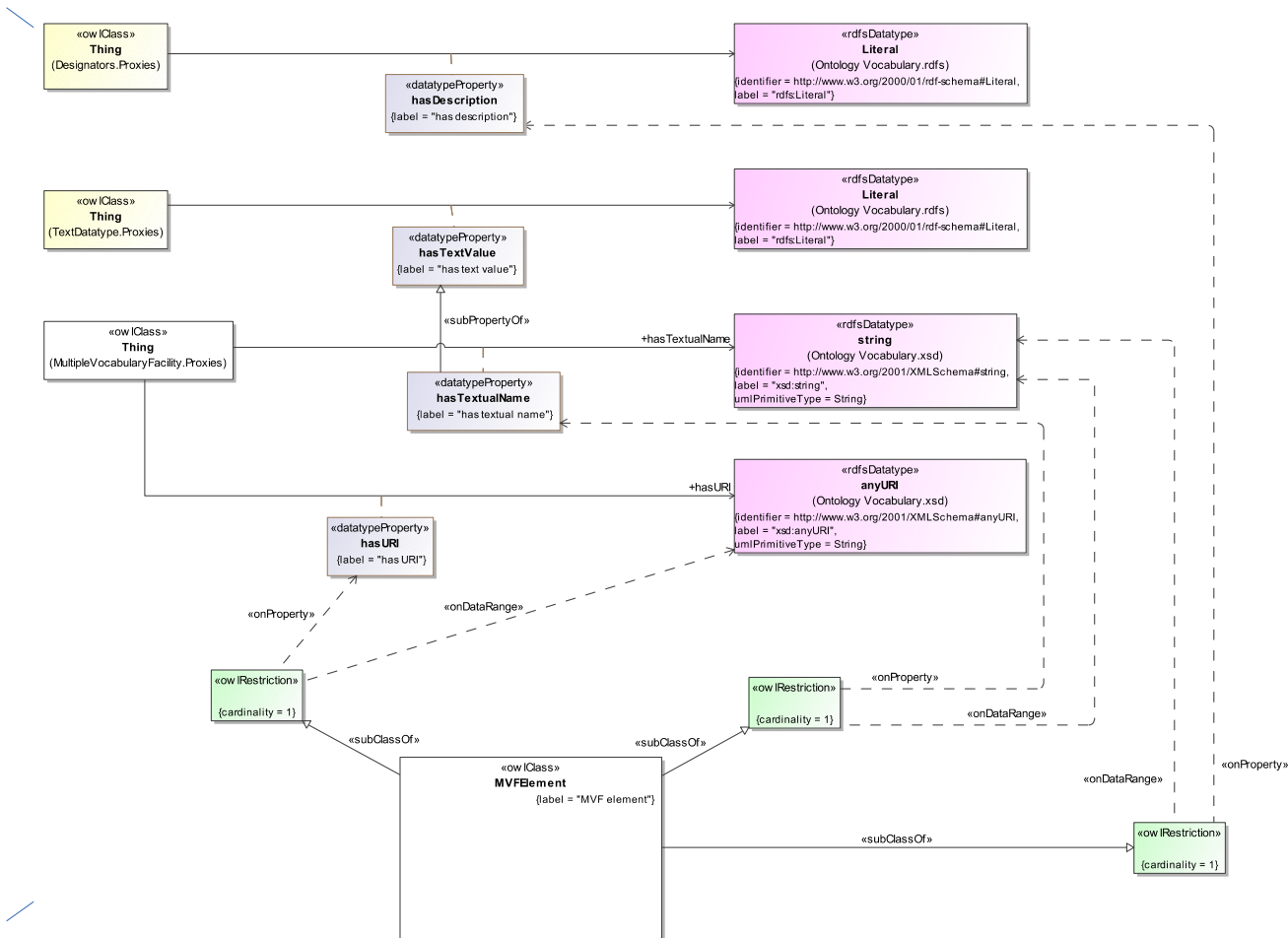
Figure 5: MVF Element Class Diagram
