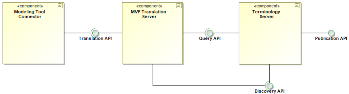
Figure 13: Notional Component / Interface Integration
