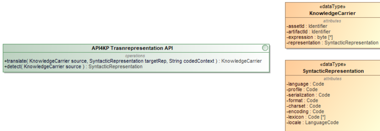
Figure 15: API4KP Translation API
