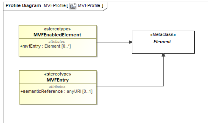
Figure 3: Multiple Vocabulary Facility UML Profile
