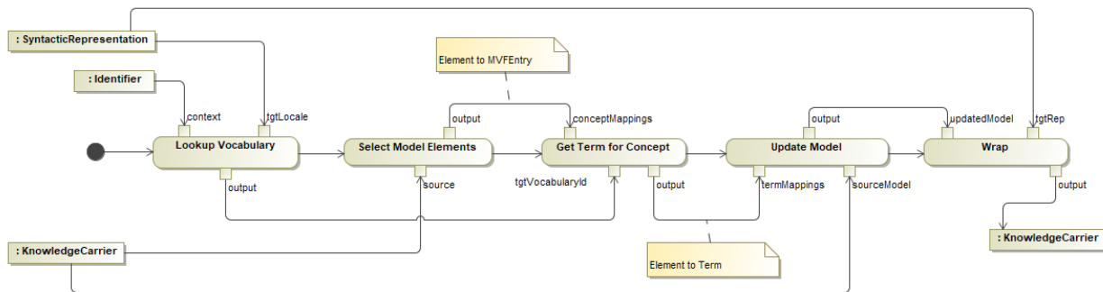
Figure 17: API4KP-based Specification of the MVF-profiled api4kp:translate operation
