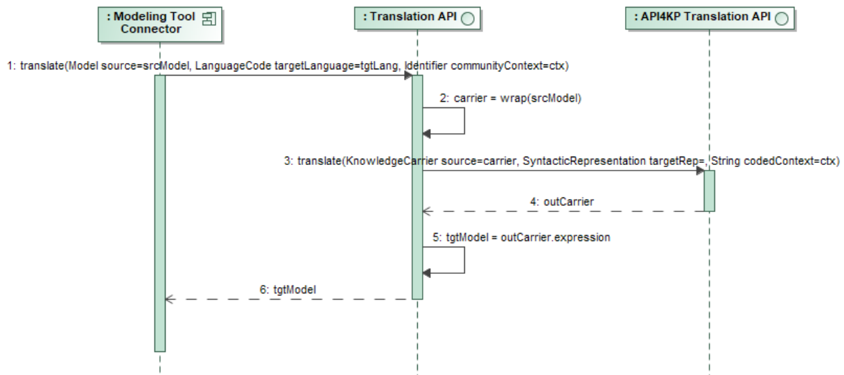
Figure 16: MVF to API4KP Delegation
