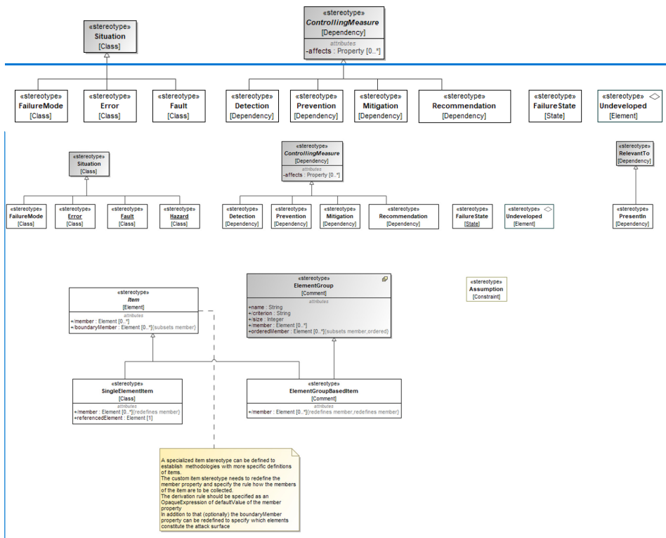
Figure 10.4 – General Concepts Profile
