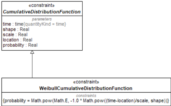
Figure 9.230 – WeibullCumulativeDistributionFunction
