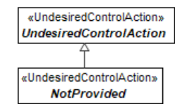
Figure 9.105 – NotProvided
