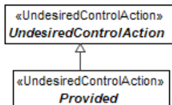
Figure 9.104 – Provided
