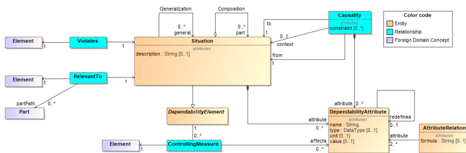
Figure 9.1 – Core concepts domain model
