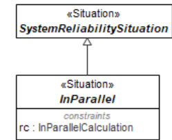
Figure 9.214 - InParallel Attributes
