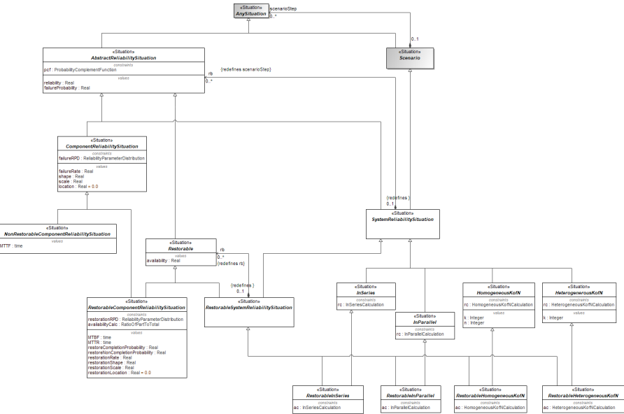
Figure 10.21 - RBD Library Elements
