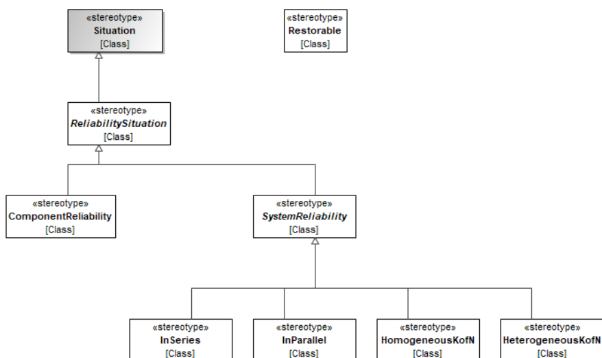
Figure 10.34 - RBD Profile Elements
