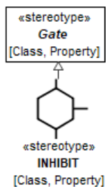
Figure 9.92 – INHIBIT
