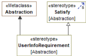
Figure 9.178 – UserInfoRequirement
