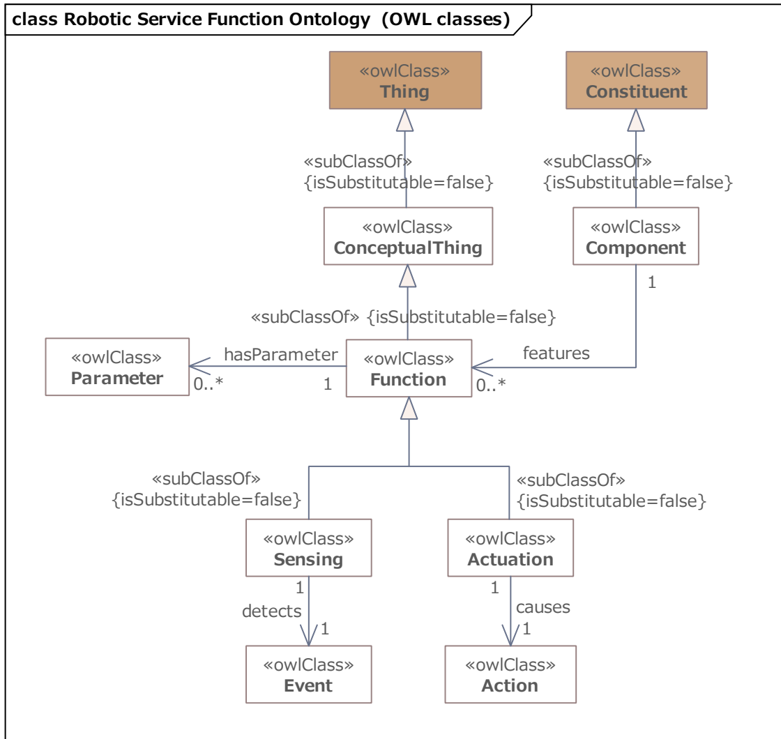
Figure 7: Robotic Service Function Ontology (OWL classes)
