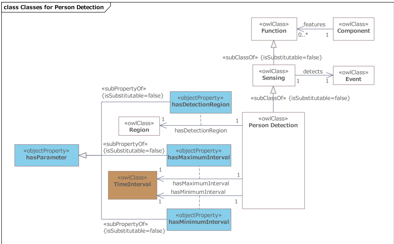
Figure 9: RoIS Person Detection Component (OWL classes)
