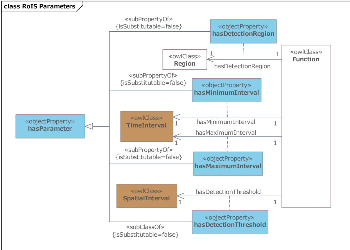
Figure 10: RoIS Person Detection Component (OWL properties)
