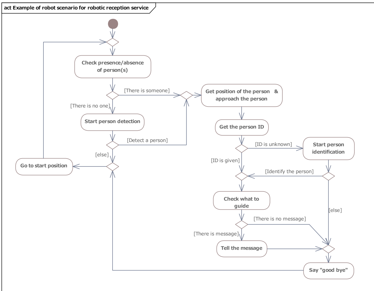
Figure 11: An example of Robotic Reception Service
