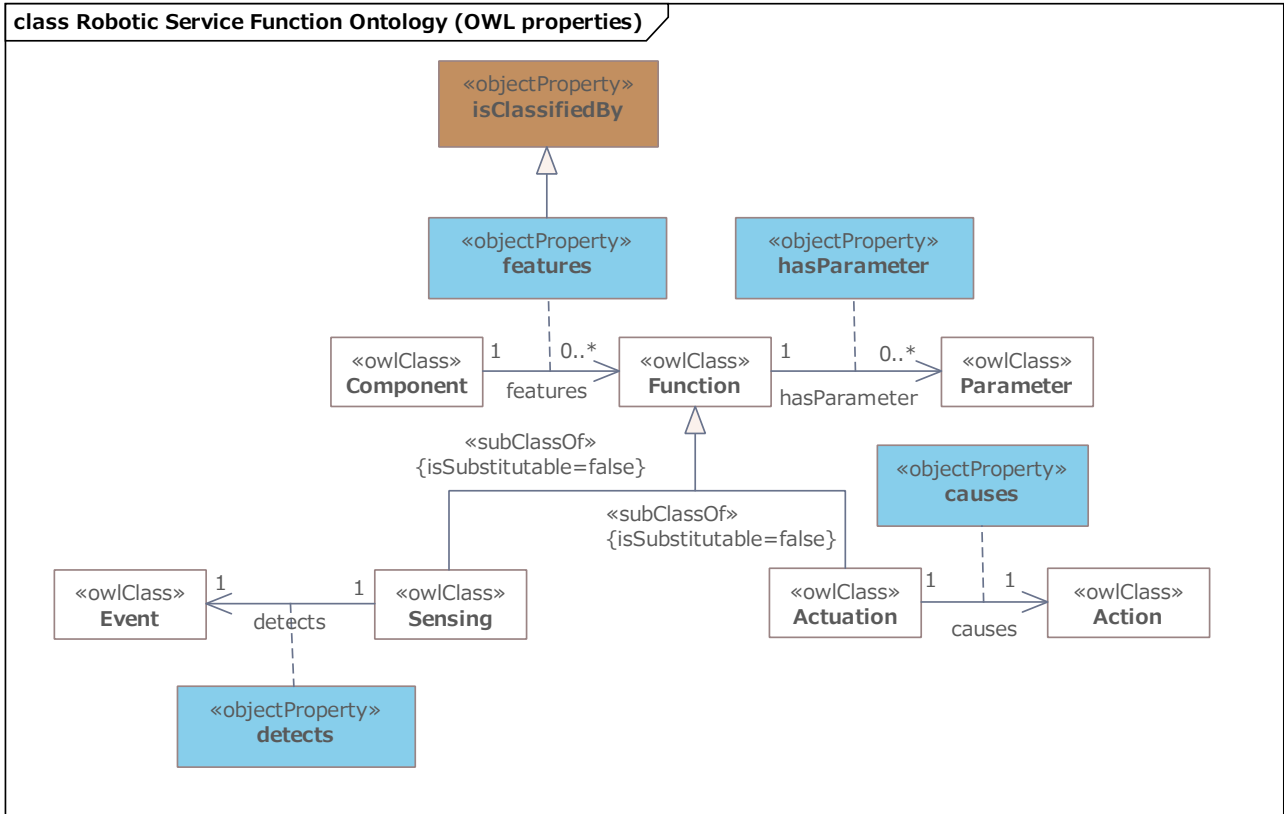
Figure 8: Robotic Service Function Ontology (OWL properties)
