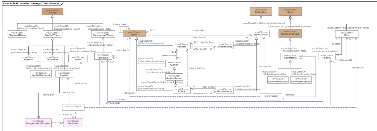
Figure 3 - Robotic Service Ontology (OWL classes)
