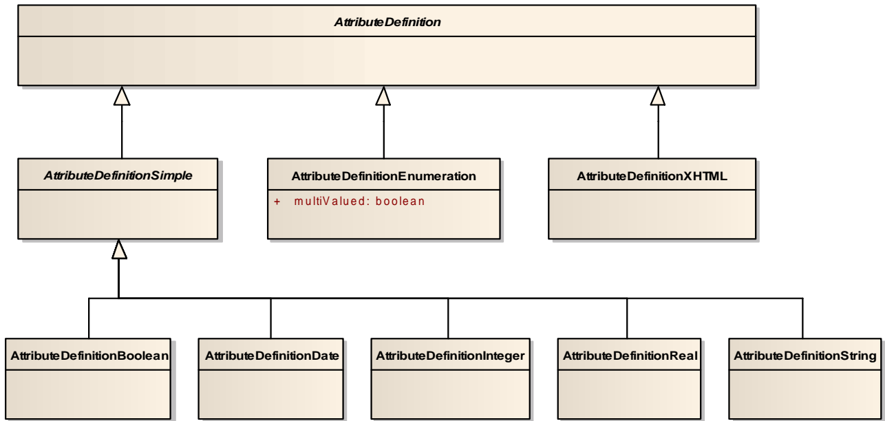
Figure 10.4 - AttributeDefinition class hierarchy
