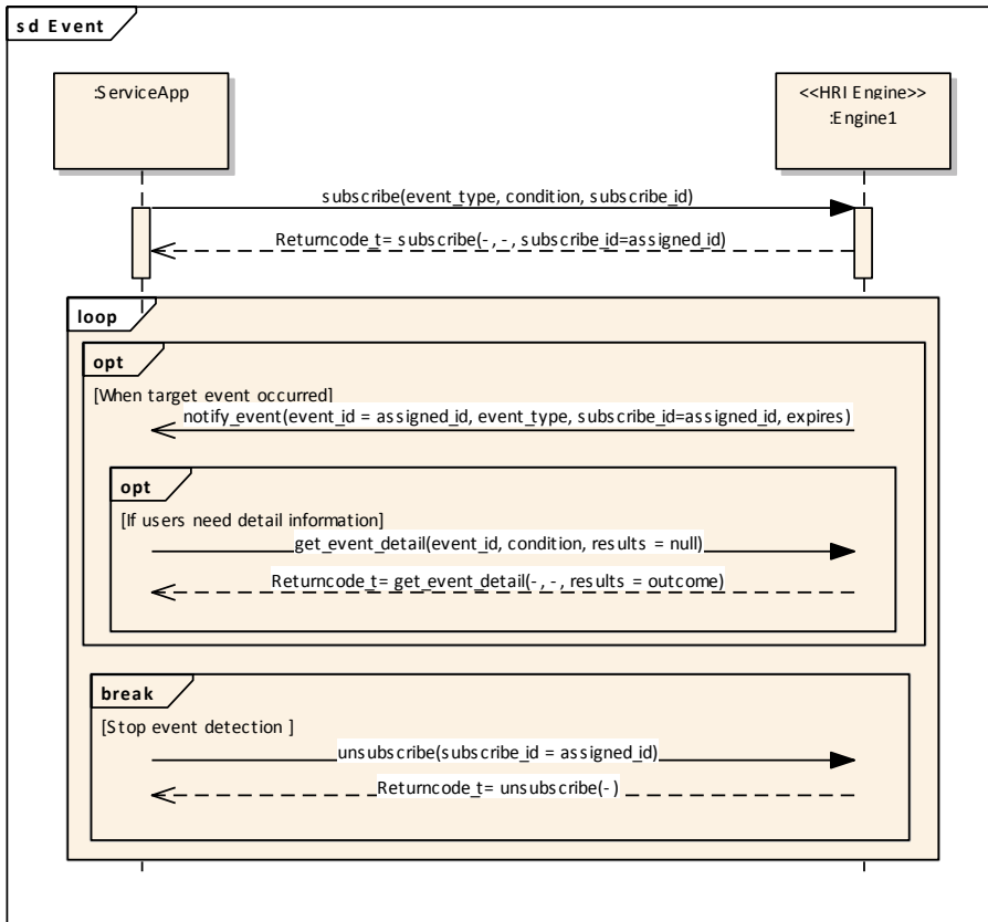
Figure 13: Sequence Diagram of Event Interface.
