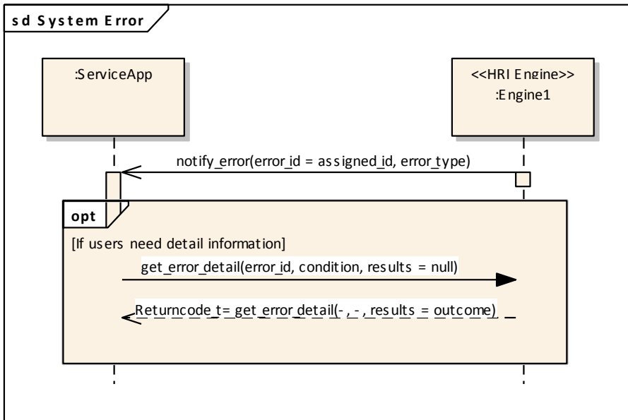
Figure 7: Sequence Diagram of System Interface (System Error)
