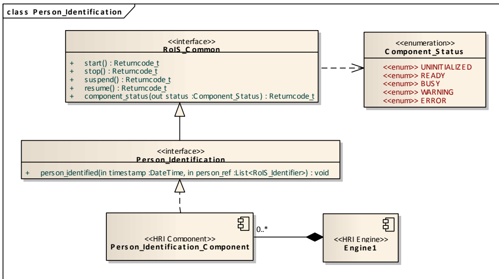
Figure 20: person identification
