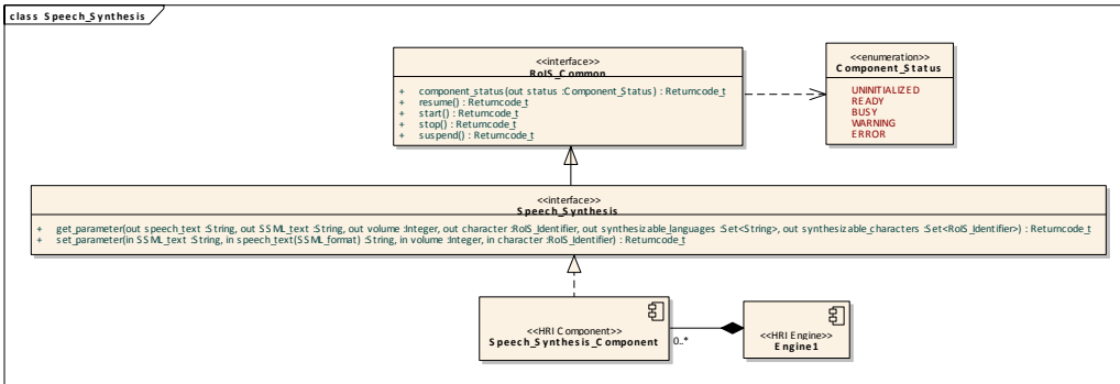
Figure 27: speech synthesis
