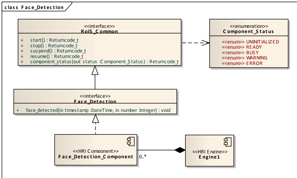
Figure 21 : face detection
