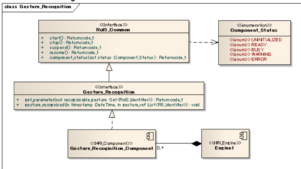
Figure 26: gesture recognition
