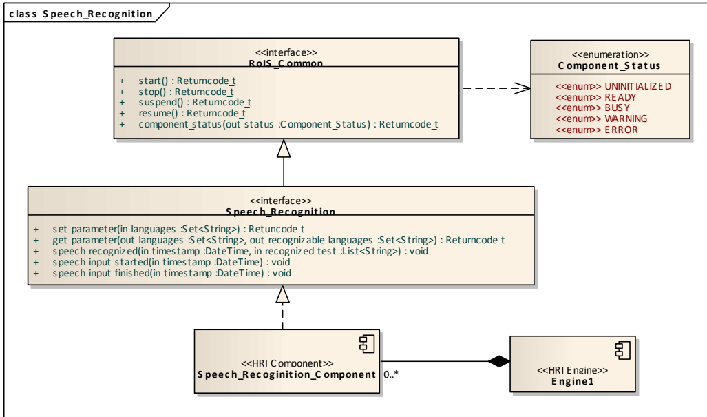
Figure 25: speech recognition
