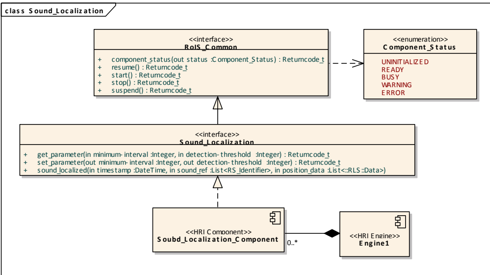
Figure 24: sound localization
