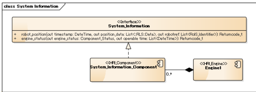
Figure 17: System Information
