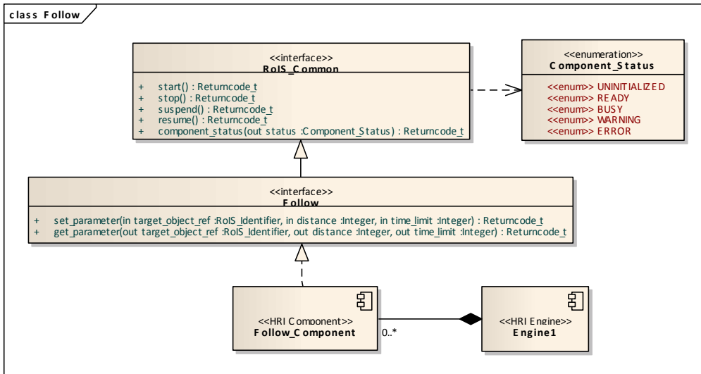
Figure 30: follow
