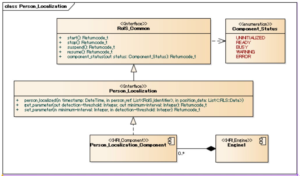
Figure 19 : person localization
