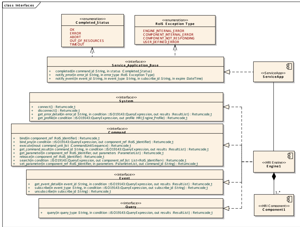
Figure 14 : RoIS Interfaces.
