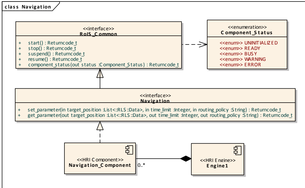
Figure 29: navigation
