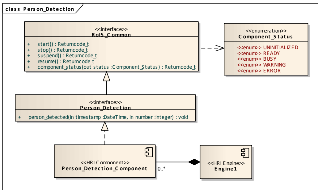
Figure 18 : person detection
