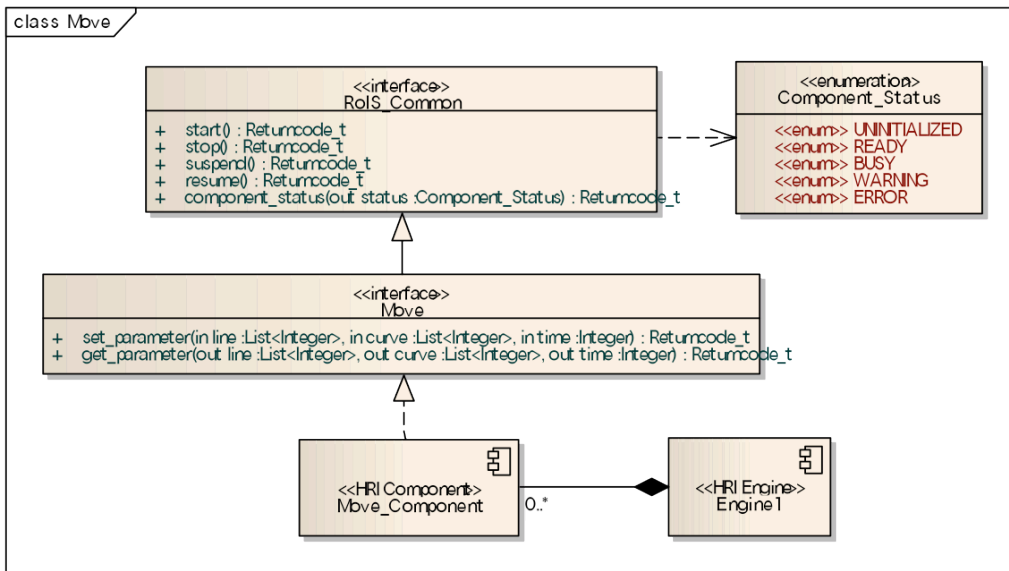
Figure 31: move
