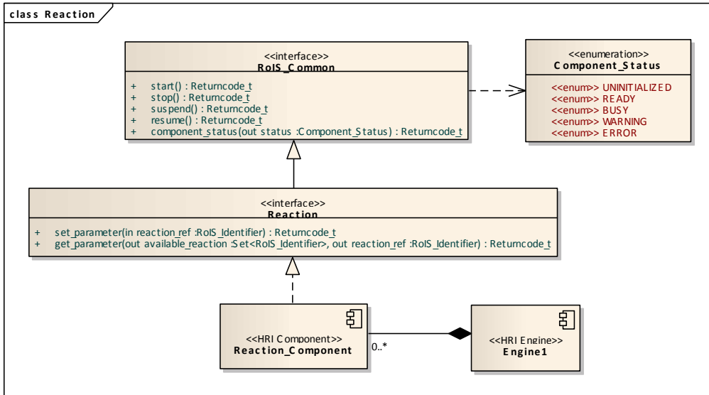
Figure 28: reaction
