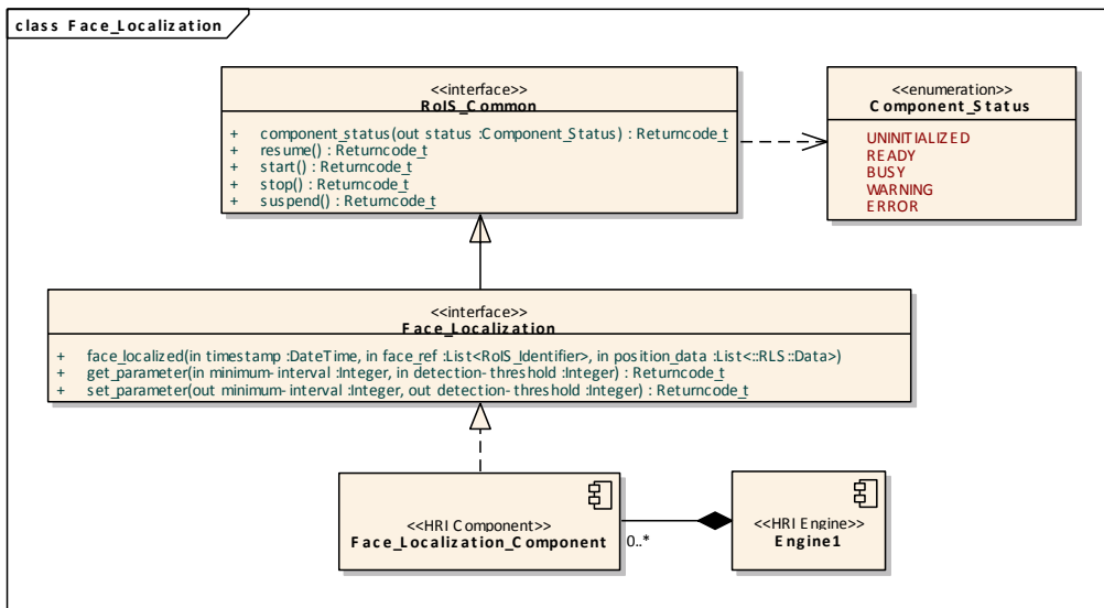
Figure 22: face localization
