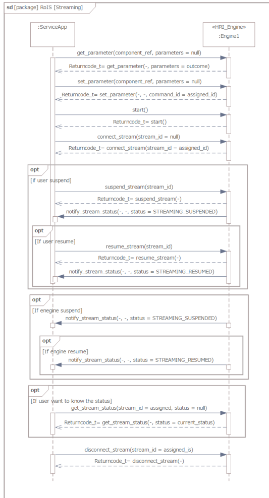
Figure 8.9: Sequence Diagram of Streaming Interface
