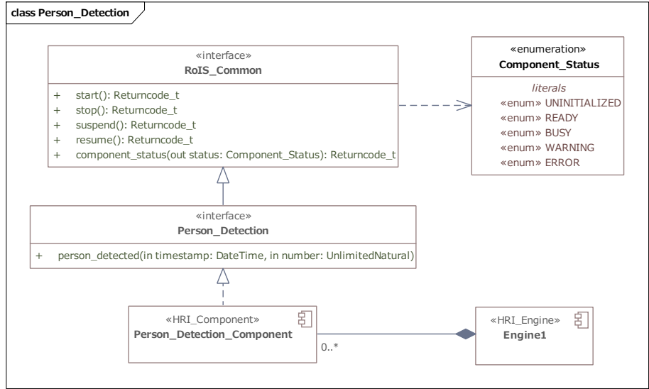
Figure 8.14: Person Detection
