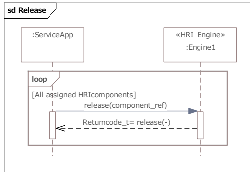
Figure 8.6: Sequence Diagram of “Release” in Command Interface
