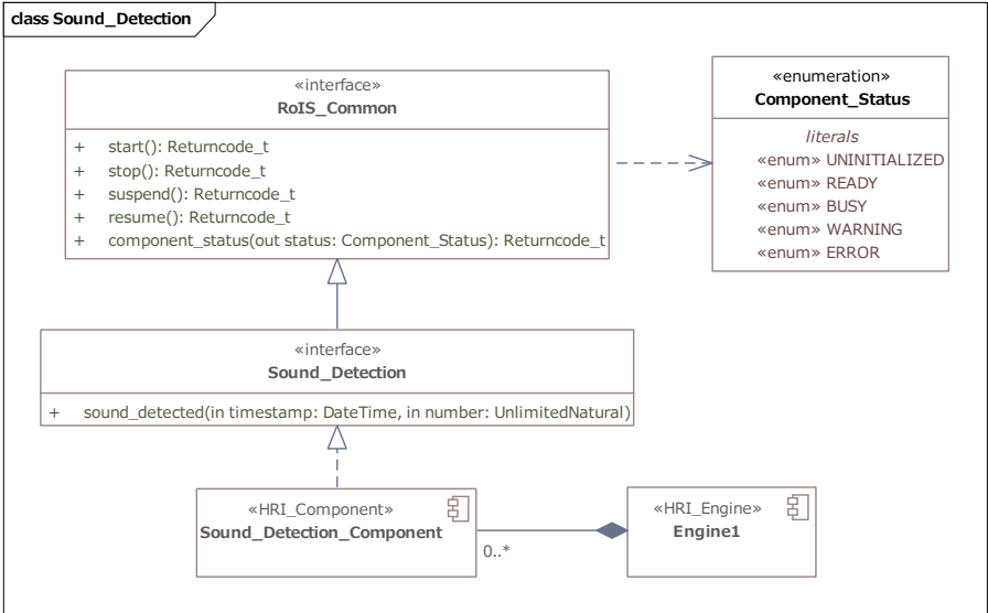
Figure 8.19: Sound Detection
