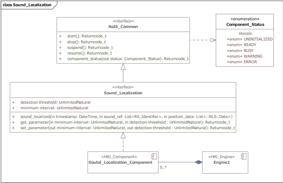
Figure 8.20: Sound Localization
