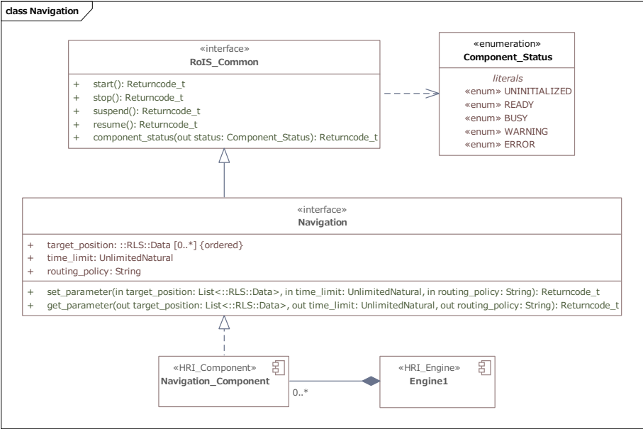
Figure 8.25: Navigation
