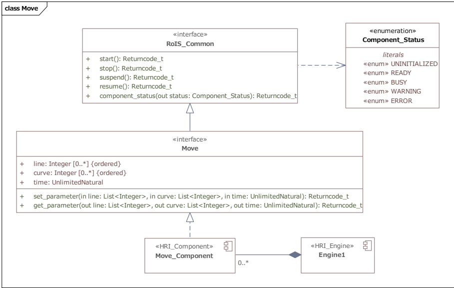
Figure 8.27: Move
