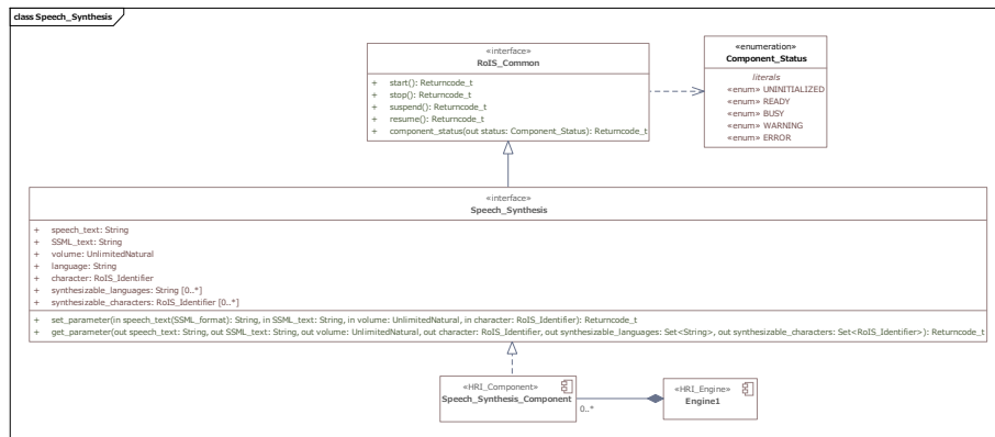
Figure 8.23: Speech Synthesis
