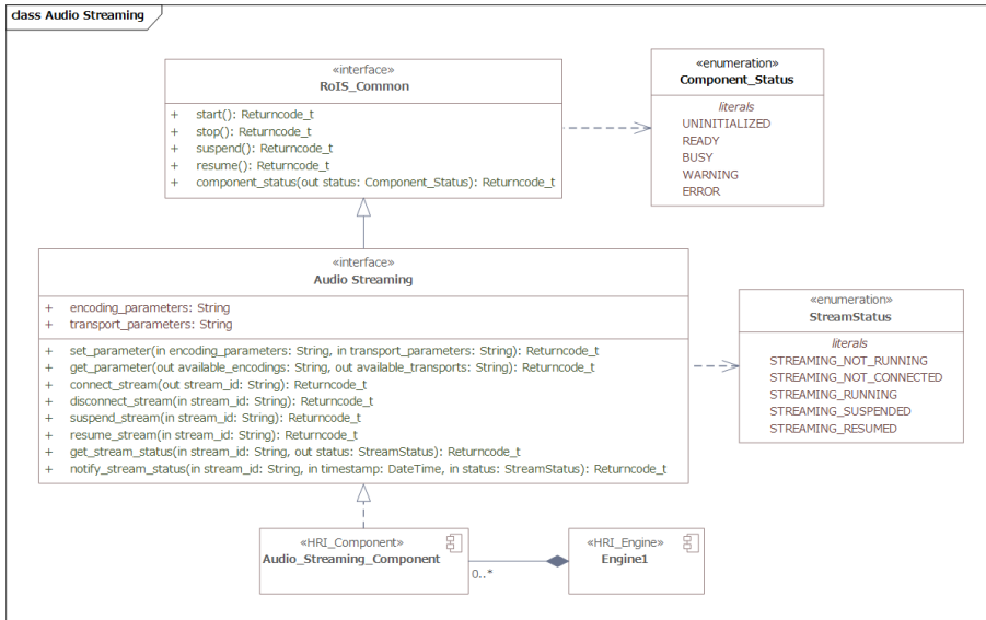
Figure 8.28: Audio Streaming
