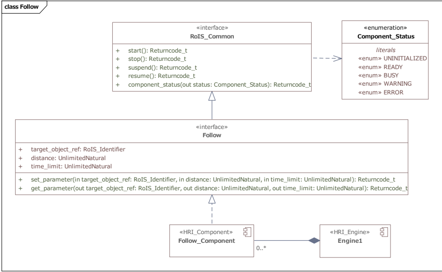
Figure 8.26: Follow
