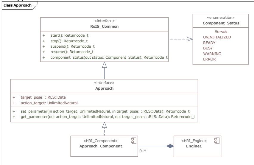
Figure C.3: Approach
