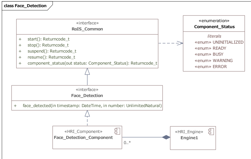
Figure 8.17: Face Detection
