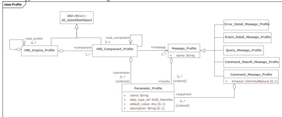
Figure 8.12: RoIS Profile. RoIS profile mainly consists of 4 types of profiles, i.e., “HRI_Engine_Profile,” “HRI_Component_Profile,” “Message_Profile,” and “Parameter_Profile.”
