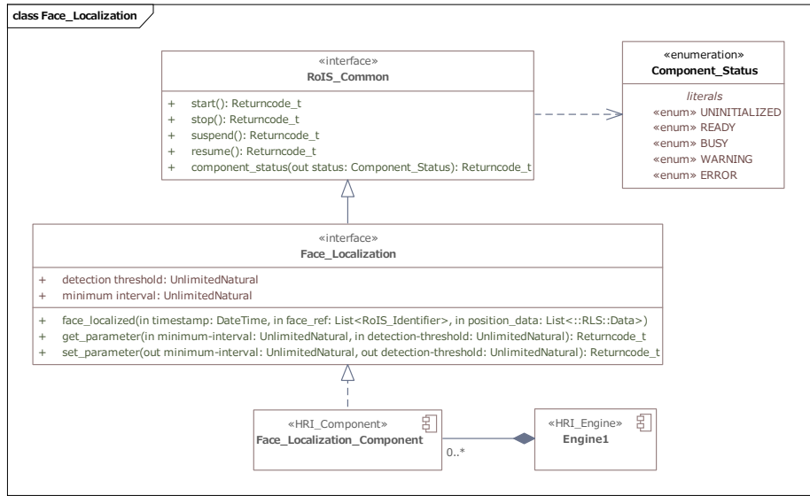
Figure 8.18: Face Localization
