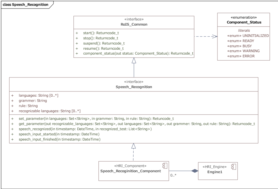
Figure 8.21: Speech Recognition
