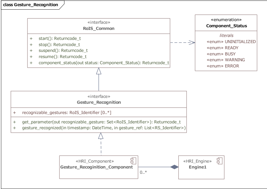
Figure 8.22: Gesture Recognition
