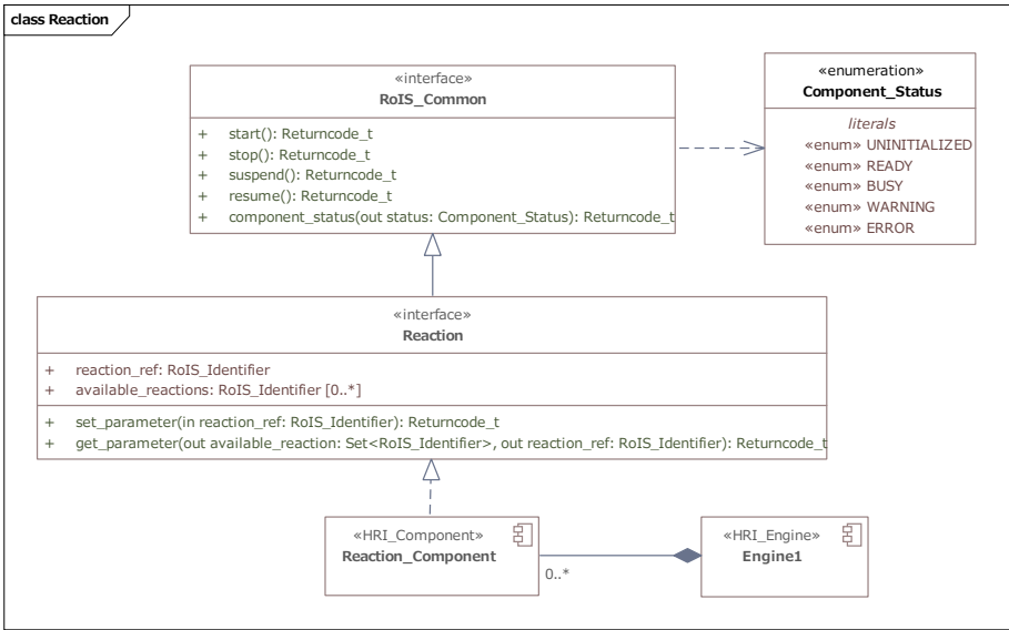
Figure 8.24: Reaction
