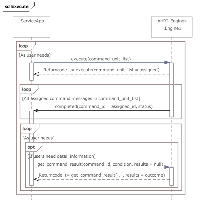
Figure 8.5: Sequence Diagram of “Execute” in Command Interface
