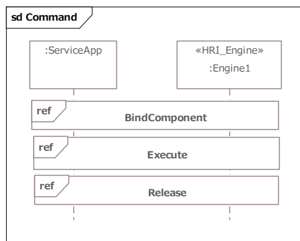
Figure 8.3: Sequence Diagram of Command Interface
