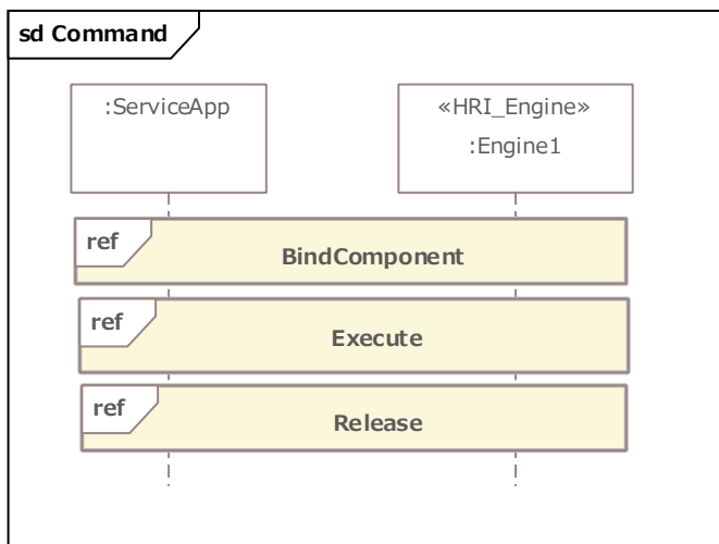
Figure 8-3: Sequence Diagram of Command Interface
