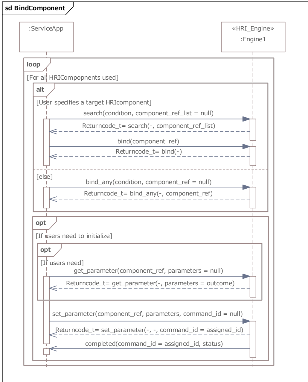
Figure 8-4: Sequence Diagram of “BindComponent” in Command Interface
