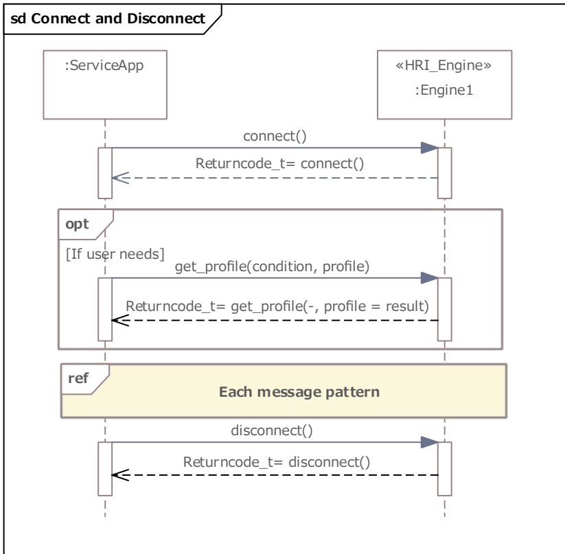
Figure 8-1: Sequence Diagram of System Interface (Connect / Disconnect)
