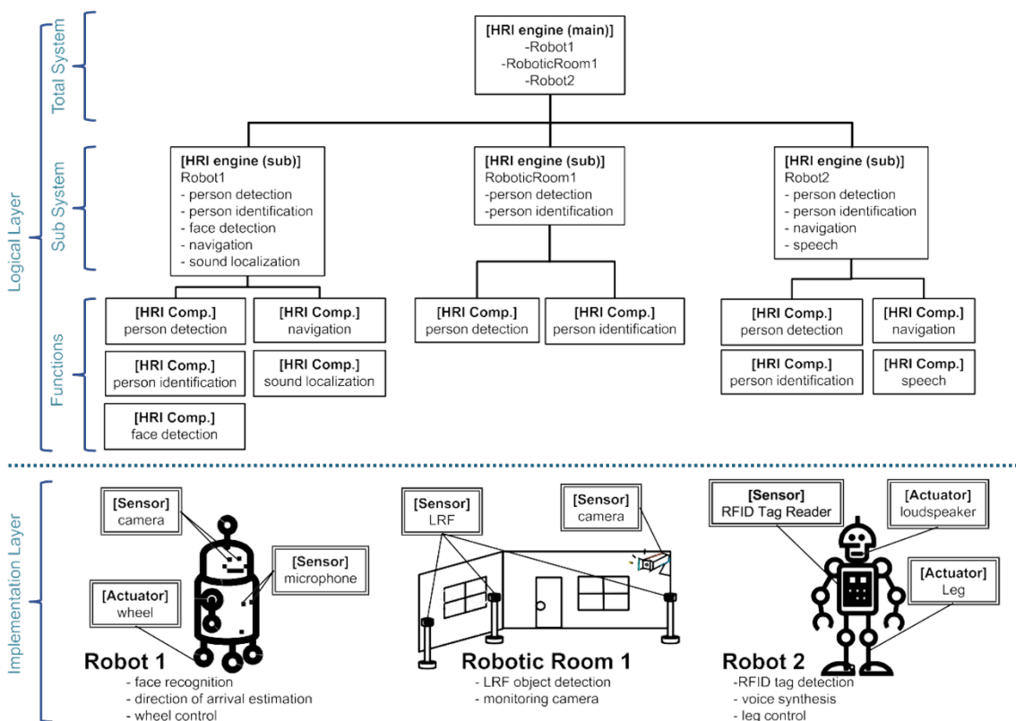
Figure 7-4: Example of HRI Engine and HRI Components
