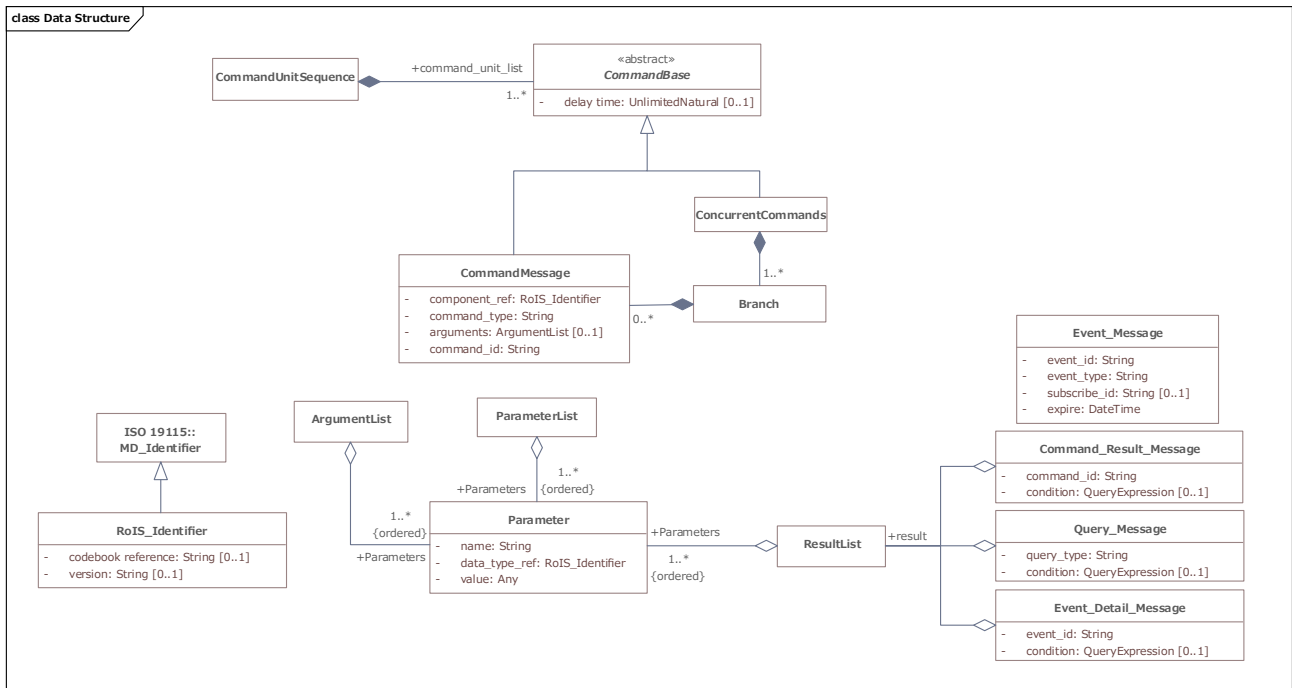
Figure 8-11: Data Structure of Command Message.
