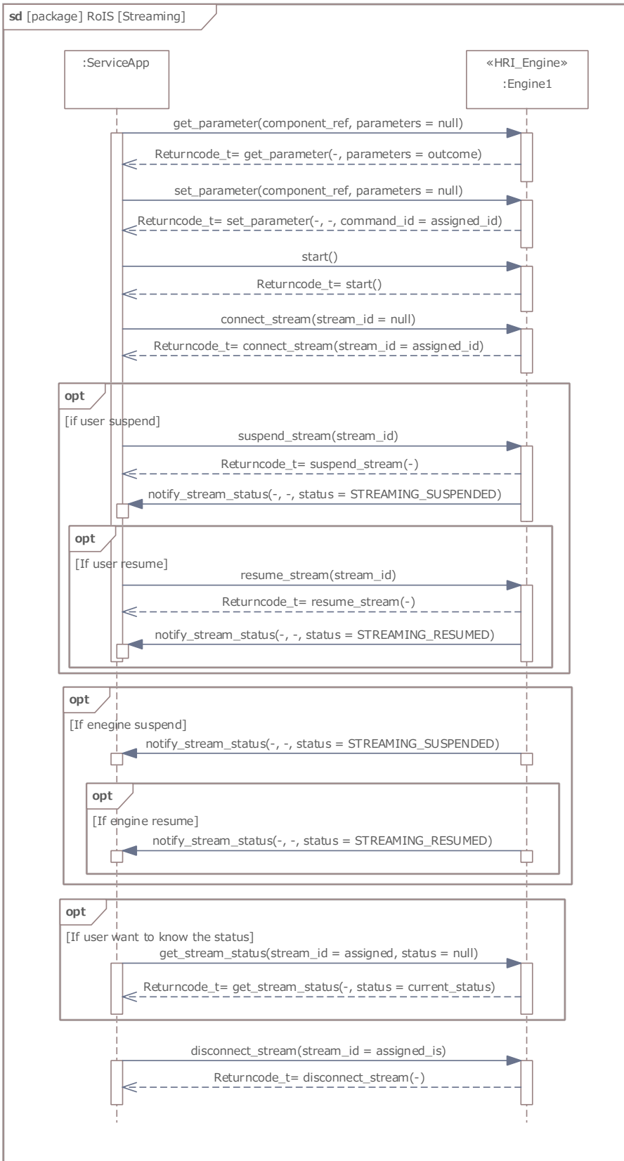
Figure 8-9: Sequence Diagram of Streaming Interface
