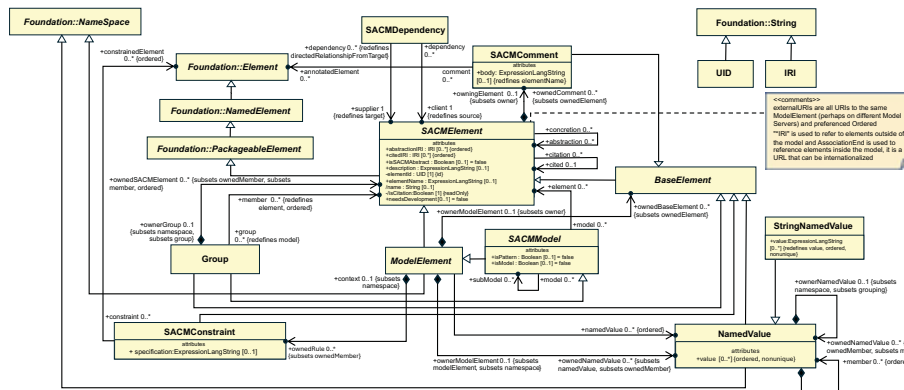
Figure 9.1 Structured Assurance Case Base Classes Diagram
