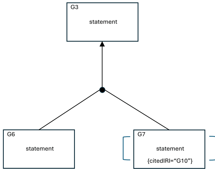
Figure D5. Example of Claim citation
