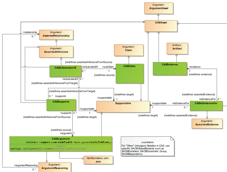
Figure A.4 – CAE Diagram
