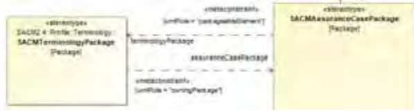
Figure F.2 – UML role in a profile
