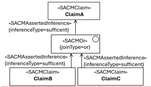
Figure 15.1.2.2 – Join in Deductive Logic Example
