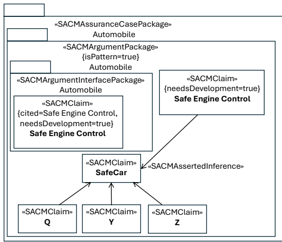
Figure E2 – Automobile Assurance Case Illustration
