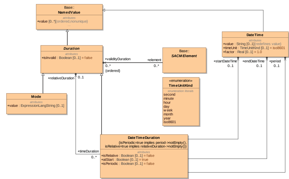
Figure 15.5.1 – Data Time Duration Diagram
