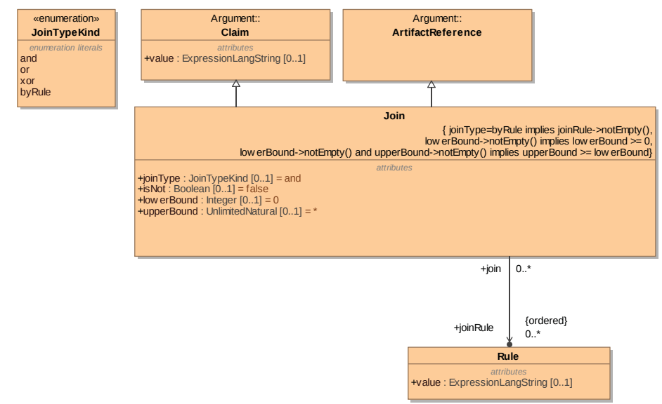
Figure 15.1.1 – SACM Join Diagram
