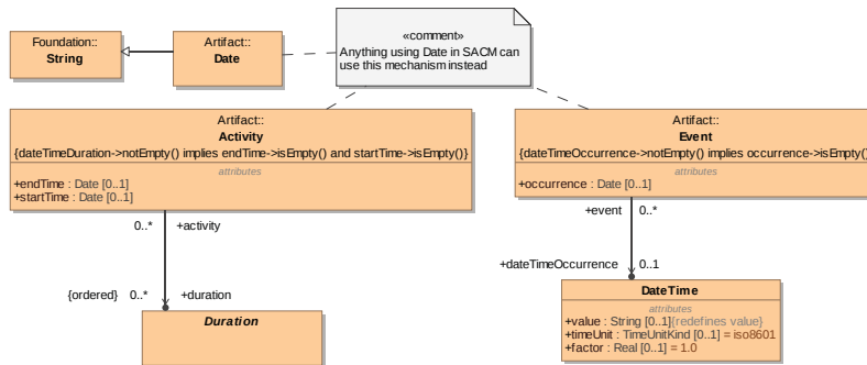
Figure 15.5.2 – Advanced Artifact Diagram
