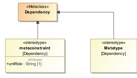
Figure F.1 – SACM metaconstraint
