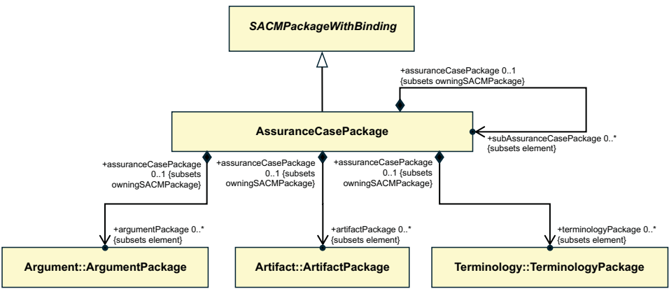
Figure 11.1 Structured Assurance Case Packages Class Diagram
