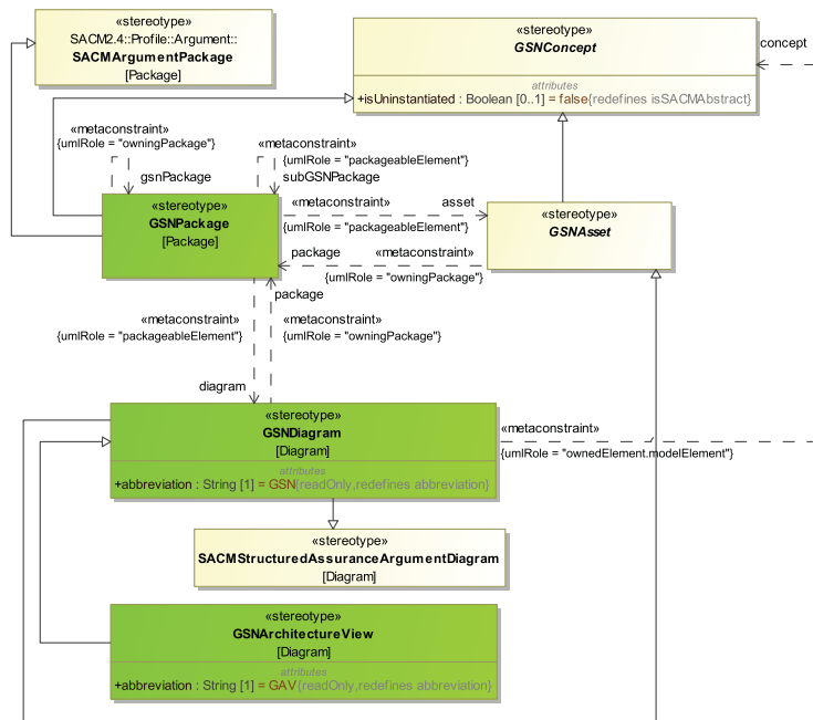
Figure A.3.2 – GSN Package Profile Diagram
