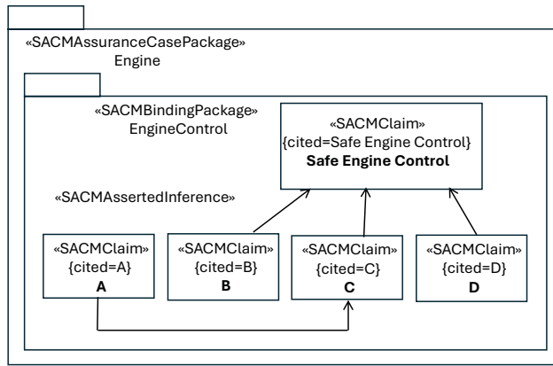
Figure E4 – Automobile Assurance Case Illustration
