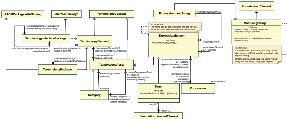
Figure 12.1 – Terminology Class Diagram
