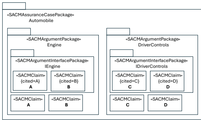
Figure E3 – Assurance Case Bindings Illustration
