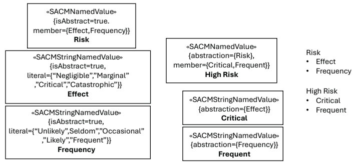
Figure 15.7.2 NamedValue Type Example
