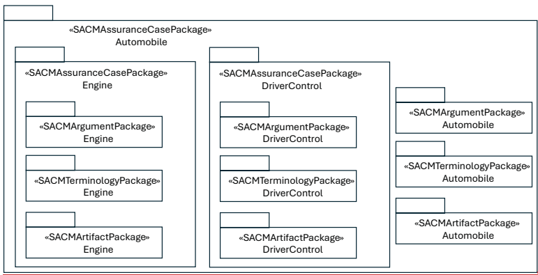
Figure E1 – Automobile Assurance Case Illustration
