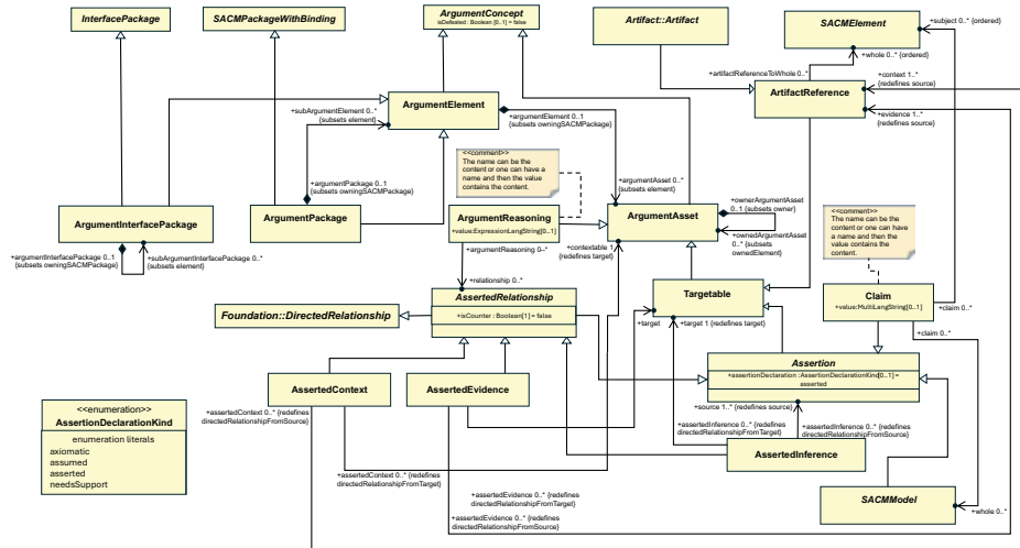
Figure 13.1 Argumentation Package Diagram
