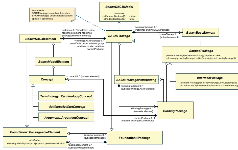
Figure 10.1 – SACM Package Class Diagram
