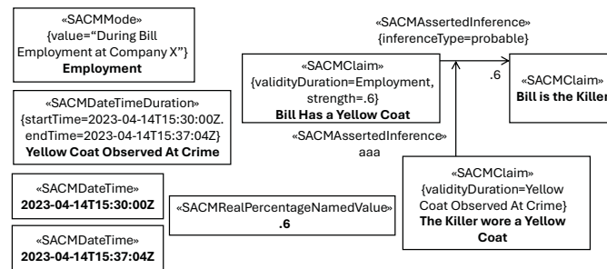
Figure 15.5.8 – DateTimeDuration Examples
