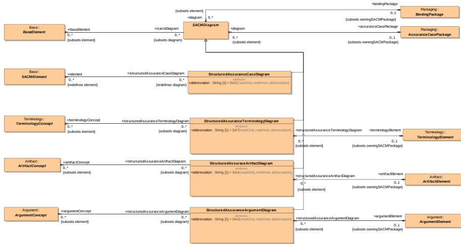
Figure 15.3.4 – SACMDiagramTypes
