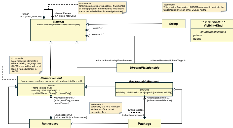
Figure 8.1 – Foundation Class
