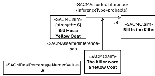
Figure 15.2.6.1 – Abduction Example
