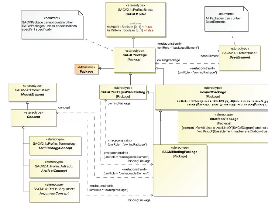
Figure F.9 – SACMPackage section of the SACM profile.
