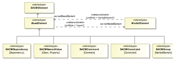
Figure F.6 – BaseElement section of the SACM profile.
