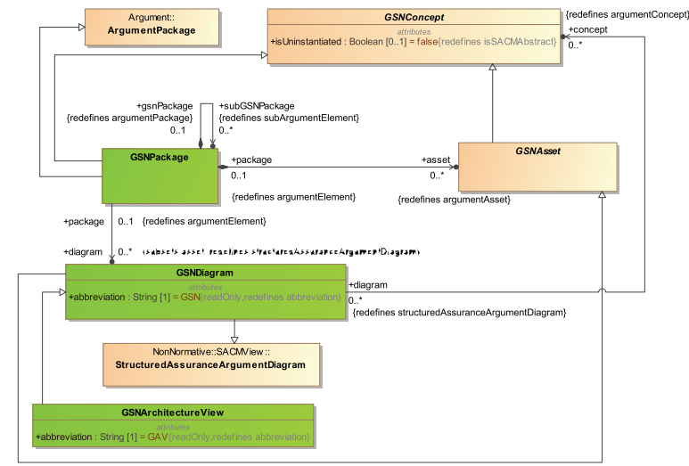
Figure A.2 – GSN Package Diagram
