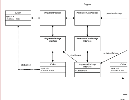
Figure E6 – Specific Relationships between DriverControls, EngineControl, and Engine Assurance Cases Illustration¶
