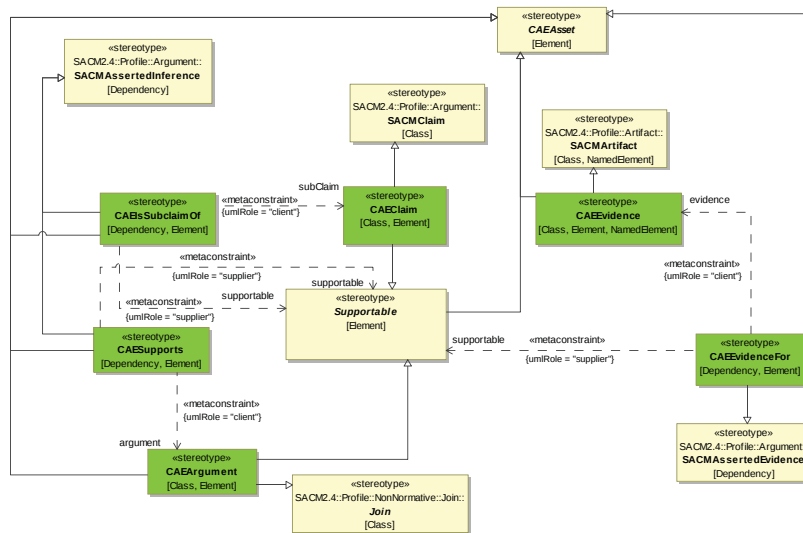
Figure A.6.1 – CAE Profile Diagram
