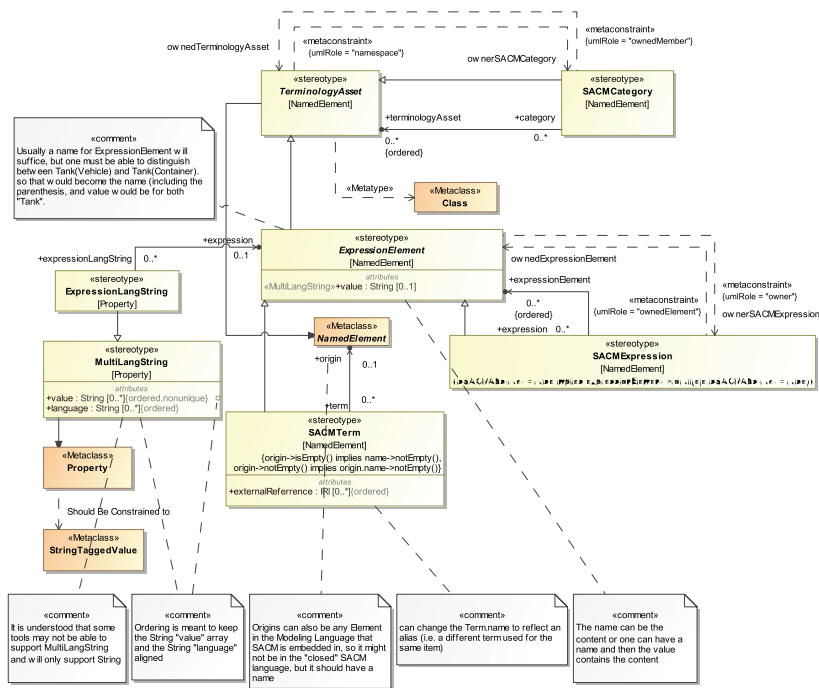
Figure F.11 – Terminology section of the SACM profile.
