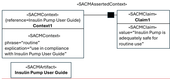
Figure 15.7.2 Argument Context Example
