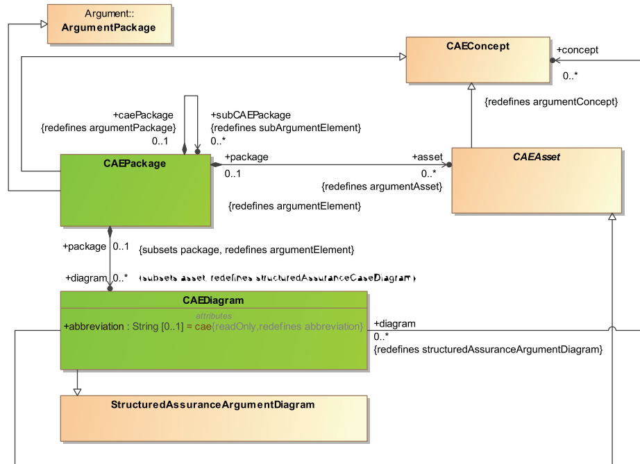
Figure A.5 – CAE Package Diagram
