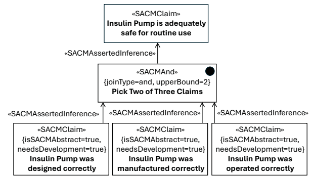
Figure 15.1.2.1 – Join in a Template Example
