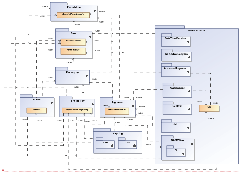
Figure 7.2 - Overall SACM Class Diagram
