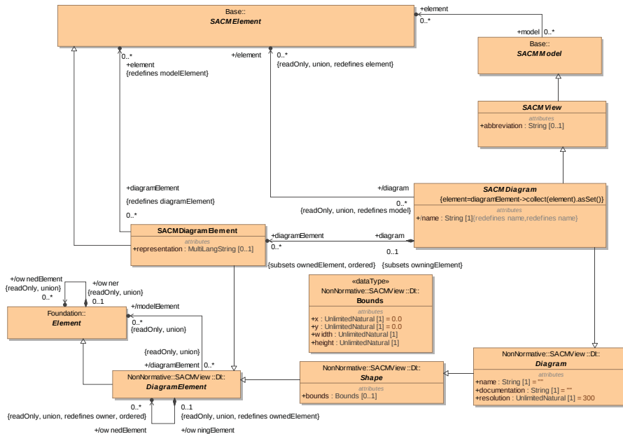
Figure 15.3.2 – SACMDiagram
