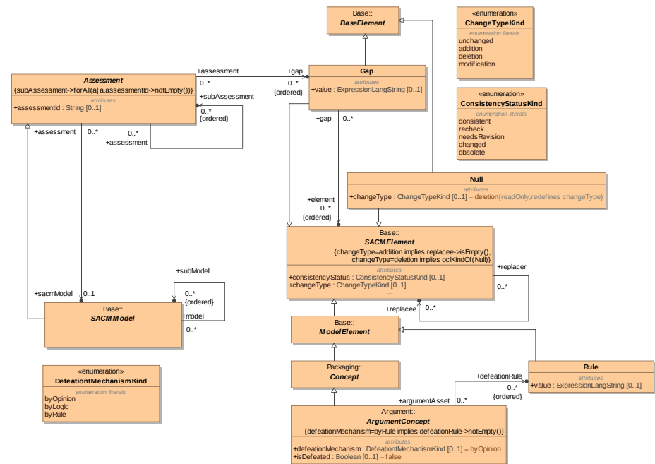
Figure 15.4.1 – SACM Assessments
