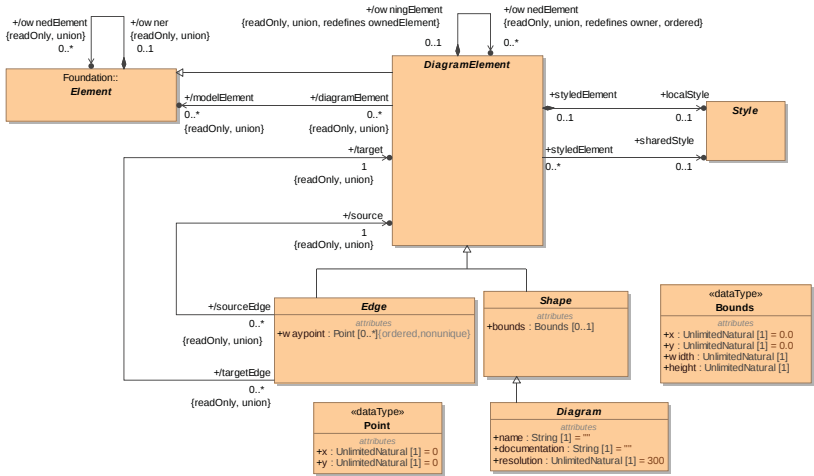
Figure 15.3.1 – OMG's DI Standard Diagram
