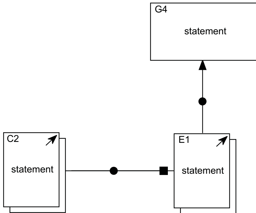
Figure D11 – Example of AssertedContext
