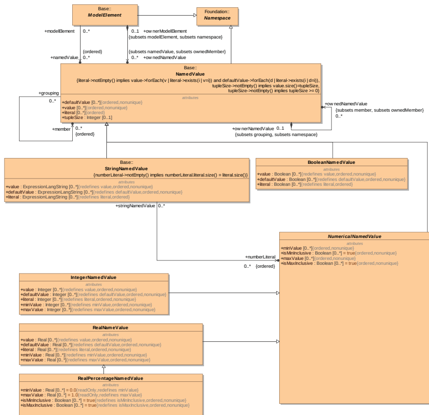
Figure 15.6.1 – NamedValue Type Diagram
