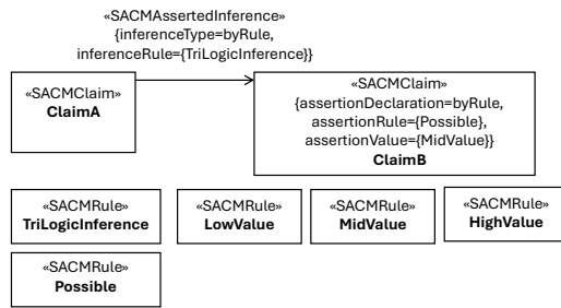
Figure 15.2.6.2 – byRule Example
