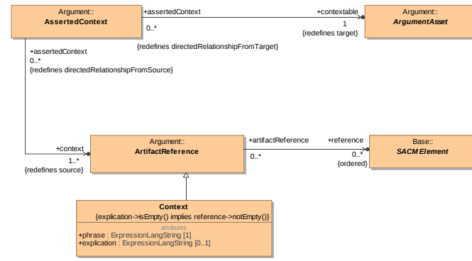
Figure 15.7.1 – Argument Context Diagram
