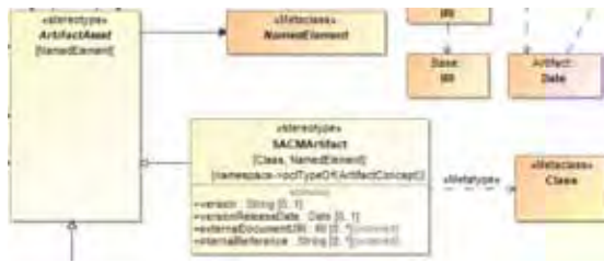
Figure F.4 – Metatype to Class
